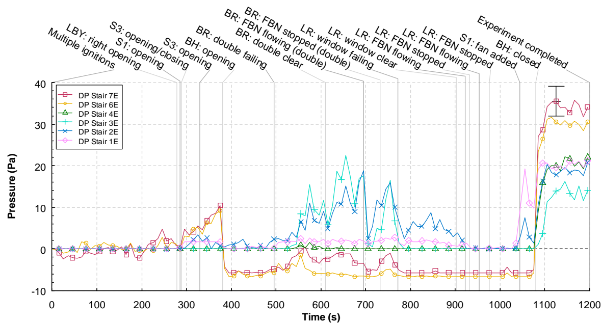
Figure 3.13-19. 3A stairwell pressures vs. time
