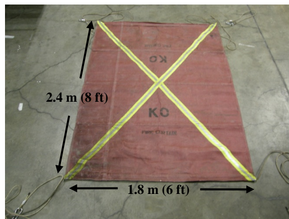
Figure 1.8-2. Wind Control Device Open
