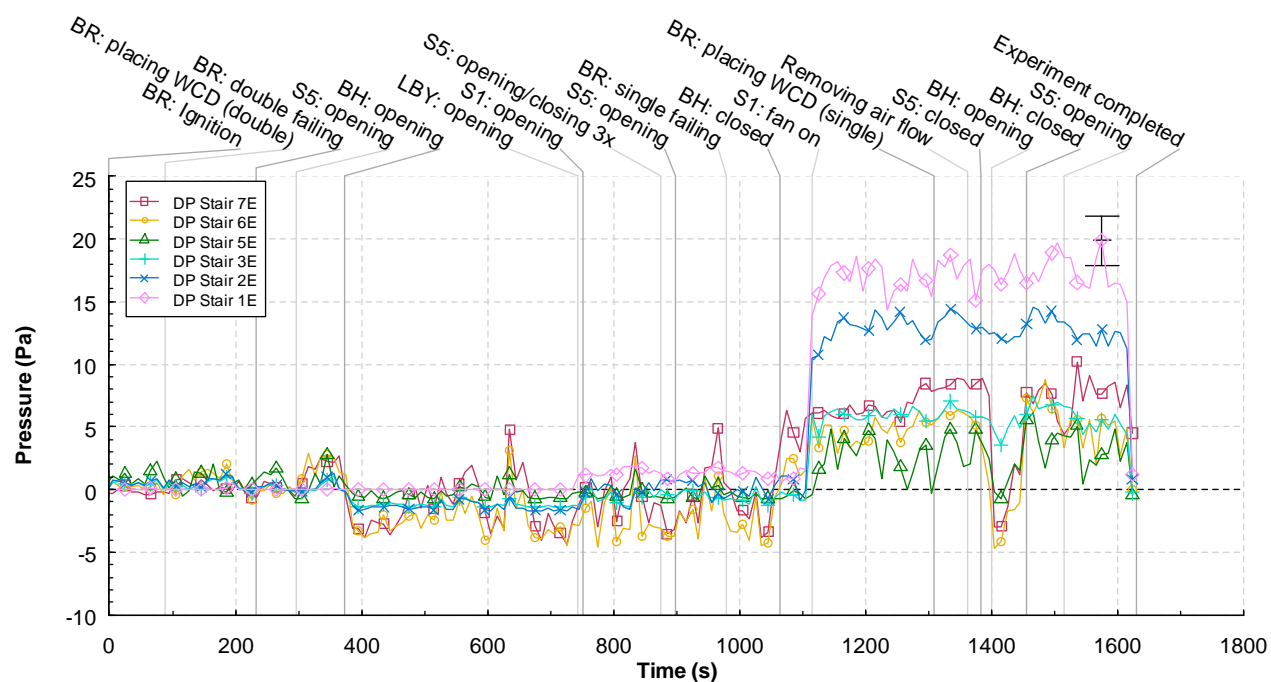
Figure 9.4-61. Differential pressure versus time for the stairwell bi-directional probes, Experiment 5E
