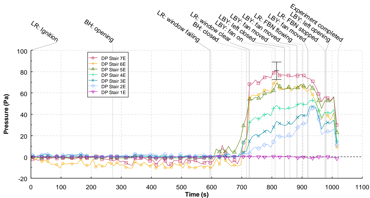
Figure 9.4-72. Differential pressure versus time for the stairwell bi-directional probes, Experiment 5E2
