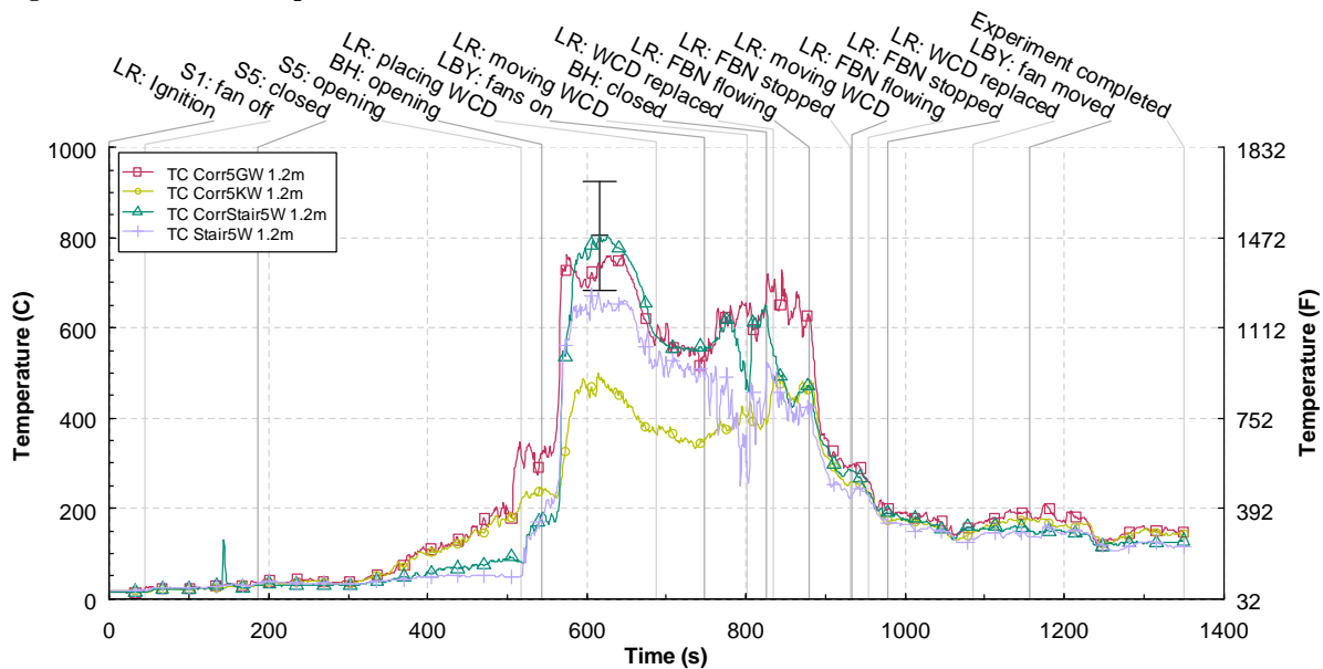
Figure 3.11-14. 5G2 Temperature vs. time at 1.2 m above the floor
