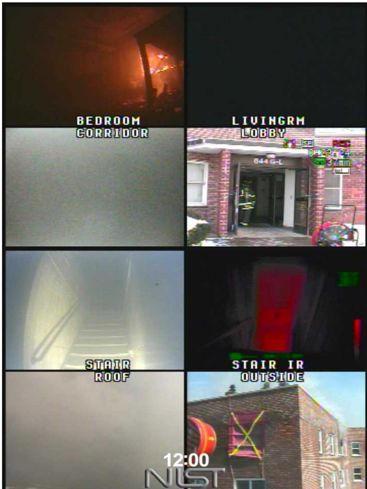
Figure 3.5-10. Experiment 7K, 720s after ignition.
