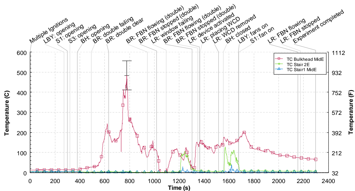
Figure 3.12-22. 3E stairwell temperature vs. time
