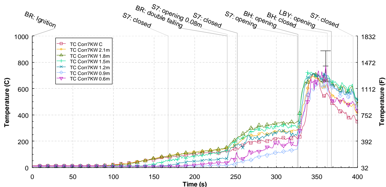
Figure 4-1. Temperature vs time from the vertical thermocouple array at the corridor position outside of apartment 7K.
