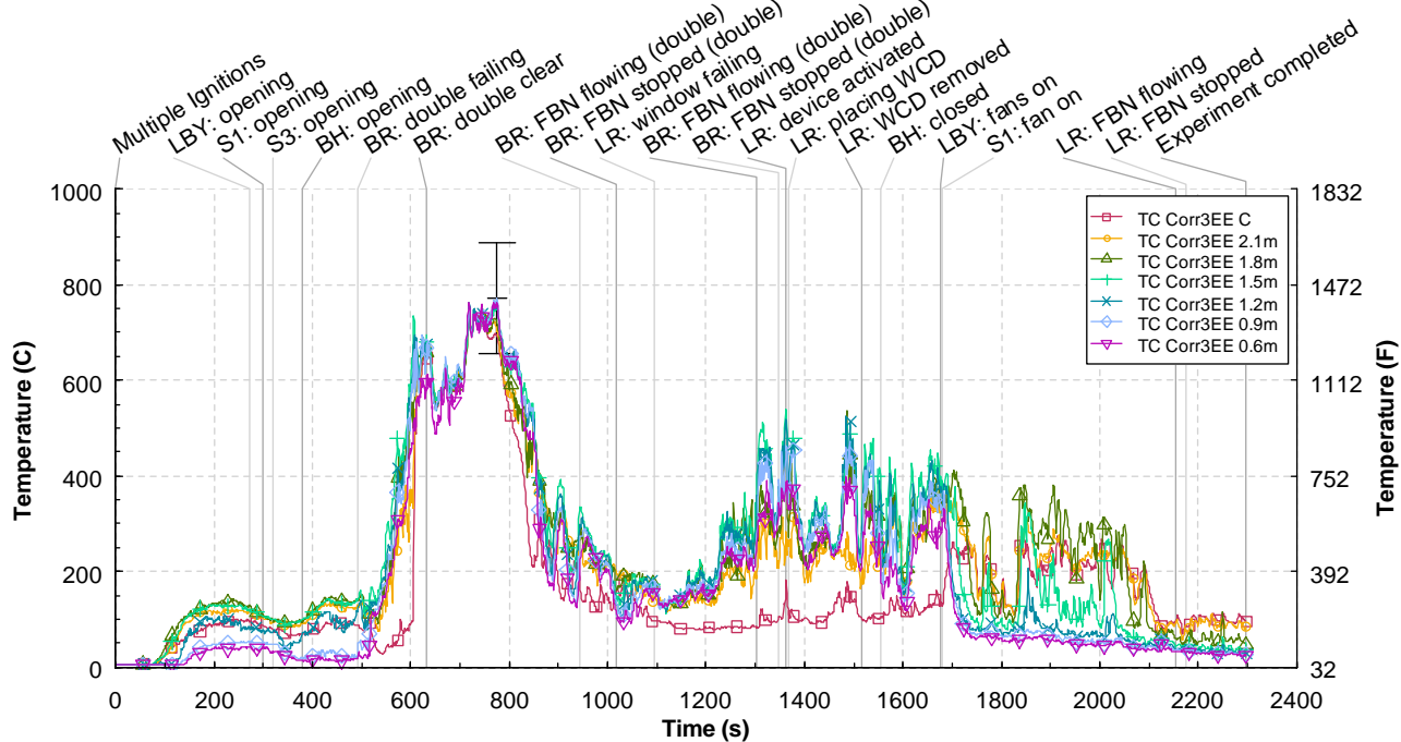
Figure 9.4-116. Temperature versus time for the 3E hall thermocouple tree, Experiment 3E
