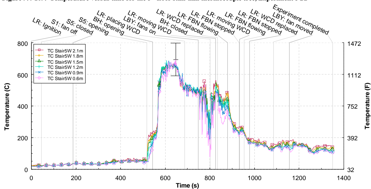
Figure 9.4-110. Temperature versus time for the 5 th floor stairwell thermocouple tree, Experiment 5G2
