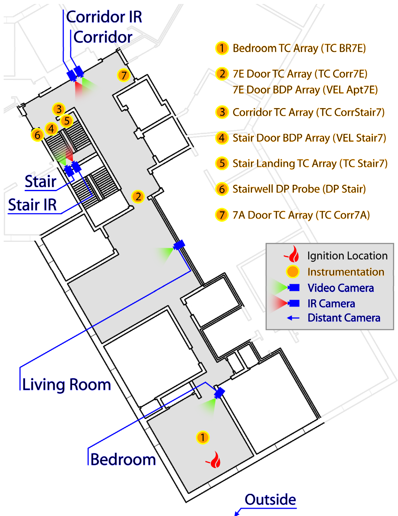
Figure 3.3-2. Instrumentation and camera locations with labels.
