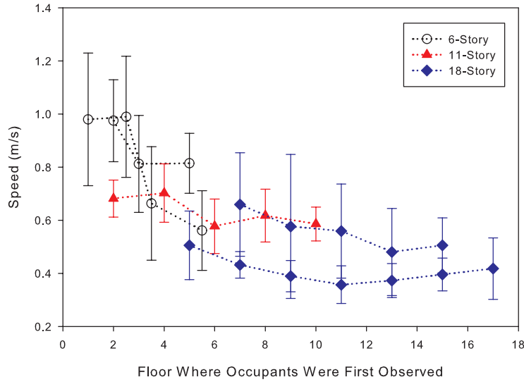
Fig. 1. Occupant movement speeds (with standard deviation) down stairwells in three fire drill evacuations.
