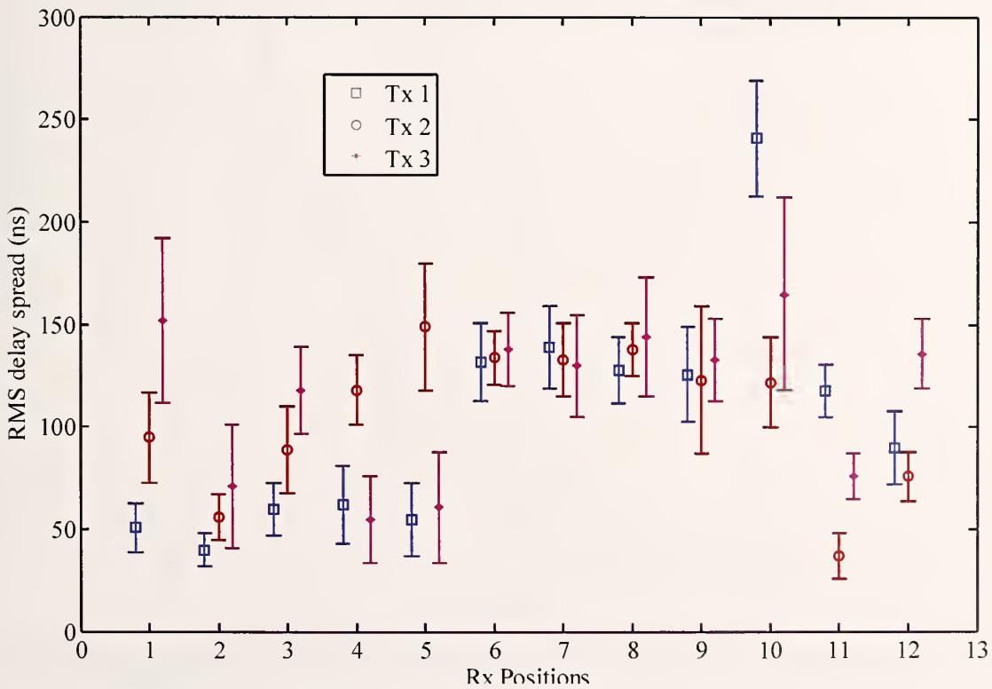
Figure 16. 4900 MHz band, mean RMS delay spread \pm \sigma for each receive antenna location for second transmit location.
