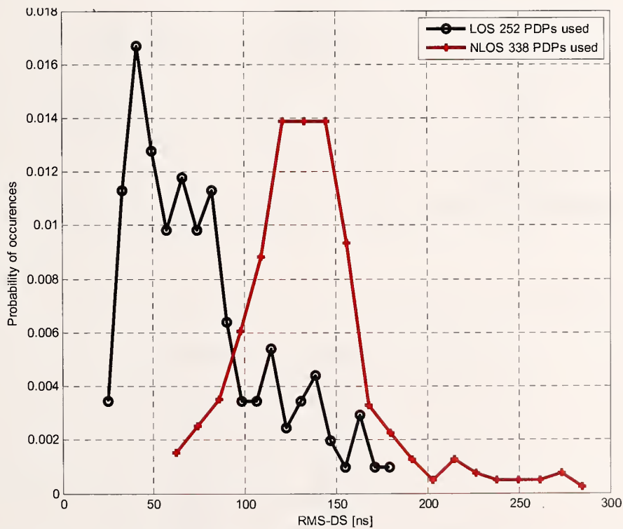
Figure 19. Histograms of RMS delay spread from power delay profiles in both LOS and NLOS locations, 4900 MHz band.
