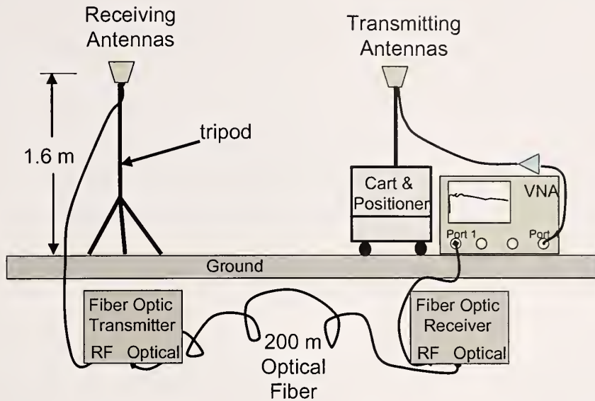
Figure 1. Wideband measurement system based on a vector network analyzer. Frequency-domain measurements, synchronized by the optical fiber link, are transformed to the time domain in post-processing. This enables determination of excess path loss, time-delay spread, and other figures of merit important in characterizing broadband modulated-signal transmissions.
