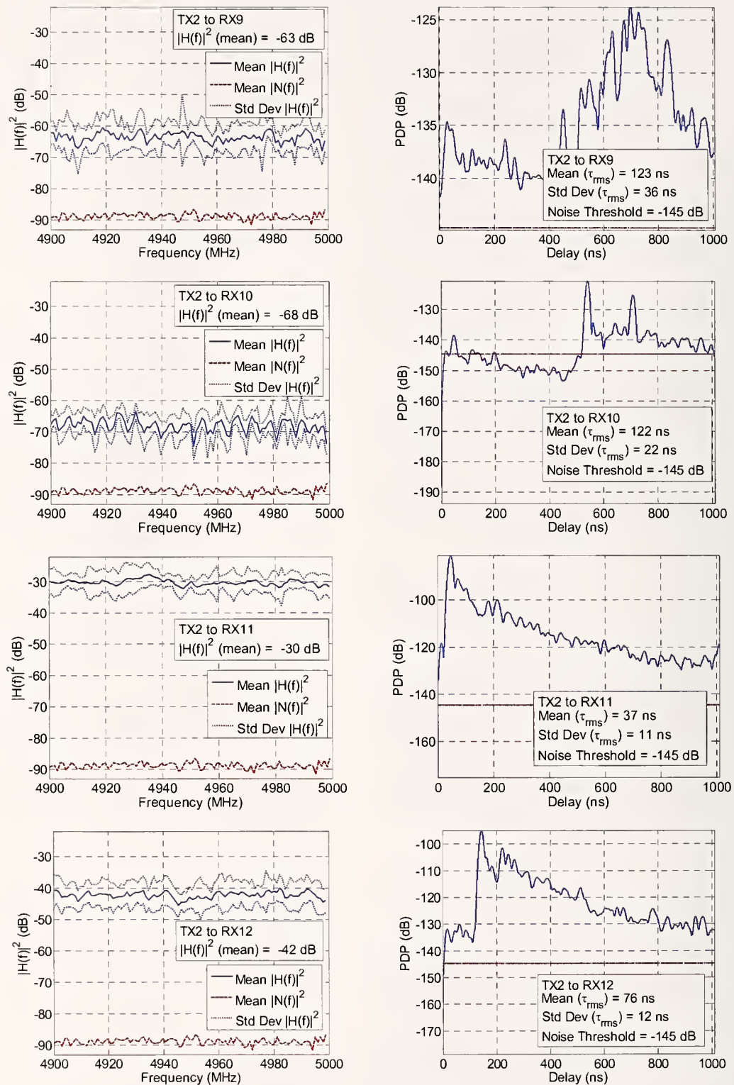
Figure 34. Magnitude squared of the channel performance and PDP for Tx2 to Rx9 through Rx12 pairings in the 4900 MHz band.
