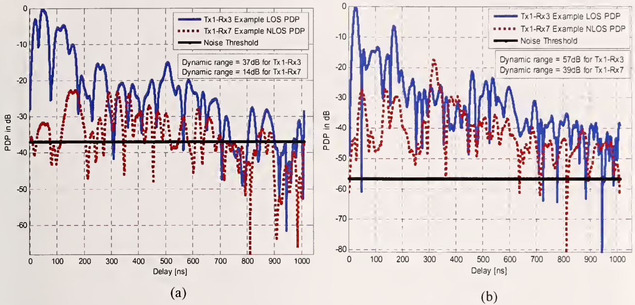
Figure 4. Example PDPs for (a) LOS (Tx1-Rx3) and NLOS (Tx1-Rx7) locations, 700 MHz band, and (b) LOS (Tx1-Rx3) and NLOS (Tx1-Rx7) locations, 4900 MHz band.
