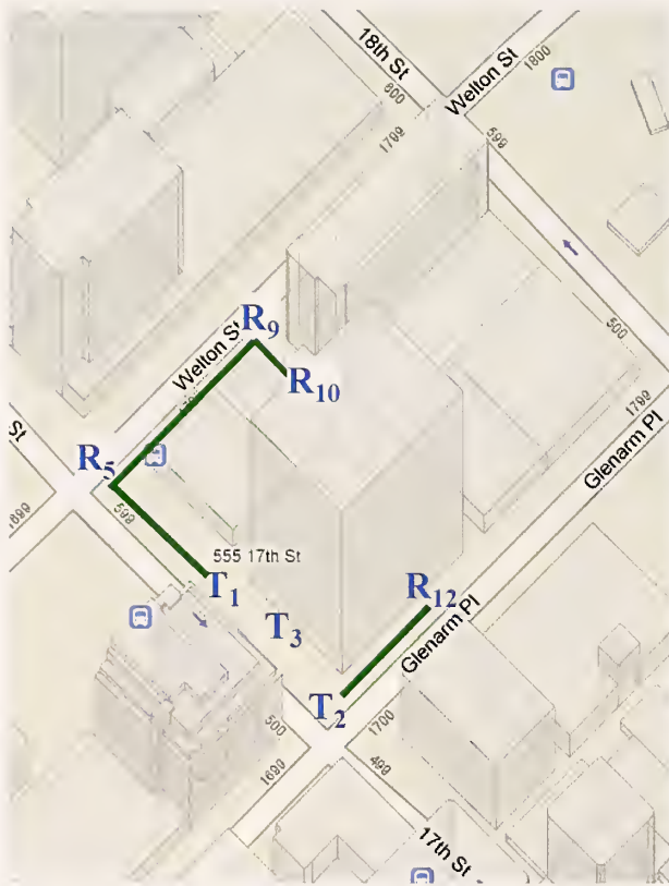
Figure 6. Google map view of test area in downtown Denver. (© 2009 Google, Map Data © 2009 Tele Atlas.) Transmit locations denoted T, receiver locations denoted R. Right: photo of Rx antennas at location R5.
