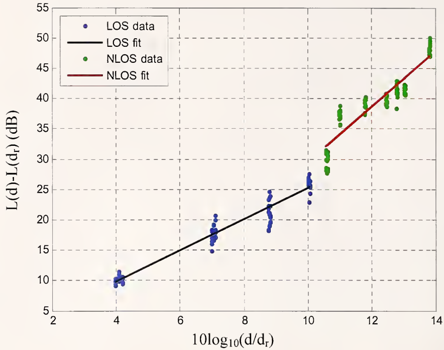
Figure 14. Excess propagation path loss (dB) vs. 10\log_{10}(\text{distance}/d_r) , 700 MHz band.
