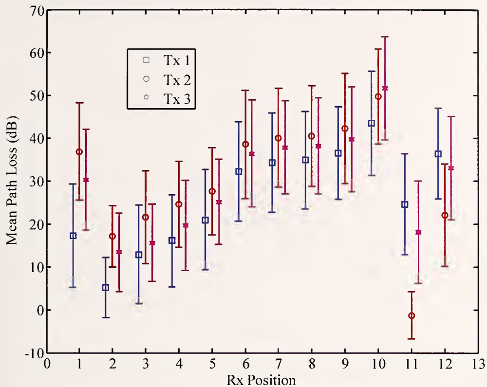
Figure 12. The mean path loss of the eighteen measurements collected at each of the twelve locations, with \pm 2\sigma error bars, for each to the three transmitter locations. 725 MHz to 800 MHz.
