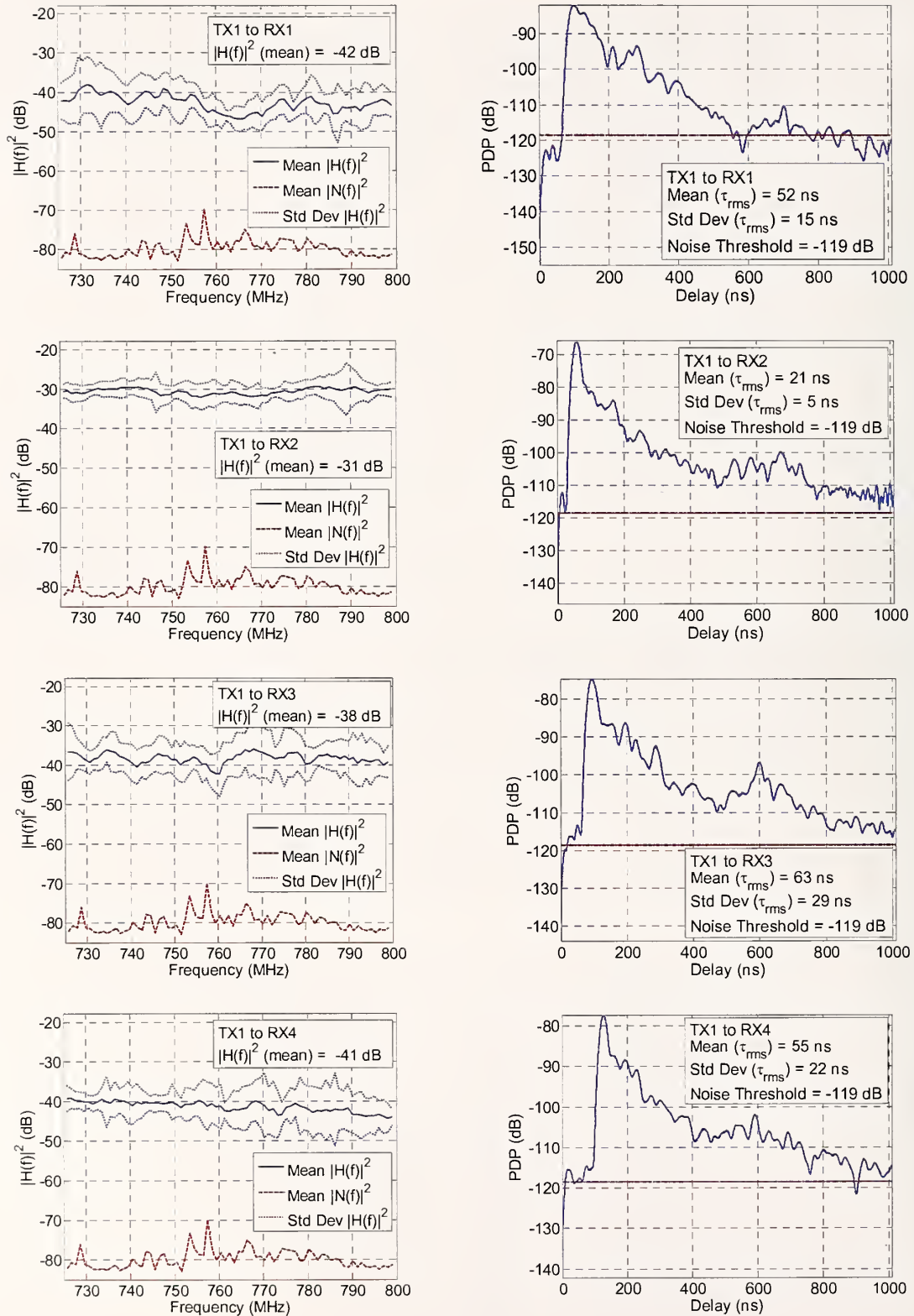
Figure 20. Magnitude squared of the channel performance and PDP for Tx1 to Rx1 through Rx4 pairings in the 700 MHz band.
