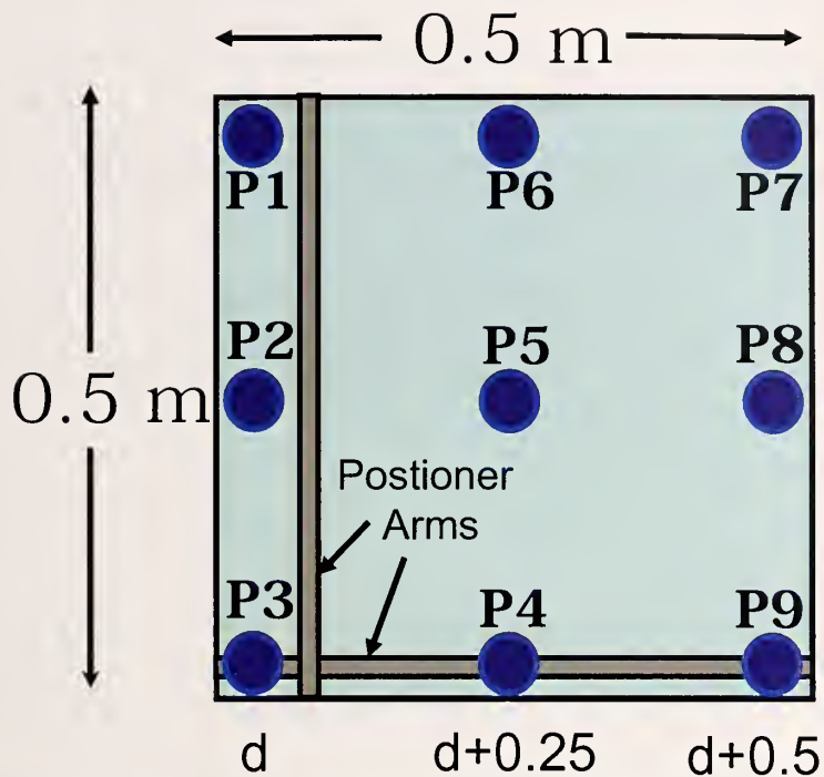
Figure 10. Plan view diagram of antenna positioner, showing nine positions.
