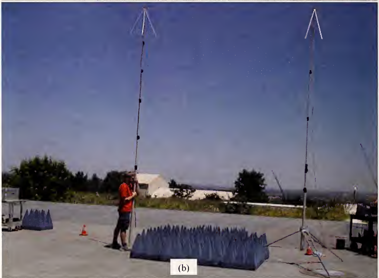
Figure 3. Reference tests at the NIST-Boulder open area test site (OATS) with (a) 700 MHz and 4900 MHz antennas at a height of 1.6 m, and (b) 700 MHz antenna at a height of 5 m.
