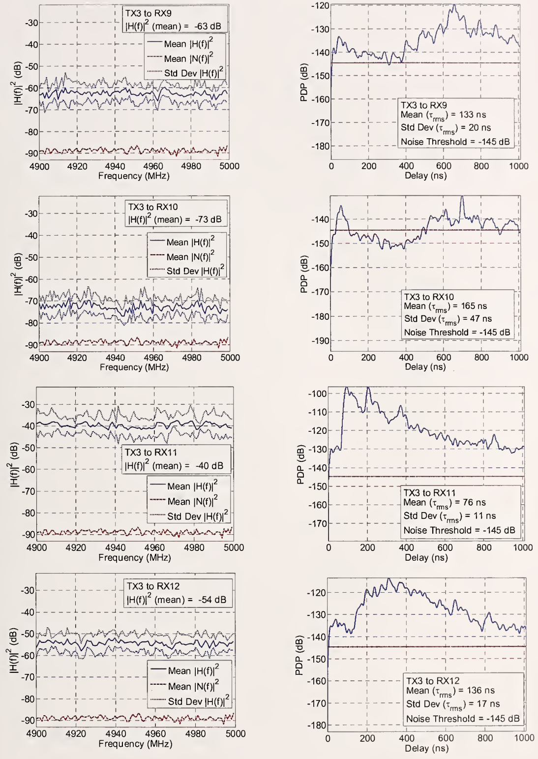
Figure 37. Magnitude squared of the channel performance and PDP for Tx3 to Rx9 through Rx12 pairings in the 4900 MHz band.
