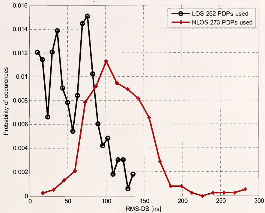
Figure 18. Histograms of RMS delay spread from power delay profiles in both LOS and NLOS locations, 700 MHz band.
