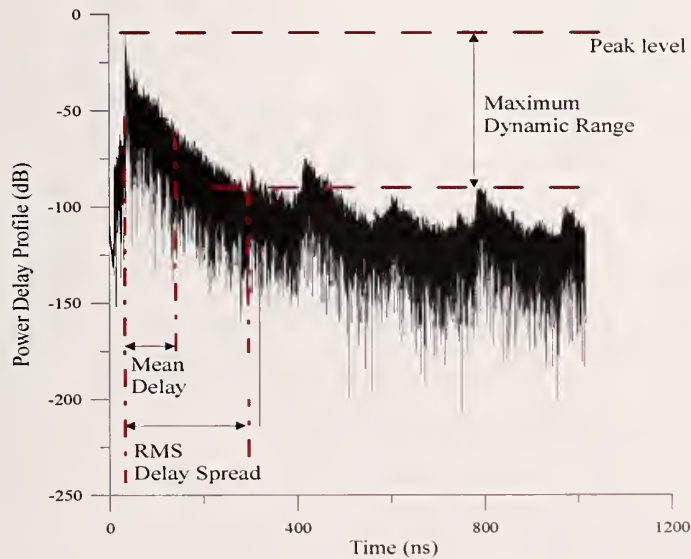
Figure 5. Power-delay profile for a building propagation measurement. Important parameters for a measured signal are the peak level, the maximum dynamic range, the mean delay, and the RMS delay spread.
