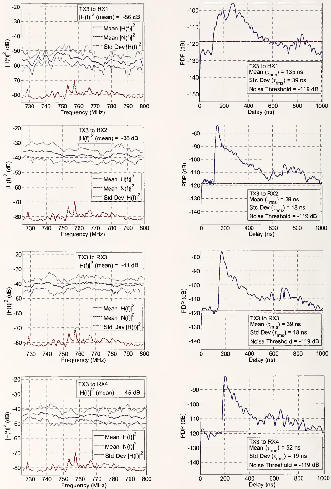
Figure 26. Magnitude squared of the channel performance and PDP for Tx3 to Rx1 through Rx4 pairings in the 700 MHz band.
