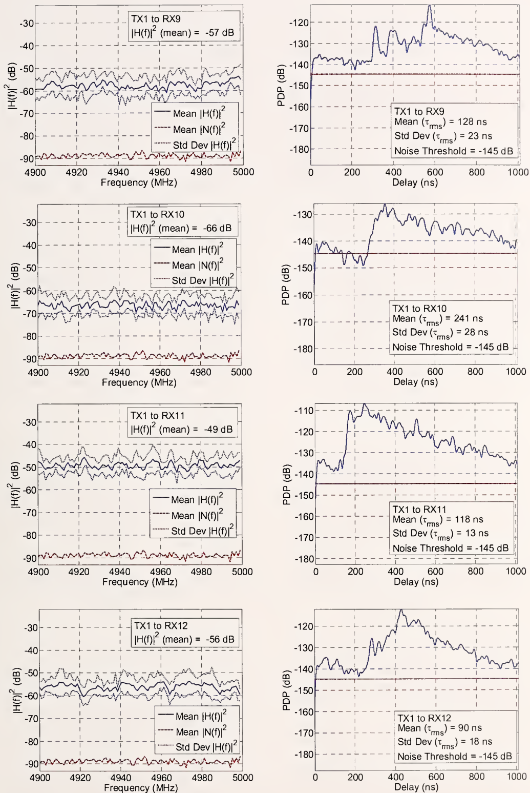
Figure 31. Magnitude squared of the channel performance and PDP for Tx1 to Rx9 through Rx12 pairings in the 4900 MHz band.
