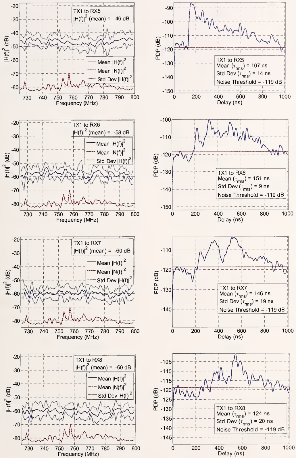
Figure 21. Magnitude squared of the channel performance and PDP for Tx1 to Rx5 through Rx8 pairings in the 700 MHz band.
