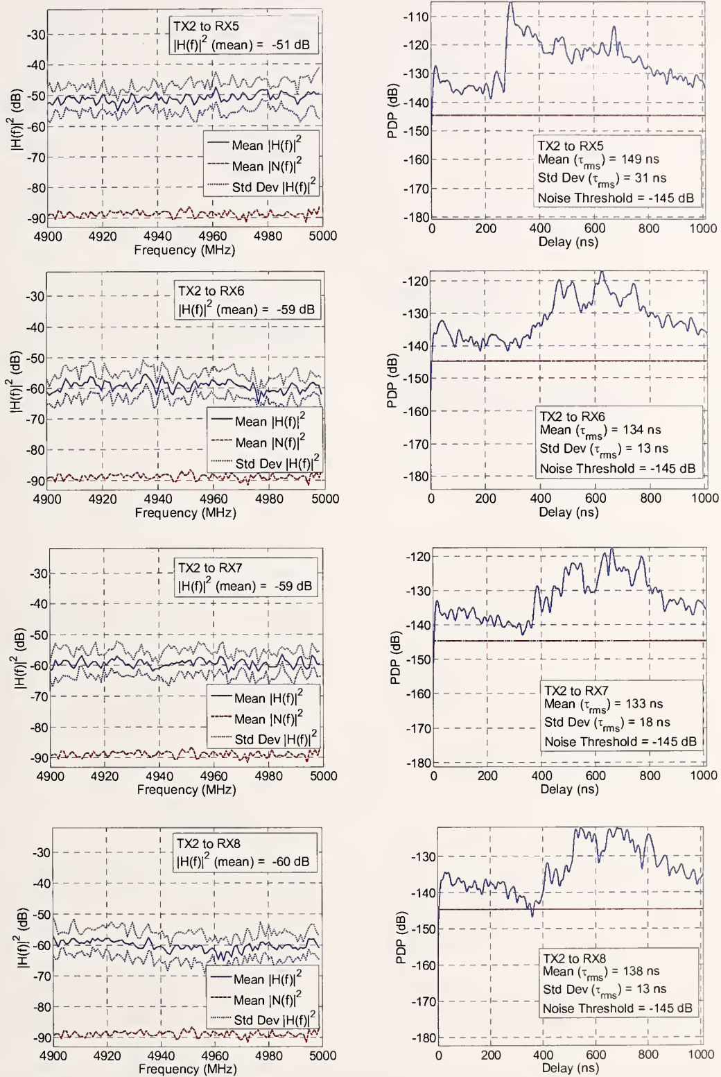
Figure 33. Magnitude squared of the channel performance and PDP for Tx2 to Rx5 through Rx8 pairings in the 4900 MHz band.
