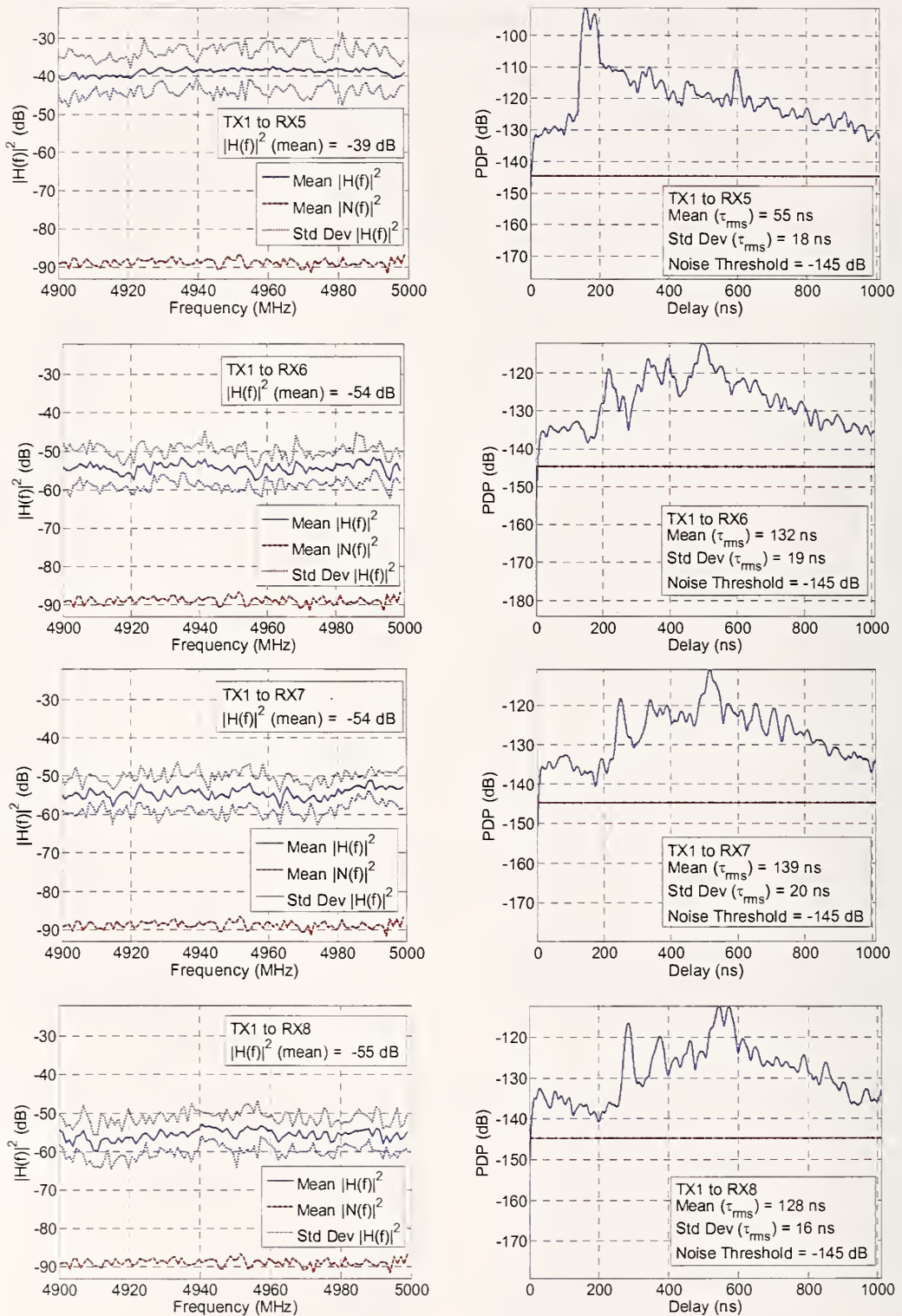
Figure 30. Magnitude squared of the channel performance and PDP for Tx1 to Rx5 through Rx8 pairings in the 4900 MHz band.
