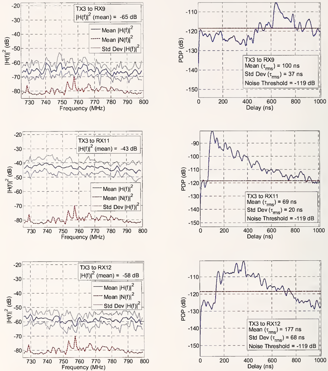
Figure 28. Magnitude squared of the channel performance and PDP for Tx3 to Rx9, Rx11, and Rx12 pairings in the 700 MHz band.
