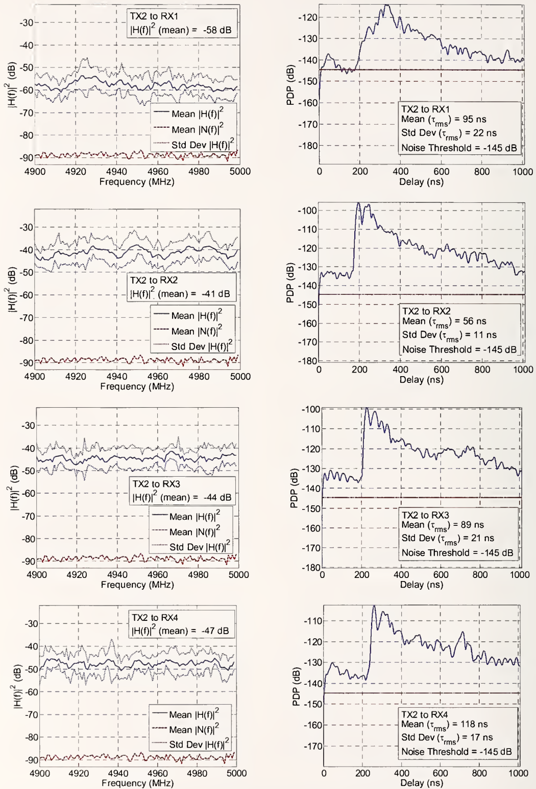
Figure 32. Magnitude squared of the channel performance and PDP for Tx2 to Rx1 through Rx4 pairings in the 4900 MHz band.
