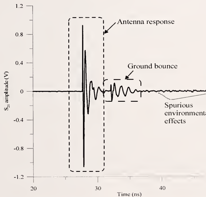
Figure 2. Reference measurement at 3 m for a dual-ridge guide horn antenna, transformed to the time domain. The waveform shows the antenna response, the ground-bounce response and the spurious environmental effects.
