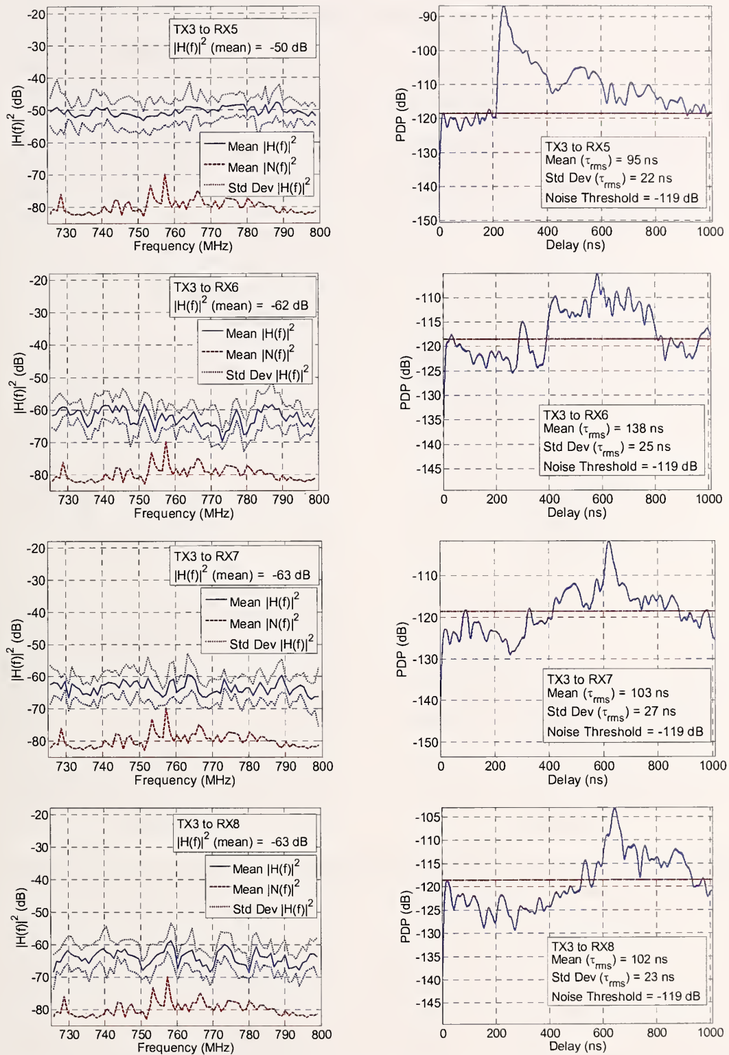
Figure 27. Magnitude squared of the channel performance and PDP for Tx3 to Rx5 through Rx8 pairings in the 700 MHz band.
