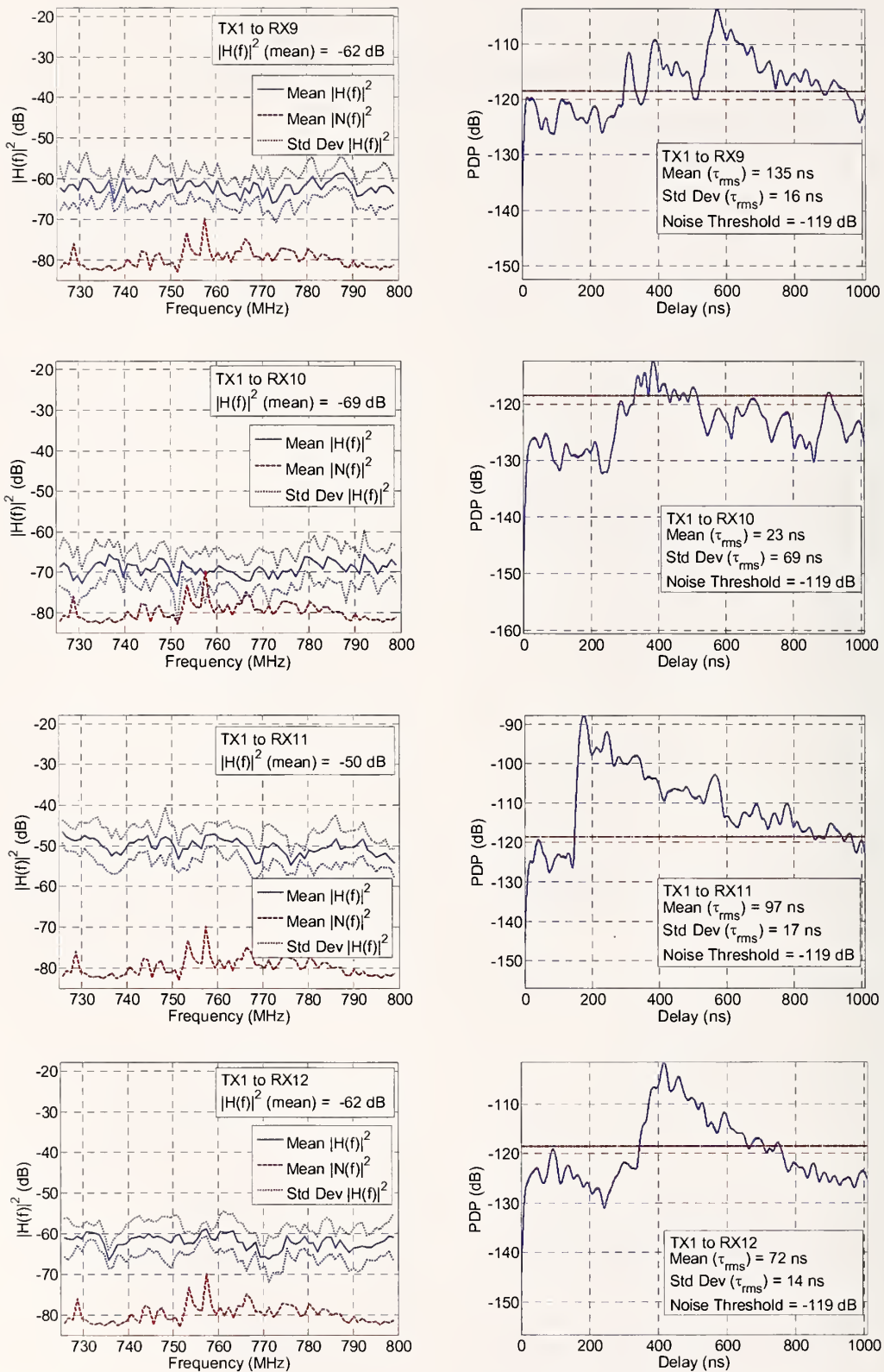
Figure 22. Magnitude squared of the channel performance and PDP for Tx1 to Rx9 through Rx12 pairings in the 700 MHz band.
