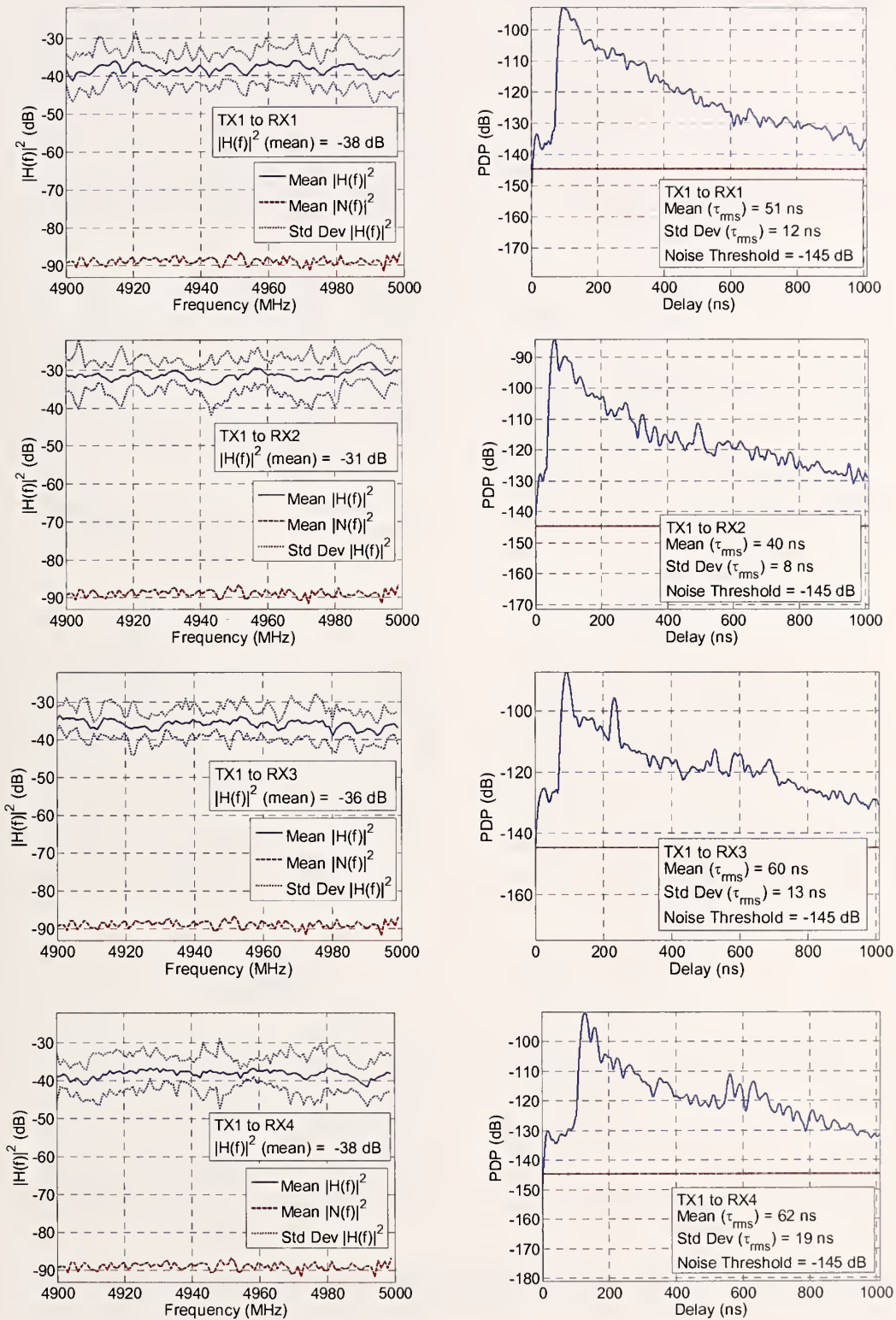
Figure 29. Magnitude squared of the channel performance and PDP for Tx1 to Rx1 through Rx4 pairings in the 4900 MHz band.
