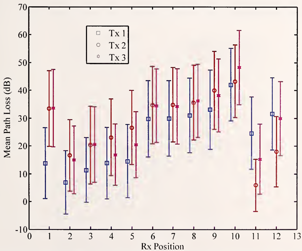
Figure 13. The mean path loss of the eighteen measurements collected at each of the twelve locations, with \pm 2\sigma error bars, for each to the three transmitter locations. 4900 MHz to 5000 MHz.
