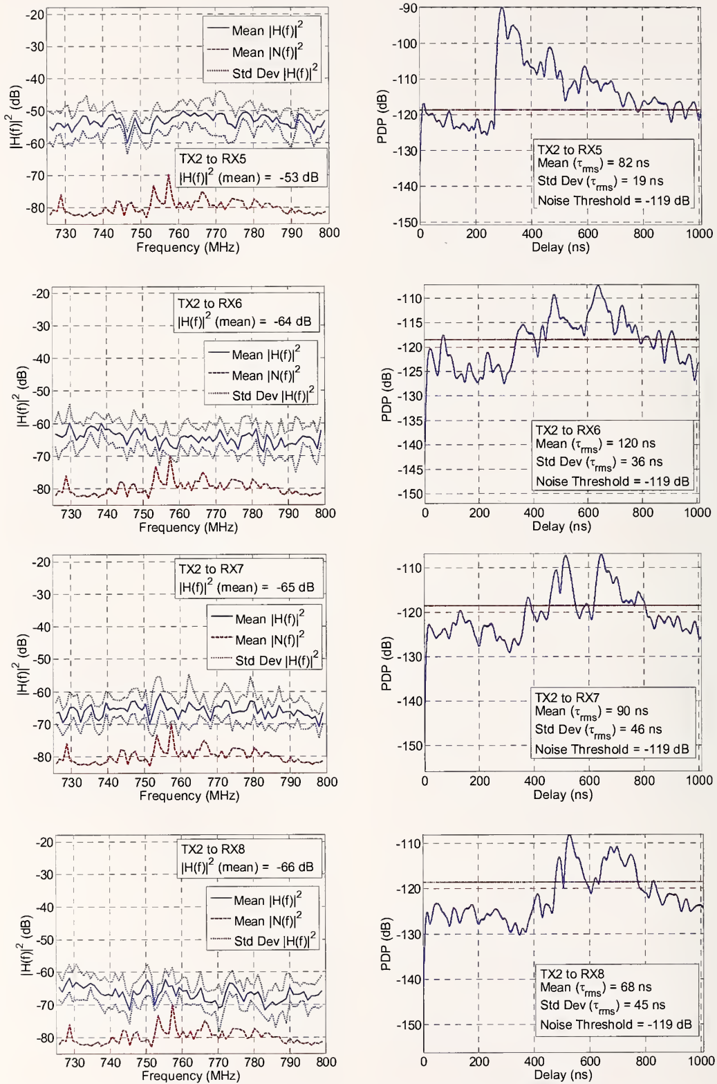
Figure 24. Magnitude squared of the channel performance and PDP for Tx2 to Rx5 through Rx8 pairings in the 700 MHz band.
