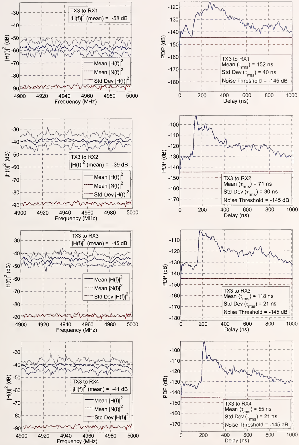
Figure 35. Magnitude squared of the channel performance and PDP for Tx3 to Rx1 through Rx4 pairings in the 4900 MHz band.
