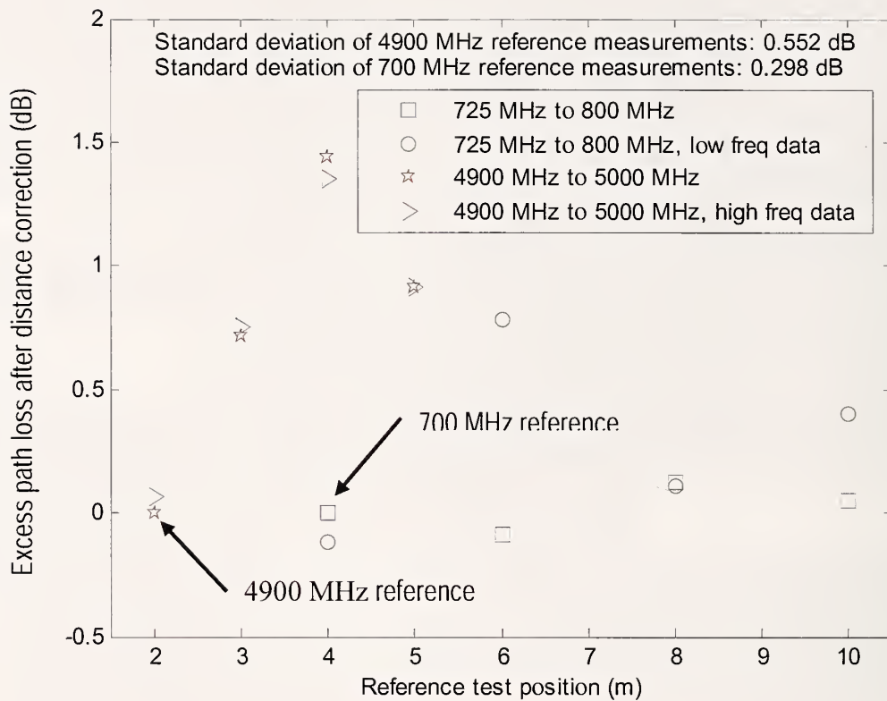
Figure 11. Excess path loss for the reference data collections performed at the NIST outdoor antenna test site. The excess path loss is calculated relative to the 700 MHz and 4900 MHz references, respectively, (i.e., the 0 dB cases), after correcting for separation distances assuming free space propagation.
