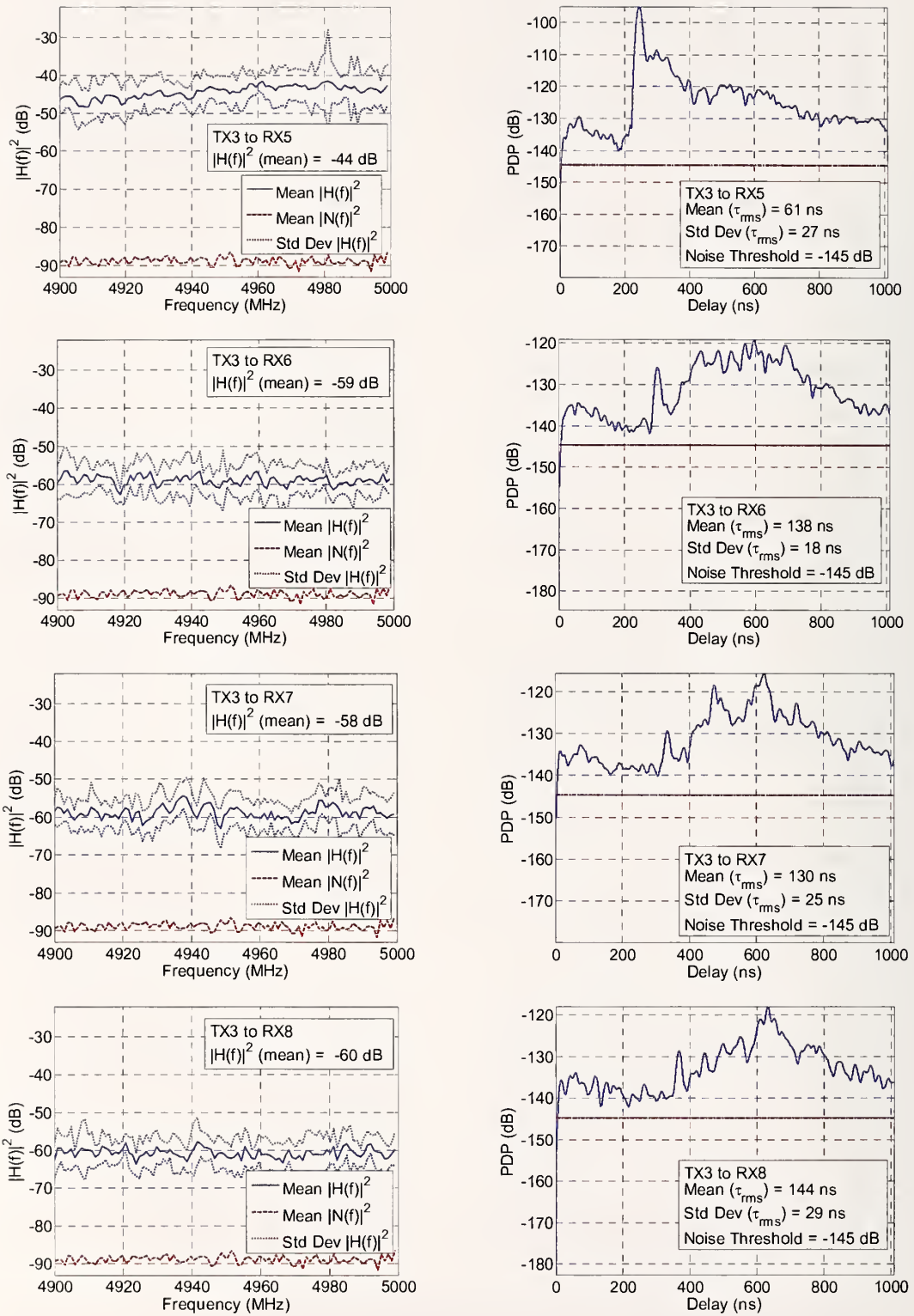
Figure 36. Magnitude squared of the channel performance and PDP for Tx3 to Rx5 through Rx8 pairings in the 4900 MHz band.
