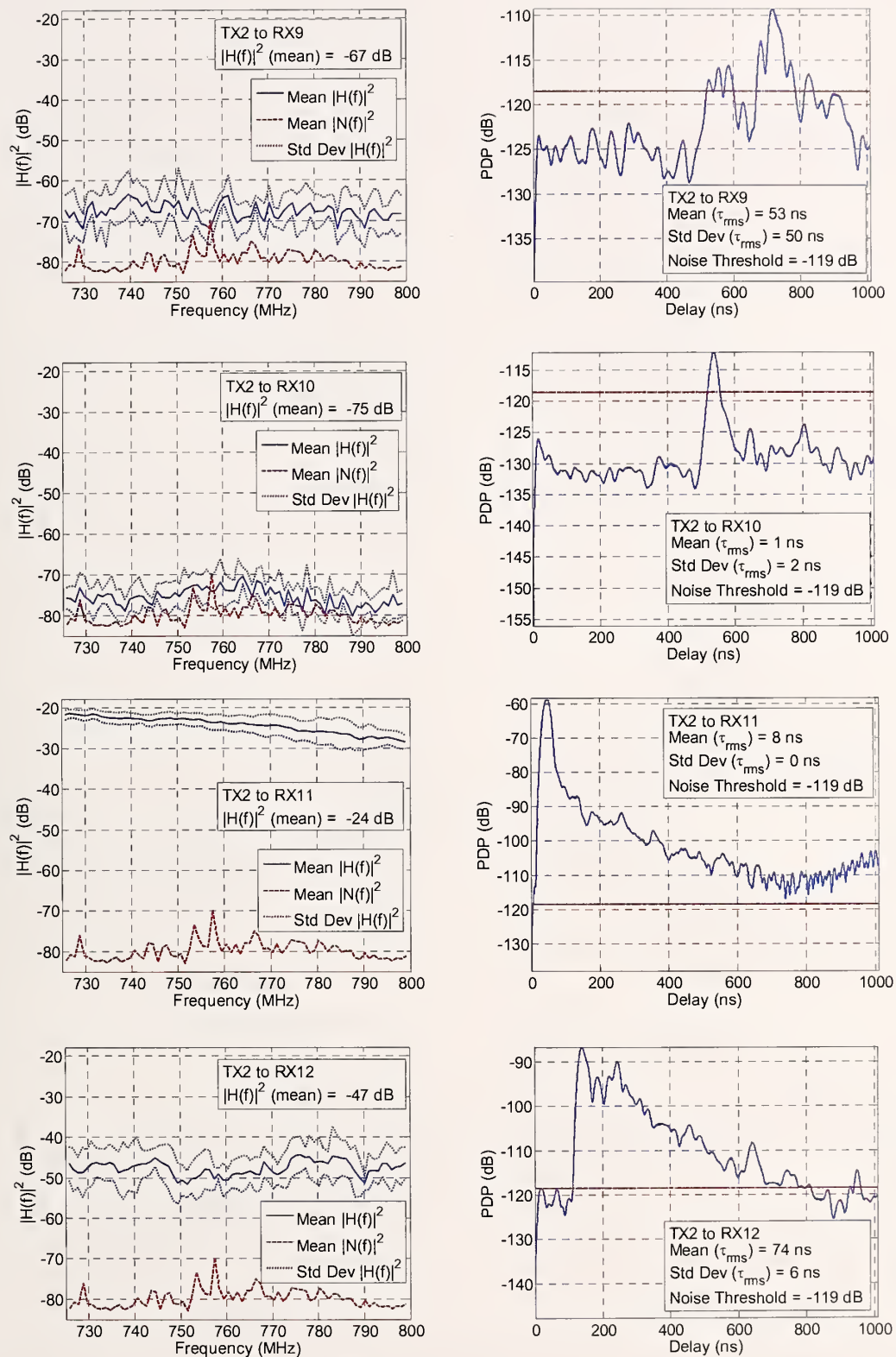
Figure 25. Magnitude squared of the channel performance and PDP for Tx2 to Rx9 through Rx12 pairings in the 700 MHz band.
