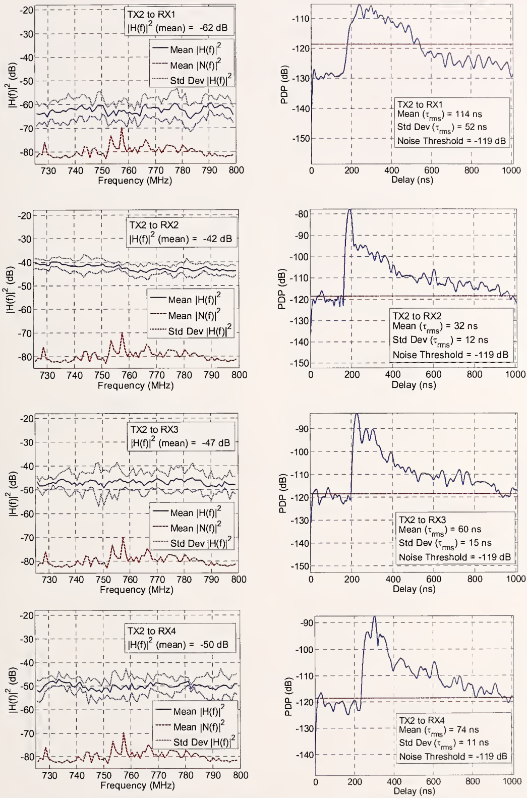
Figure 23. Magnitude squared of the channel performance and PDP for Tx2 to Rx1 through Rx4 pairings in the 700 MHz band.
