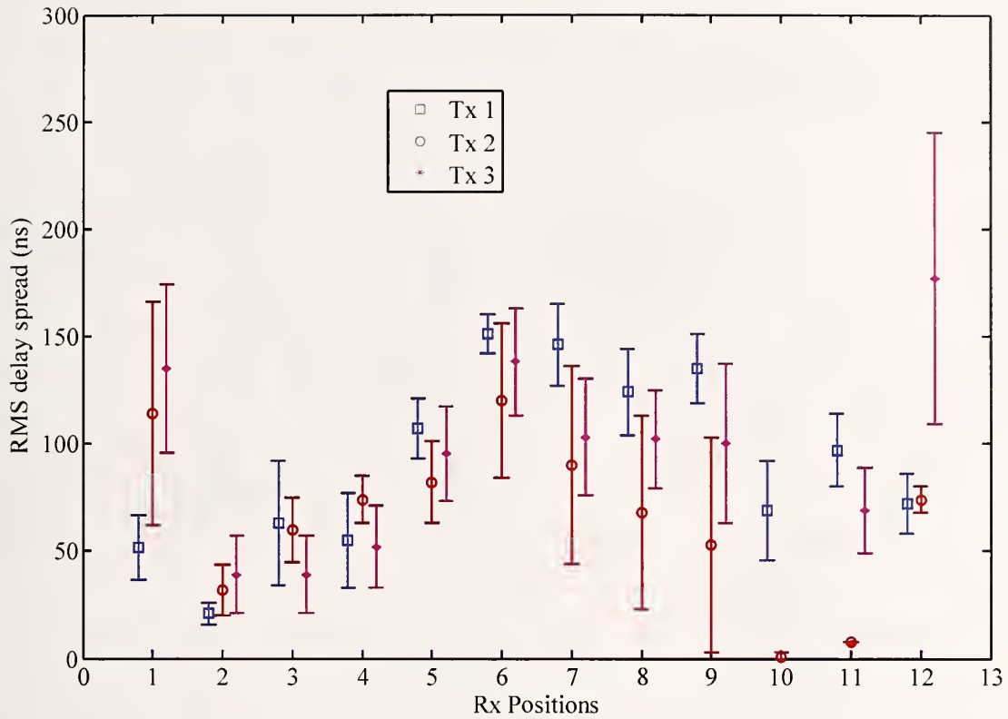
Figure 15. 700 MHz band, mean RMS delay spread \pm \sigma for each receive antenna location for the first transmit location.
