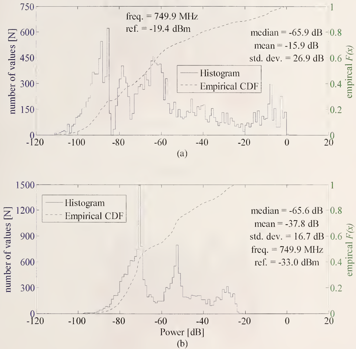
Figure 90. Histogram and empirical CDF of the narrowband receiver signal power at NIST Boulder laboratory for (a) receive site one and (b) receive site two. Path II, walk 2.
