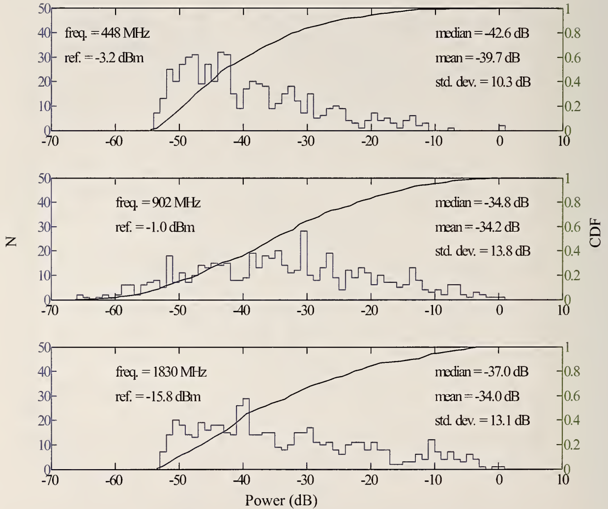
Figure 53. New Orleans, LA apartment building statistics, histograms, and empirical CDF for walk-through data at 448.60, 902.60, and 1832.50 MHz.
