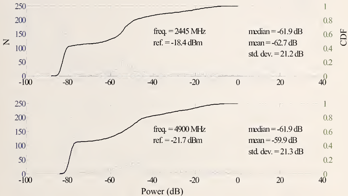
Figure 257. NIST Boulder laboratory statistics, histograms, and empirical CDF for walk-through data at 2445.0 and 4900.0 MHz; receiver at wing 4 site.
