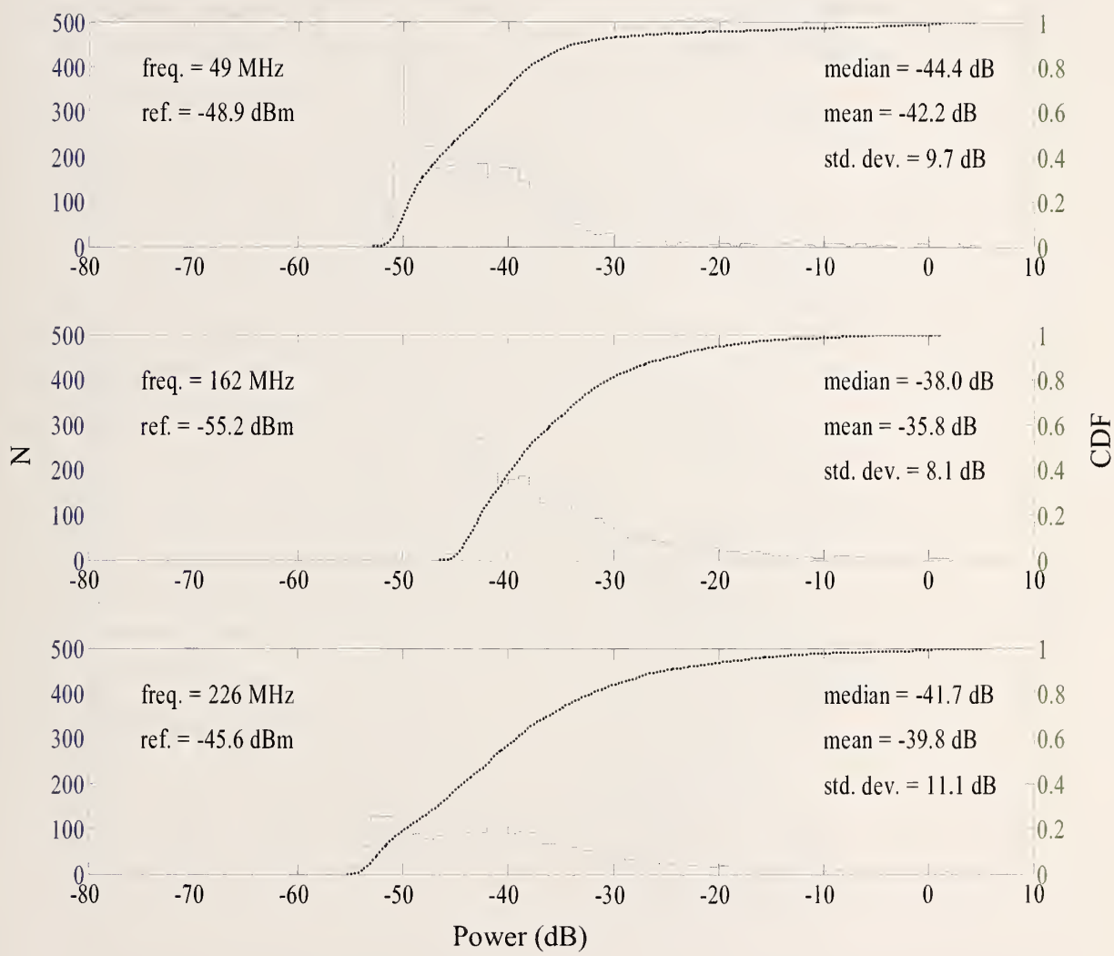
Figure 160. Bethesda, MD shopping mall statistics, histograms, and empirical CDF for walk-through data with the receiver at site 2; 49.60, 162.09, and 226.40 MHz.
