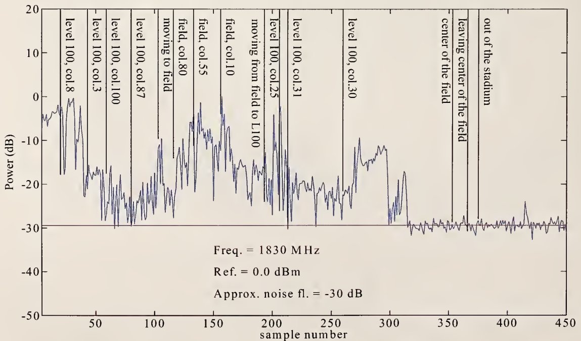
Figure 67. Philadelphia, PA sports stadium second inside walk at 1832.00 MHz; horizontal polarization.
