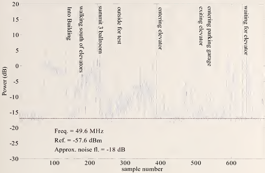
Figure 114. Colorado Springs, CO hotel first walk-through at 49.60 MHz; receiver at site 2.
