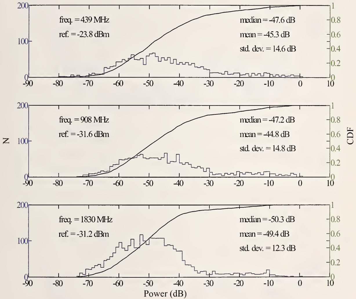
Figure 223. SUNCOR oil refinery statistics, histograms, and empirical CDF for walk-through data at 439.25, 908.0, and 1830.1 MHz; receiver at south site.
