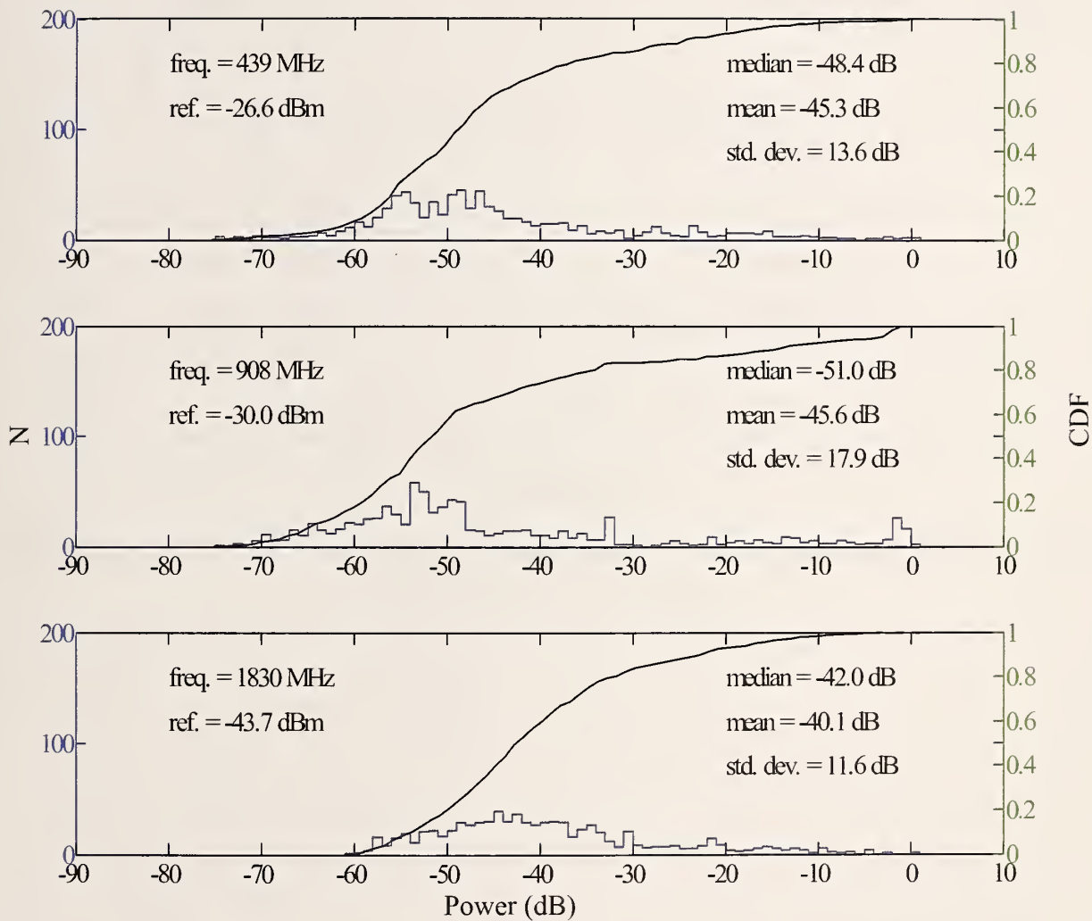
Figure 245. SUNCOR oil refinery statistics, histograms, and empirical CDF for walk-through data at 439.25, 908.0, and 1830.1 MHz.
