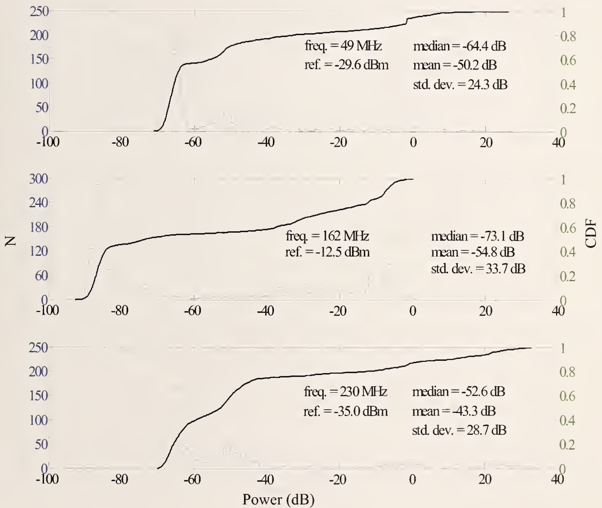
Figure 255. NIST Boulder laboratory statistics, histograms, and empirical CDF for walk-through data at 49.8, 162.075, and 230.0 MHz; receiver at wing 4 site.
