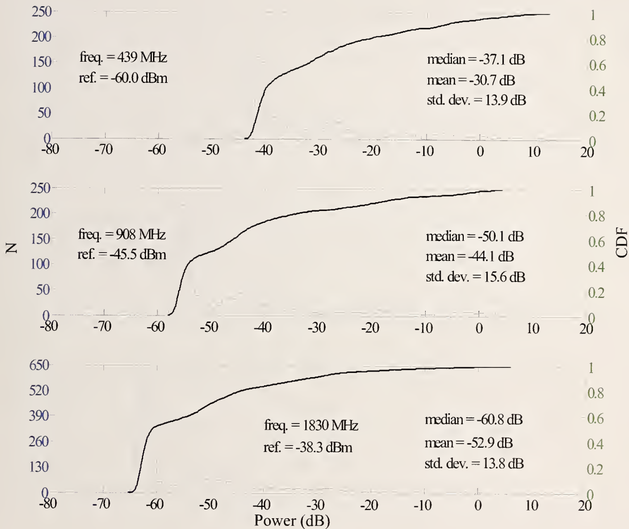
Figure 267. NIST Boulder laboratory statistics, histograms, and empirical CDF for walk-through data at 439.25, 908.0, and 1830.0 MHz; receiver at wing 6 site.
