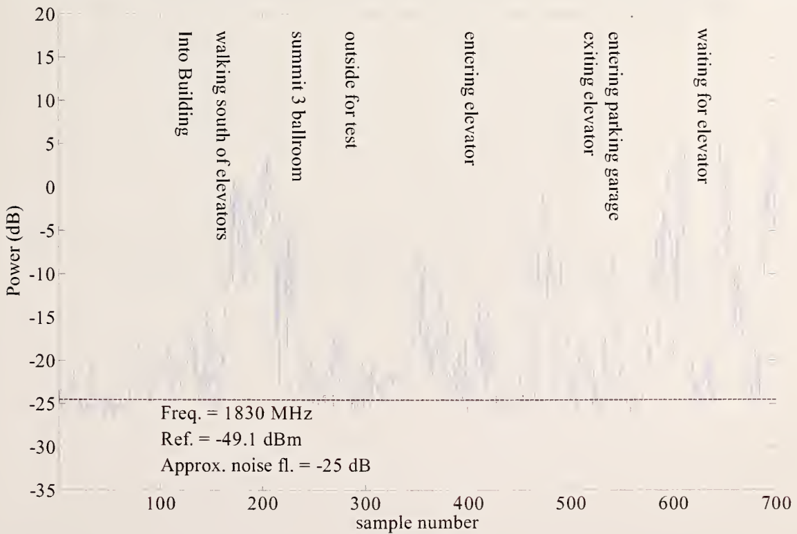
Figure 119. Colorado Springs, CO hotel first walk-through at 1830.00 MHz; receiver at site 2.
