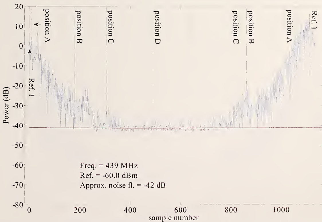
Figure 261. NIST Boulder laboratory walk-through at 439.25 MHz; receiver at wing 6 site.
