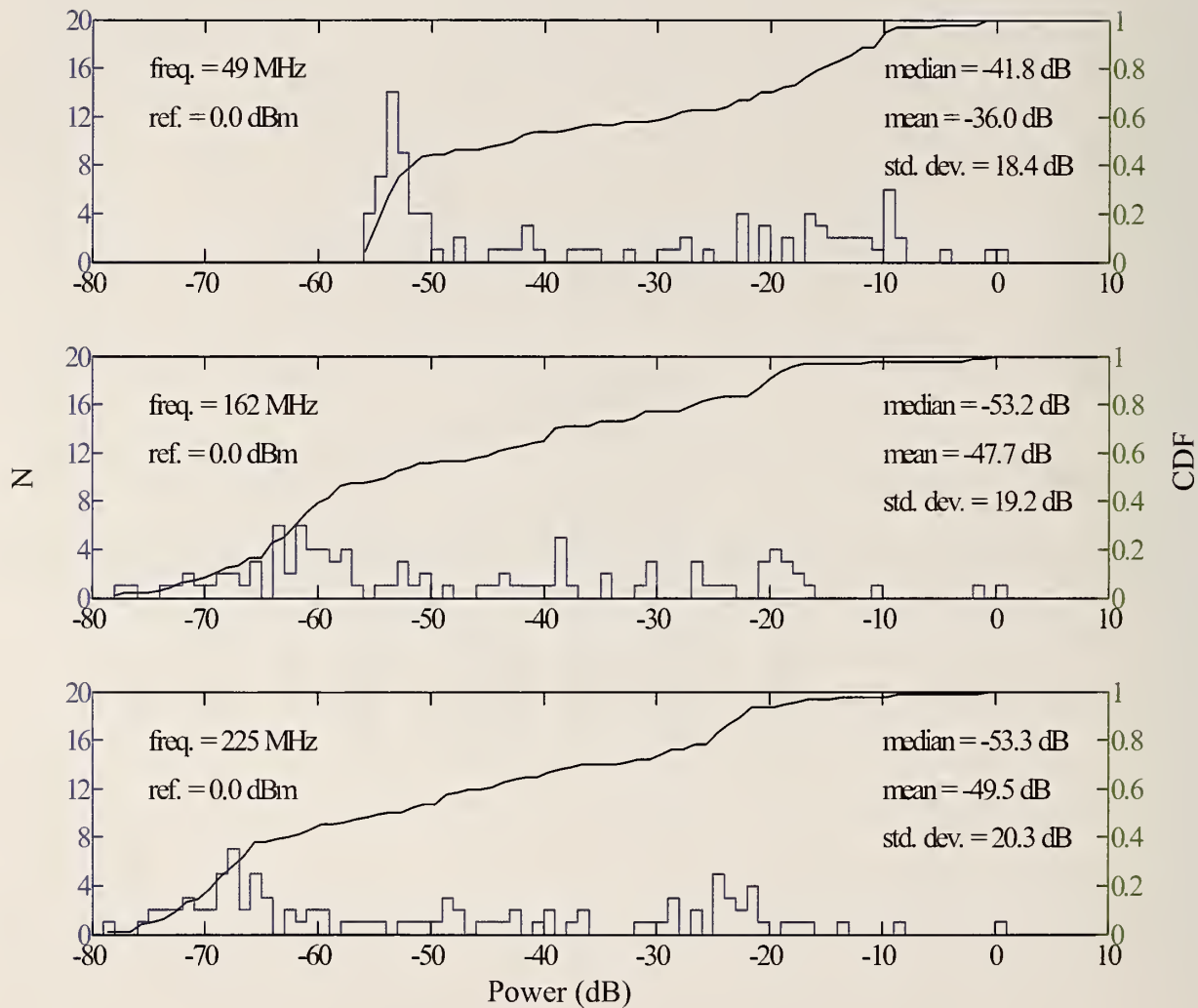
Figure 92. Philadelphia, PA sports stadium statistics, histograms, and empirical CDF for outside walk data at 49.60, 162.09, and 225.30 MHz; vertical polarization.
