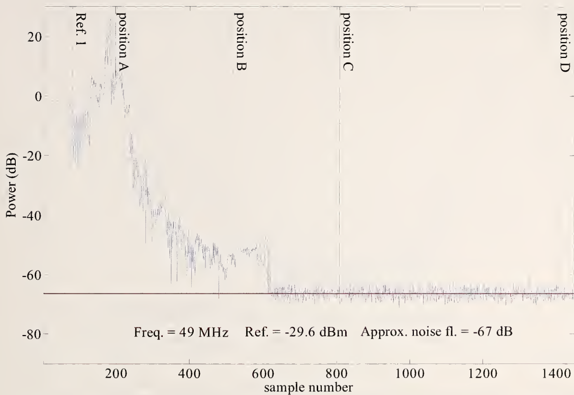
Figure 247. NIST Boulder laboratory walk-through at 49.8 MHz; receiver at wing 4 site.
