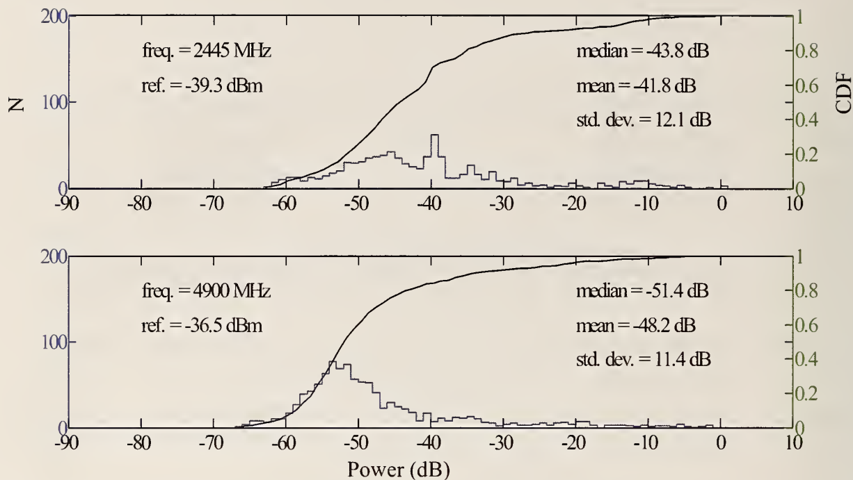
Figure 246. SUNCOR oil refinery statistics, histograms, and empirical CDF for walk-through data at 2445.0 and 4900.0 MHz.
