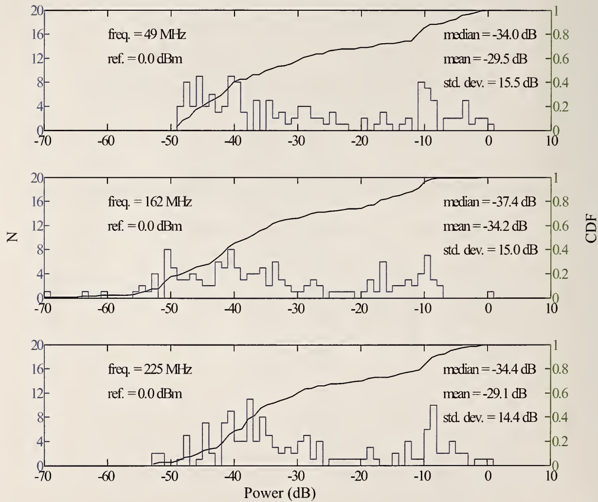
Figure 60. Philadelphia, PA sports stadium statistics, histograms, and empirical CDF for first inside walk data at 49.60, 162.09, and 225.30 MHz; horizontal polarization.
