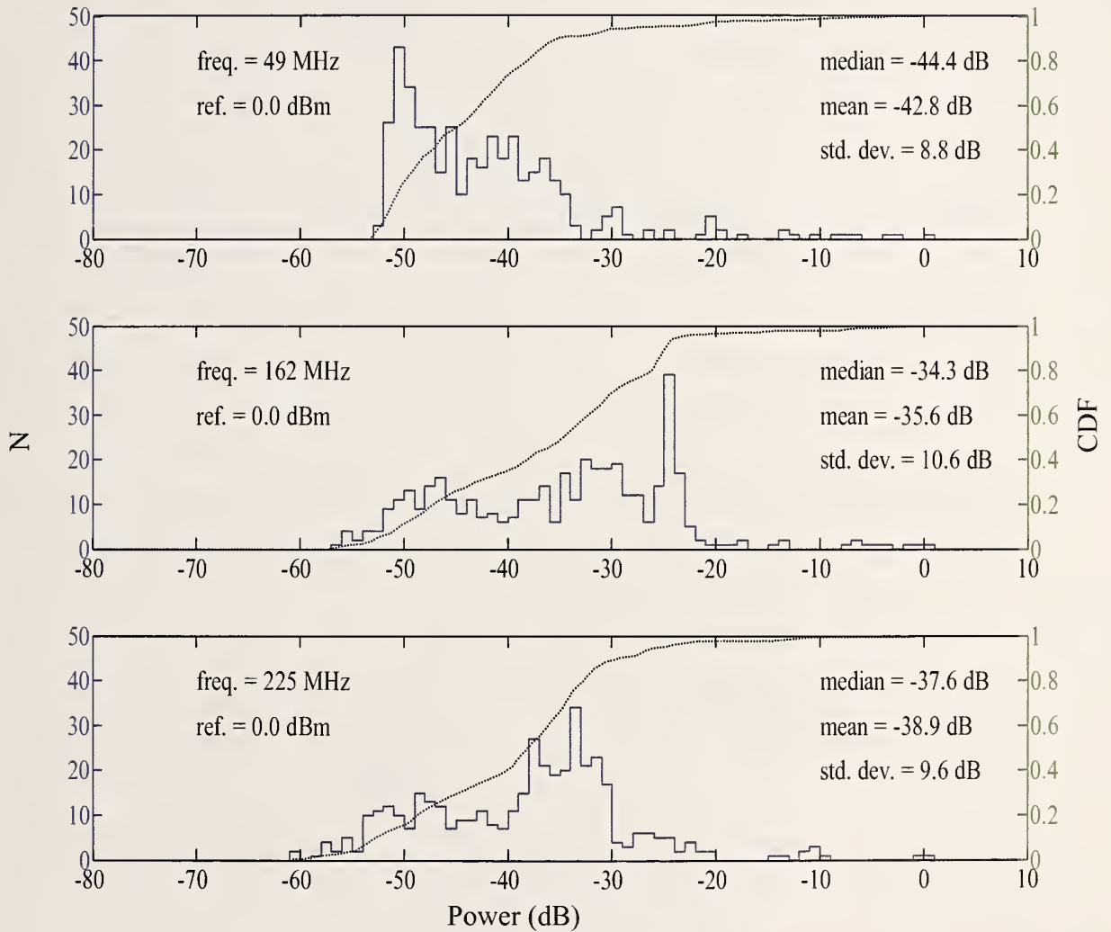
Figure 68. Philadelphia, PA sports stadium statistics, histograms, and empirical CDF for second inside walk data at 49.60, 162.09, and 225.30 MHz; horizontal polarization.
