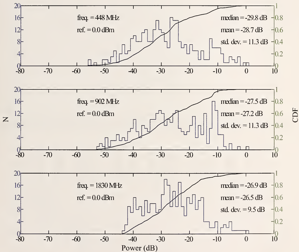
Figure 77. Philadelphia, PA sports stadium statistics, histograms, and empirical CDF for inside walk data at 448.50, 902.45, and 1832.00 MHz; vertical polarization.
