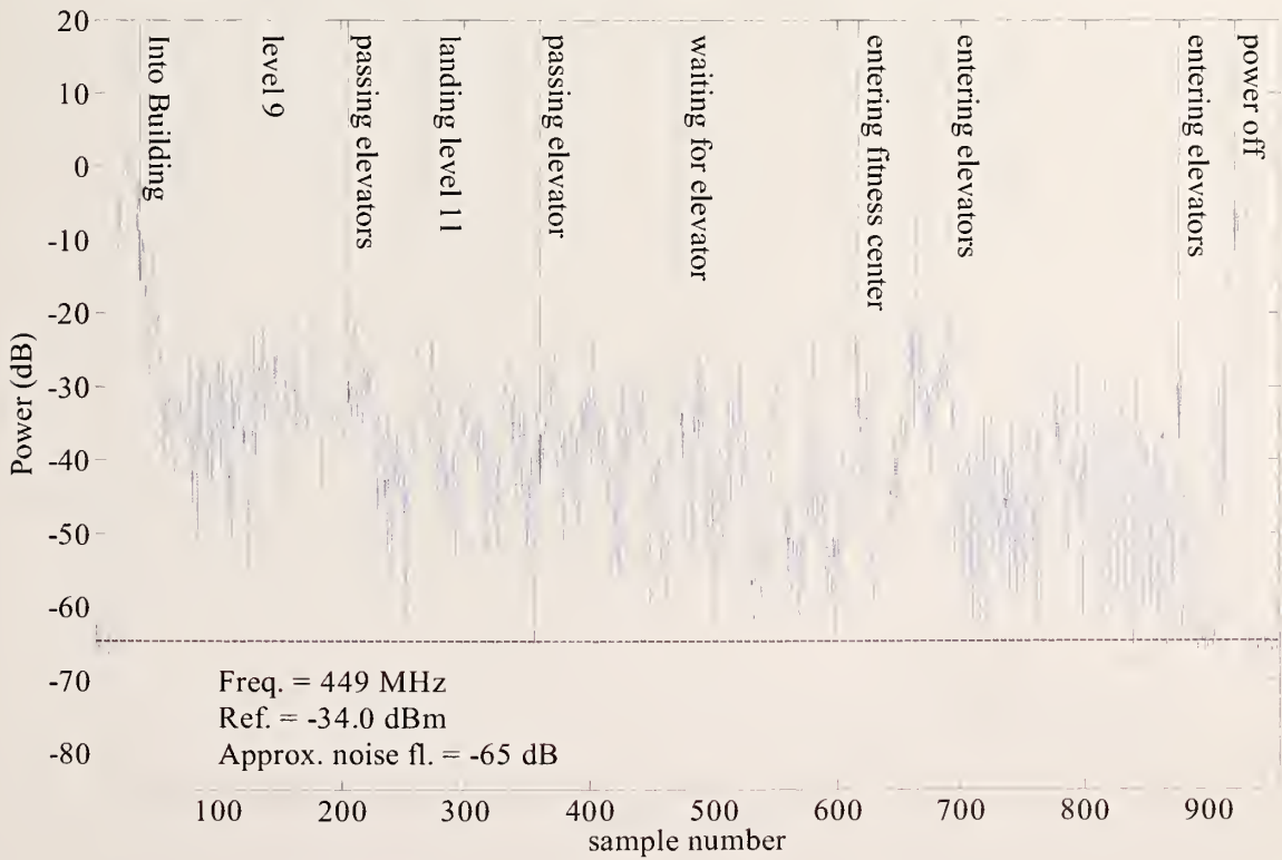
Figure 109. Colorado Springs, CO hotel second walk-through at 448.50 MHz; receiver at site 1.
