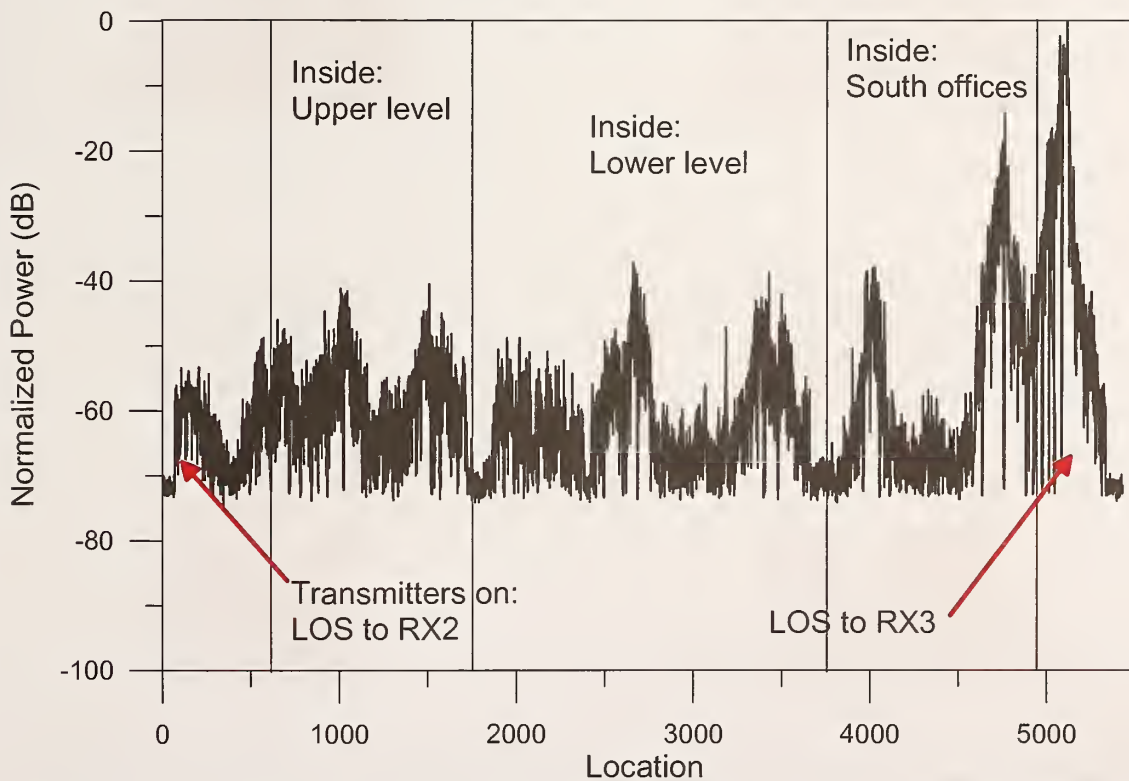
Figure 40. Convention Center walk-through for receiving site RX3 at 1830.00 MHz.
