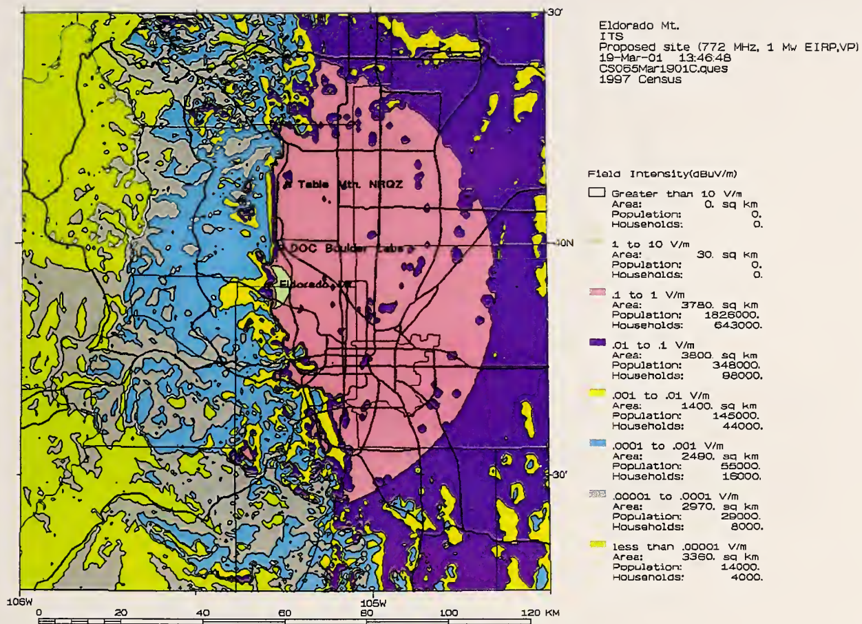
Figure 52. Contour plot of the modeled (or predicted) E-field levels around the Denver-Boulder area for a vertically polarized antenna. These results are for a transmitter on Eldorado Mountain for a frequency of 772 MHz, EIRP=1 MW, a transmitter height of 3.66 m (12 ft), and a receiver height of 2.95 m (9.68 ft).
