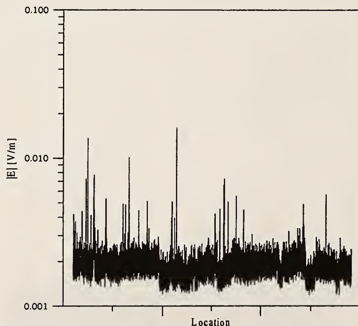
Figure 38. Measured E-field levels scaled to 1 MW EIRP on Greenbriar loop. These results are for a transmitter on Squaw Mountain for a frequency of 533 MHz, a transmitter height of 8.2 m (26.9 ft), and a receiver height of 2.95 m (9.68 ft).
