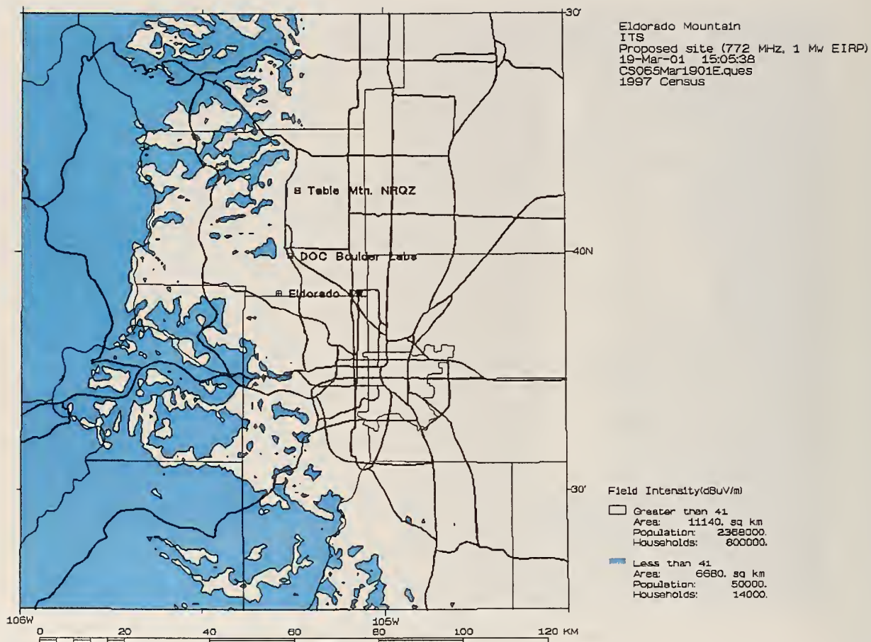
Figure 77. Area coverage plot of the 41 dBμV/m FCC recommendation around the Denver-Boulder area for a horizontally polarized antenna. These results are for a transmitter on Eldorado Mountain for a frequency of 772 MHz, EIRP=1 MW, a transmitter height of 116 m (379 ft), and a receiver height of 9.14 m (30 ft).
