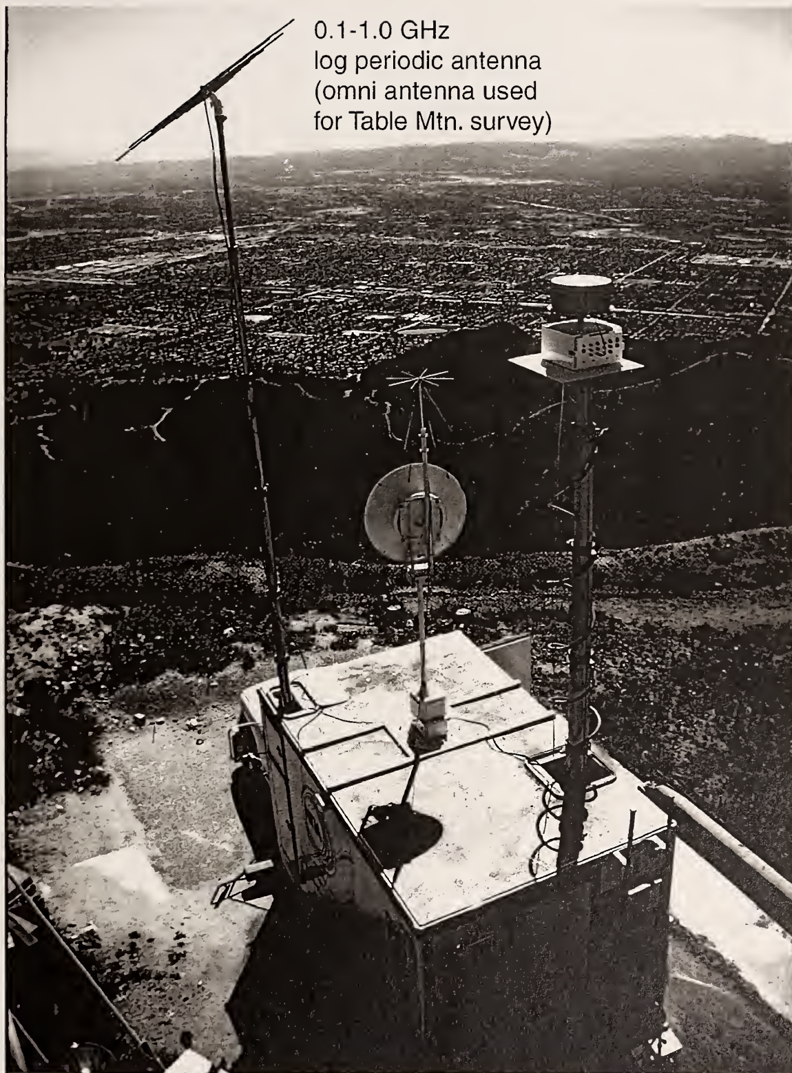
Figure 5. Illustration of the RSMS with telescoping masts raised and antennas mounted for a broadband spectrum survey such as was performed at the Table Mountain NRQZ.
