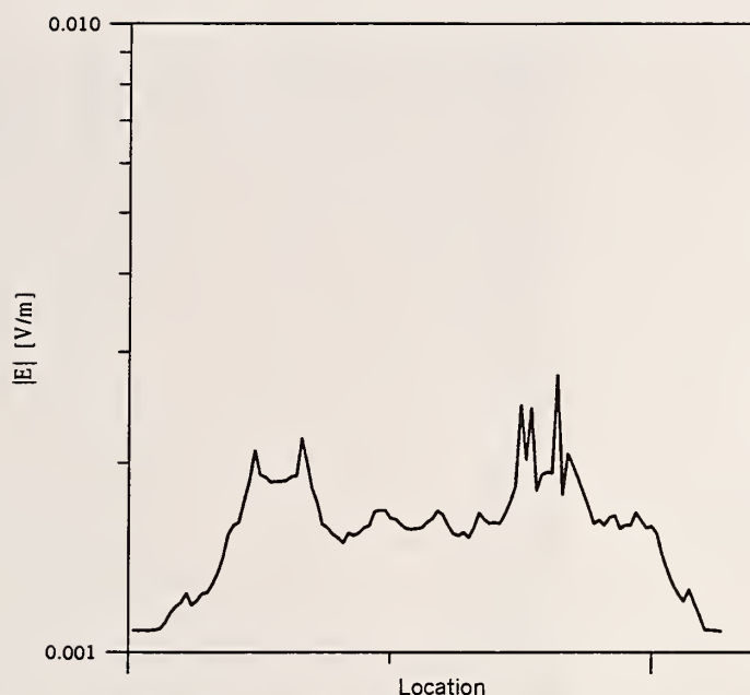
Figure 62. Modeled (or predicted) E-field levels at the Table Mountain NRQZ. These results are for a transmitter on Squaw Mountain for a frequency of 533 MHz, EIRP=1 MW, a transmitter height of 8.20 m (26.91 ft), and a receiver height of 2.95 m (9.68 ft).
