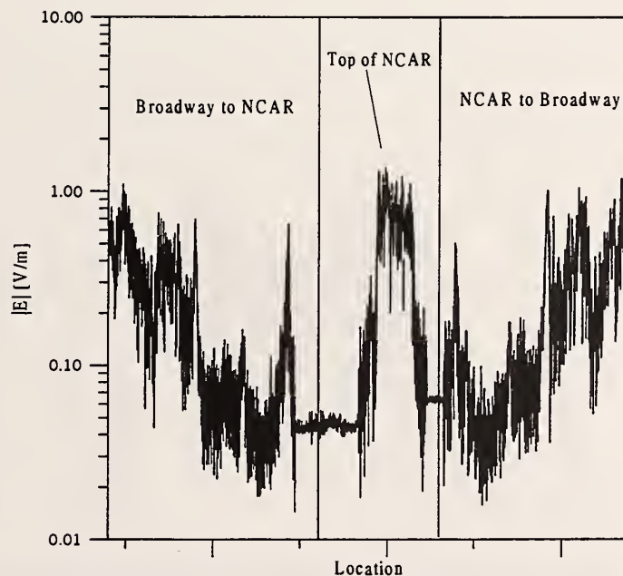
Figure 16. Measured E-field levels scaled to 1 MW EIRP at the NCAR facility at the top of Table Mesa. These results are for a transmitter on Eldorado Mountain for a frequency of 533 MHz, a transmitter height of 3.66 m (12.0 ft), and a receiver height of 2.95 m (9.68 ft).
