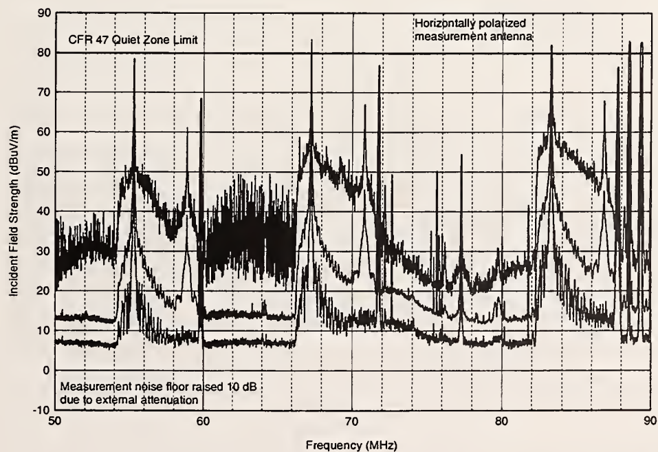
Figure A.35. Table Mountain NRQZ, 50-90 MHz, 10 kHz IF bandwidth, 2,300 sweeps, horizontal polarization.
