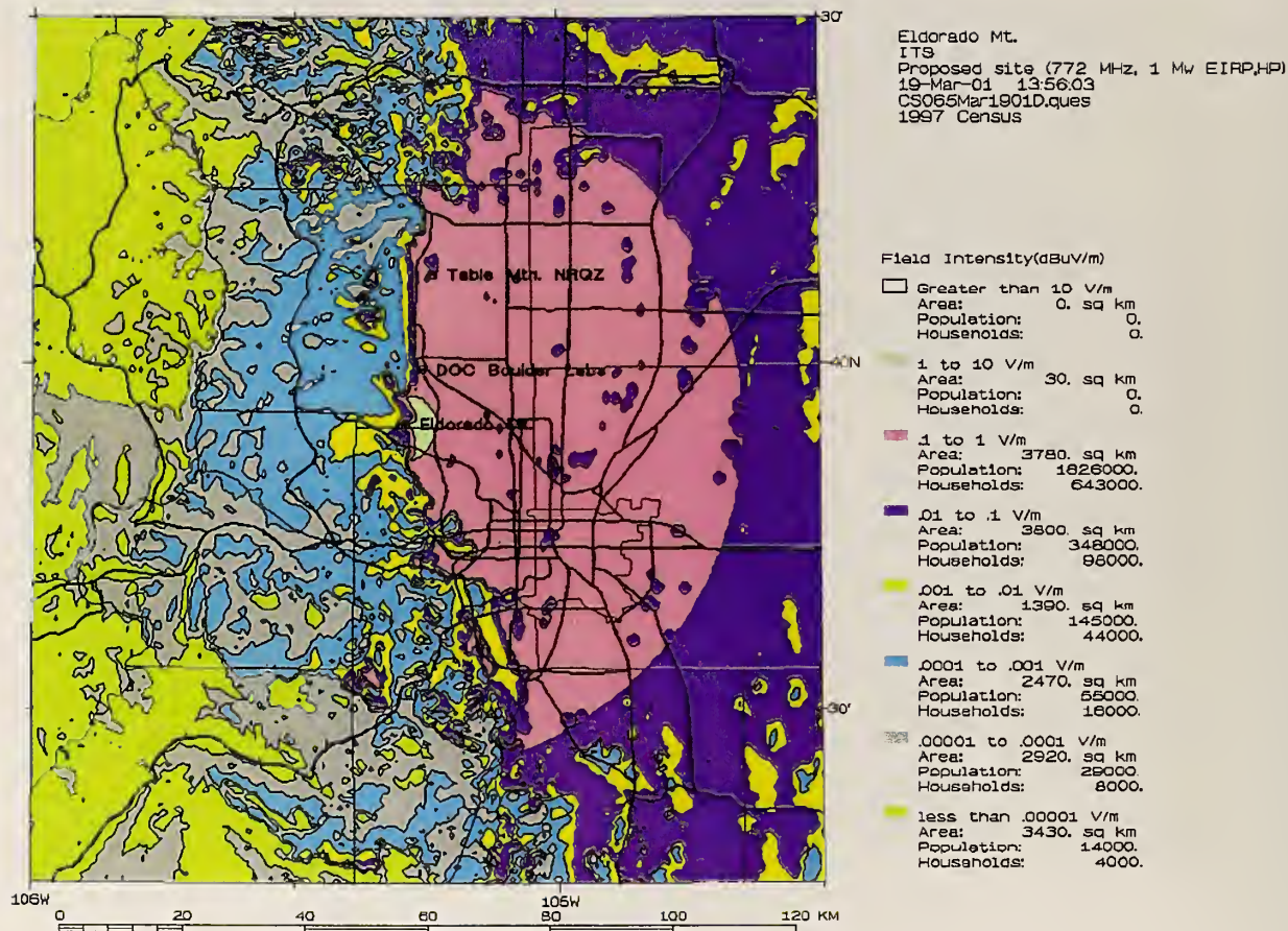
Figure 51. Contour plot of the modeled (or predicted) E-field levels around the Denver-Boulder area for a horizontally polarized antenna. These results are for a transmitter on Eldorado Mountain for a frequency of 772 MHz, EIRP=1 MW, a transmitter height of 3.66 m (12 ft), and a receiver height of 2.95 m (9.68 ft).
