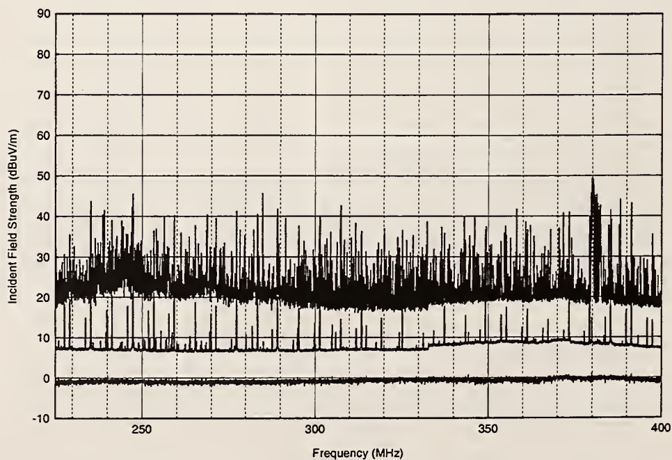
Figure A.25. NIST groundscreen, 225-400 MHz, 30 kHz IF bandwidth, 9,600 sweeps, vertical polarization.
