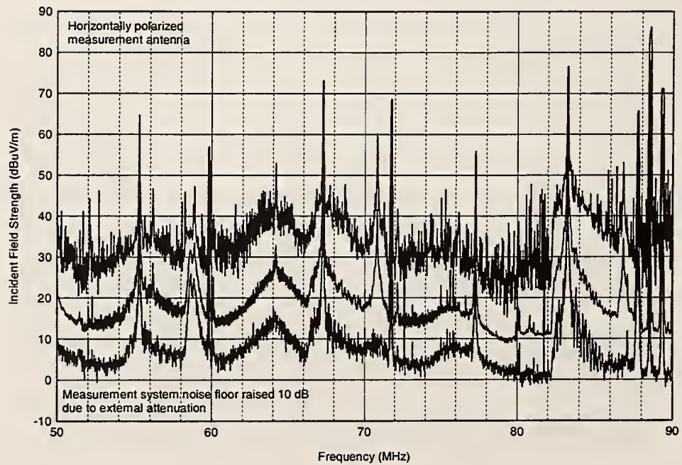
Figure A.37. Bldg. 1, Wing 4, 50-90 MHz, 10 kHz IF bandwidth, 2,100 sweeps, horizontal polarization.
