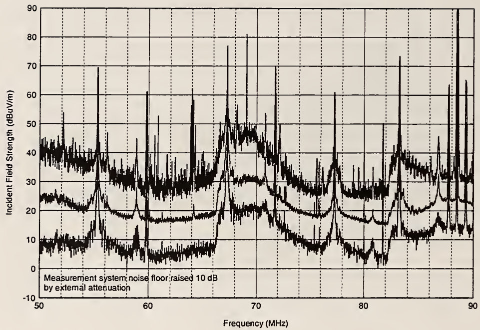
Figure A.36. NIST groundscreen, 50-90 MHz, 10 kHz IF bandwidth, 700 sweeps, horizontal polarization.
