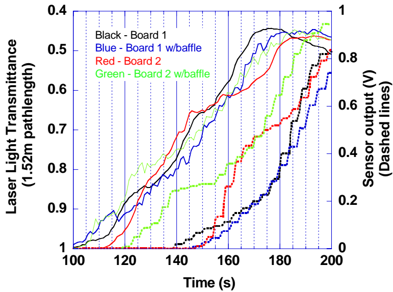
Figure 74. Photo-3 response, fan speed 5 Hz - repeat test
