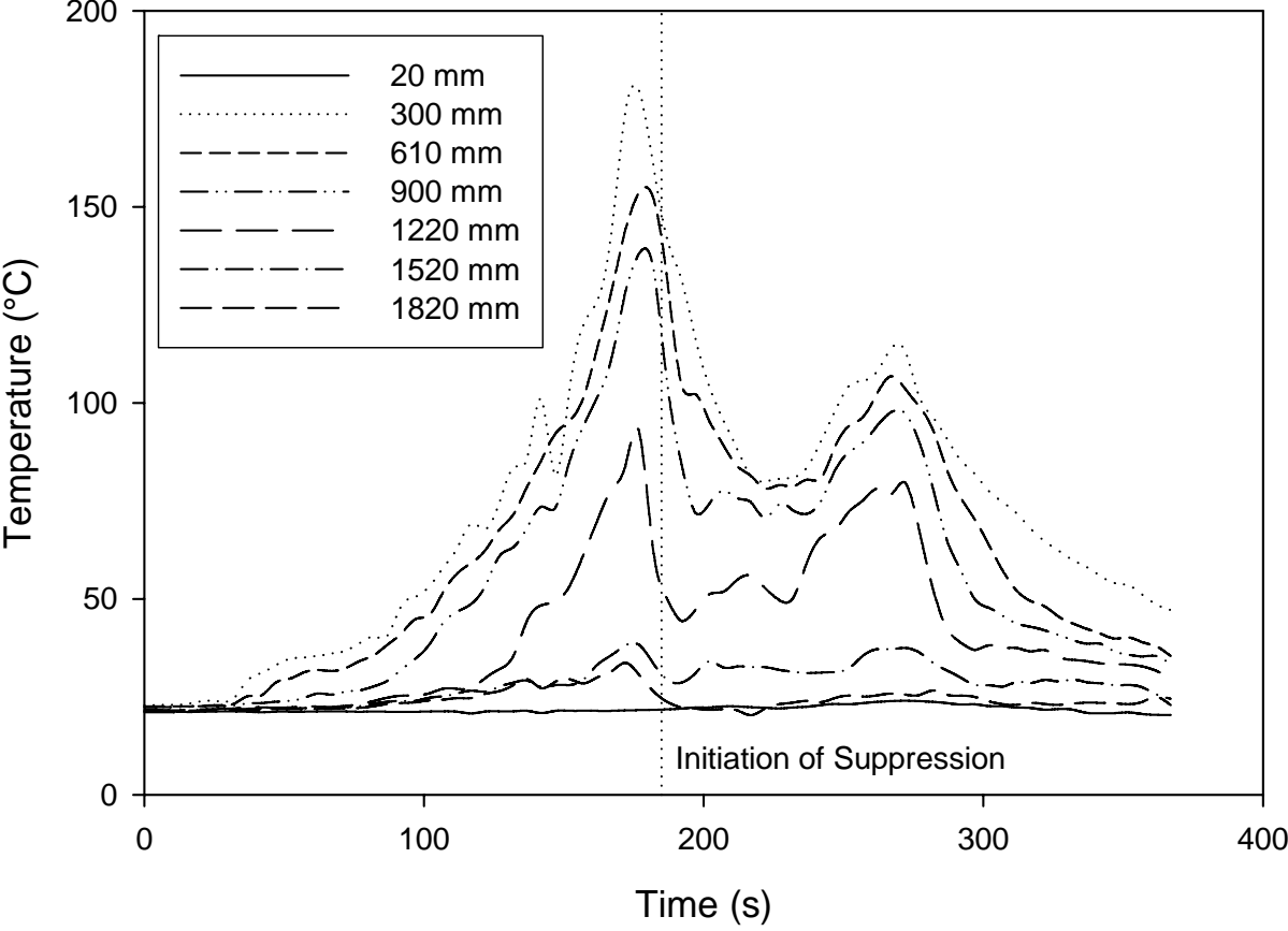
Figure 102. Gas temperatures from ceiling to floor in main bedroom (ignition location) during a flaming ignition test of a mattress, test SDC05
