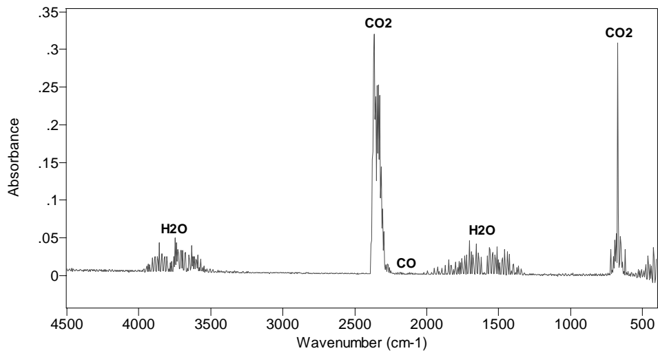
Figure 9. 2-min average of spectra from fire location before water discharge in Test 2
