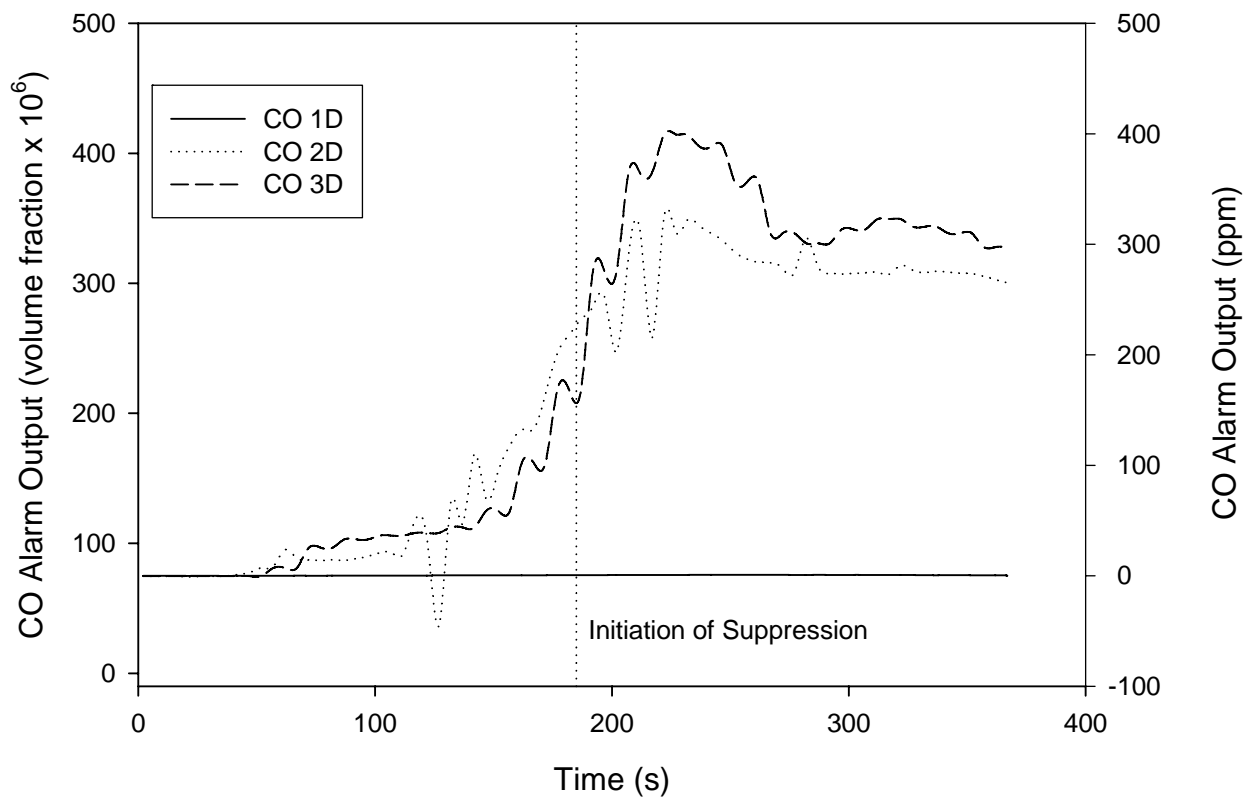
Figure 119. Measured output for several analog-modified carbon monoxide alarms in hallway outside main bedroom during a flaming ignition test of a mattress, test SDC05
