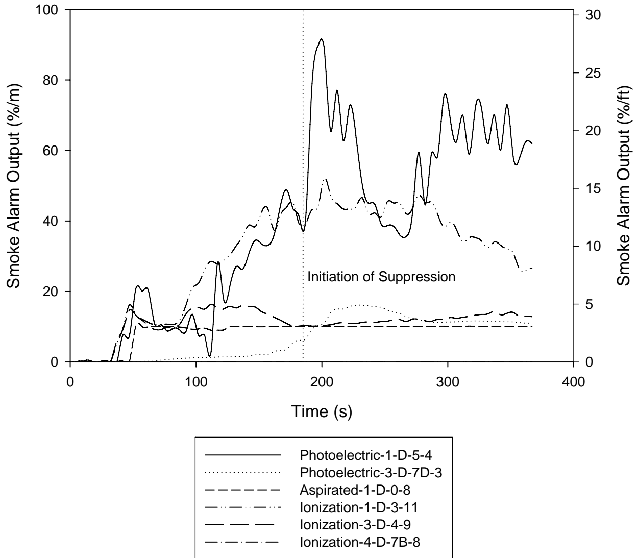
Figure 118. Measured output for several analog-modified smoke alarms in hallway outside main bedroom during a flaming ignition test of a mattress, test SDC05
