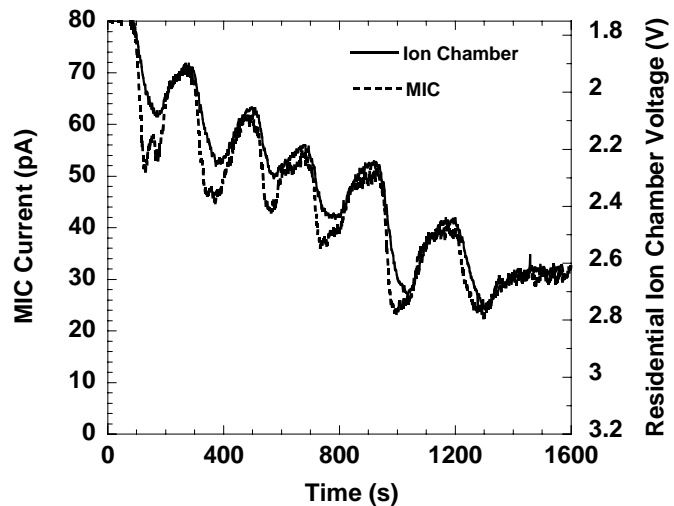
Figure 143. Response of the ion chamber and MIC to cotton smolder smoke
