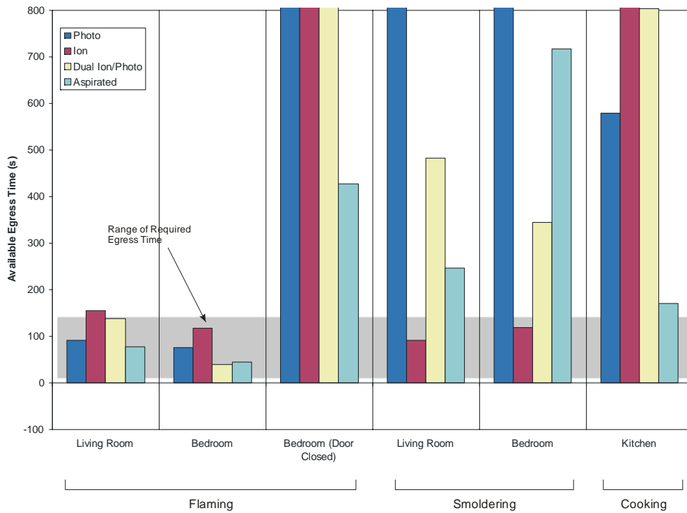
Figure 207. Average available egress time for several different alarm and fire types with alarms on every level + bedrooms for manufactured home tests
