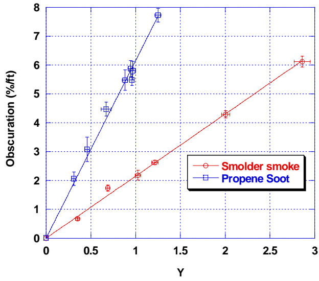
Figure 11. Calibration runs for Ion-1 alarm
