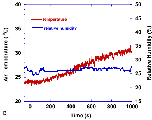
Figure 170. Broiling hamburgers - four hamburgers in oven set on broil, floor fan off. Oven on at t=0
