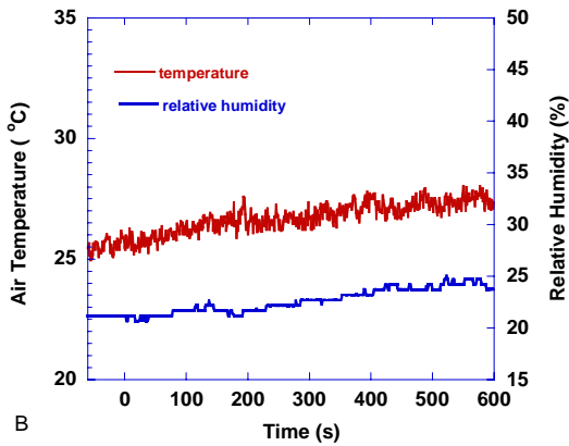
Figure 163. Frying hamburgers - three hamburgers in non-stick frying pan, floor fan on, living room window open. Hamburgers in pan at t=160 s
