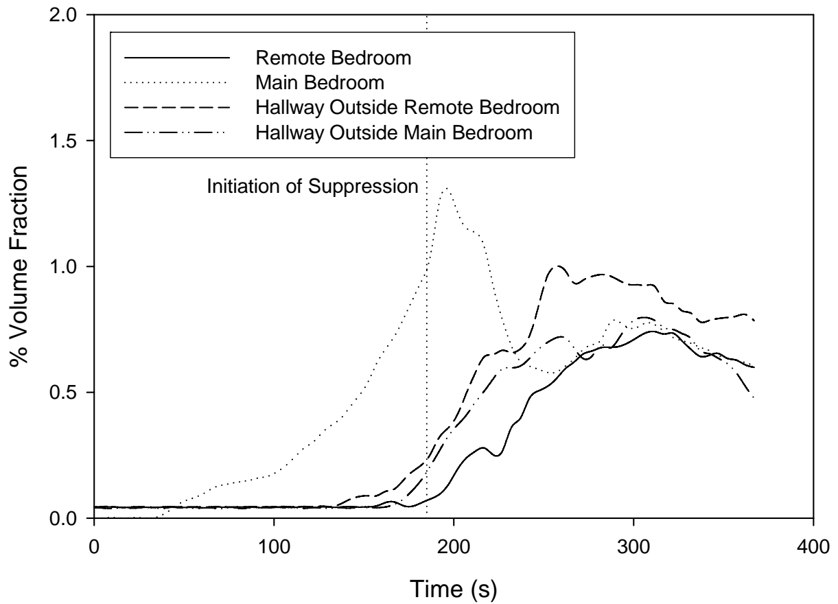
Figure 116. Carbon dioxide concentration 900 mm below ceiling at four locations during a flaming ignition test of a mattress, test SDC05
