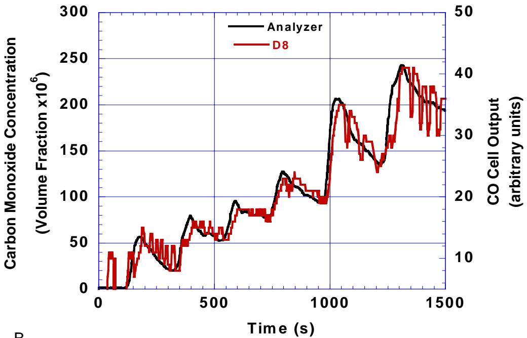
Figure 188. Electrochemical cell CO sensor response to cotton smolder smoke calibration test. A and B indicate repeated tests
