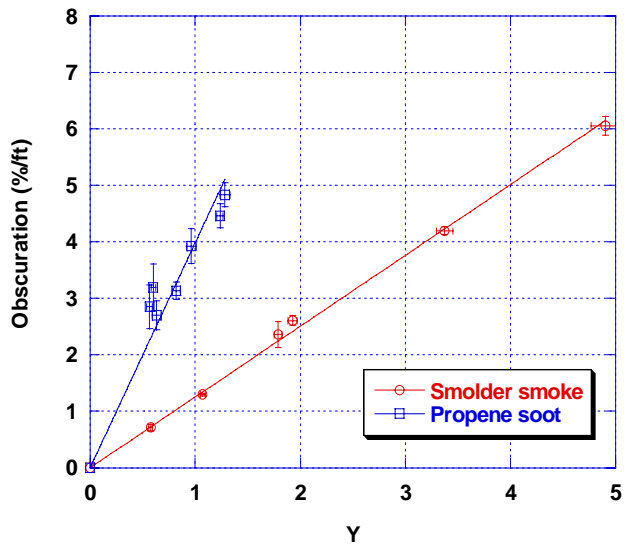
Figure 12. Calibration runs for Ion-3 alarm
