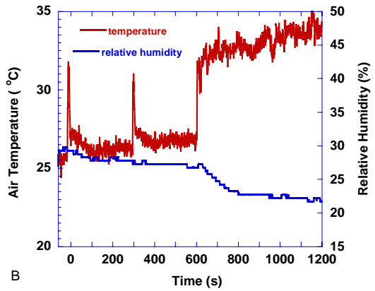
Figure 168. Bake/ broil pizza - one frozen pizza in oven set on bake and pre-heated to 350 °F, then set to broil 630 s later. Floor fan was off. Pizza in at t=0
