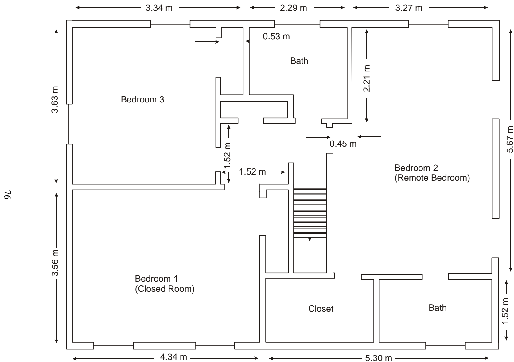
Figure 89. Layout of second floor of two-story home used for tests of smoke alarm performance
