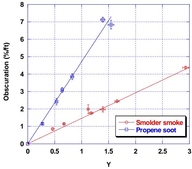
Figure 13. Calibration runs for Ion-4 alarm
