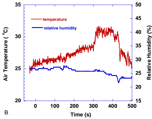
Figure 159. Frying butter scenario - cast iron pan, electric range, floor fan off, butter in pan at t=0
