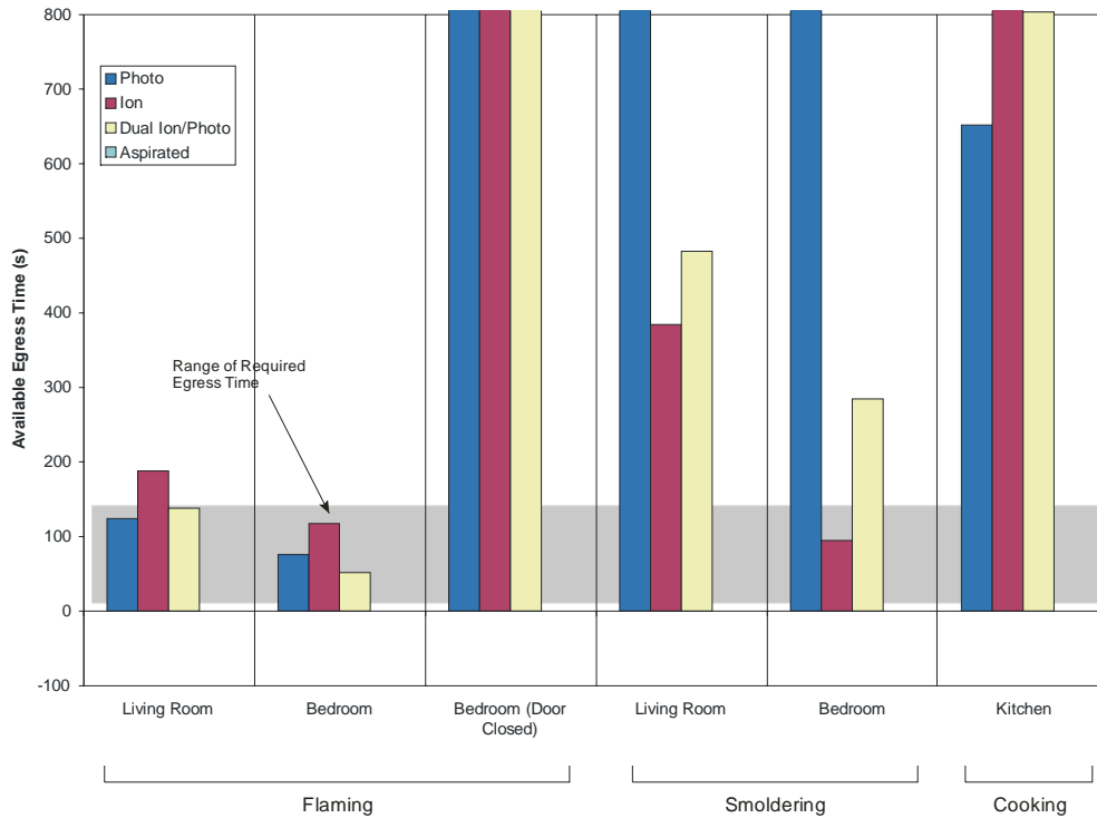
Figure 208. Average available egress time for several different alarm and fire types with alarms in every room for manufactured home tests
