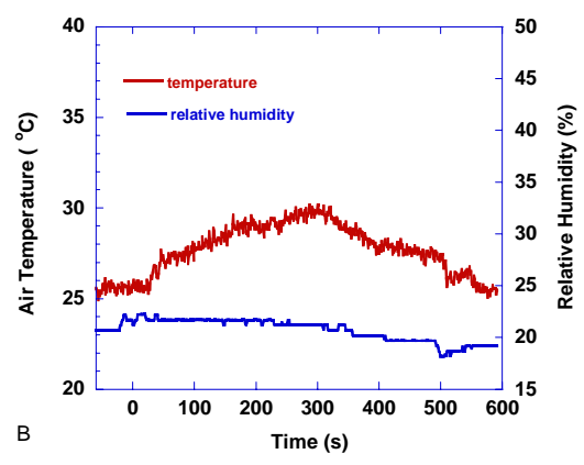
Figure 151. Toasting frozen bagel scenario – toaster on at t=0, off at 300 s. Room fan turned off
