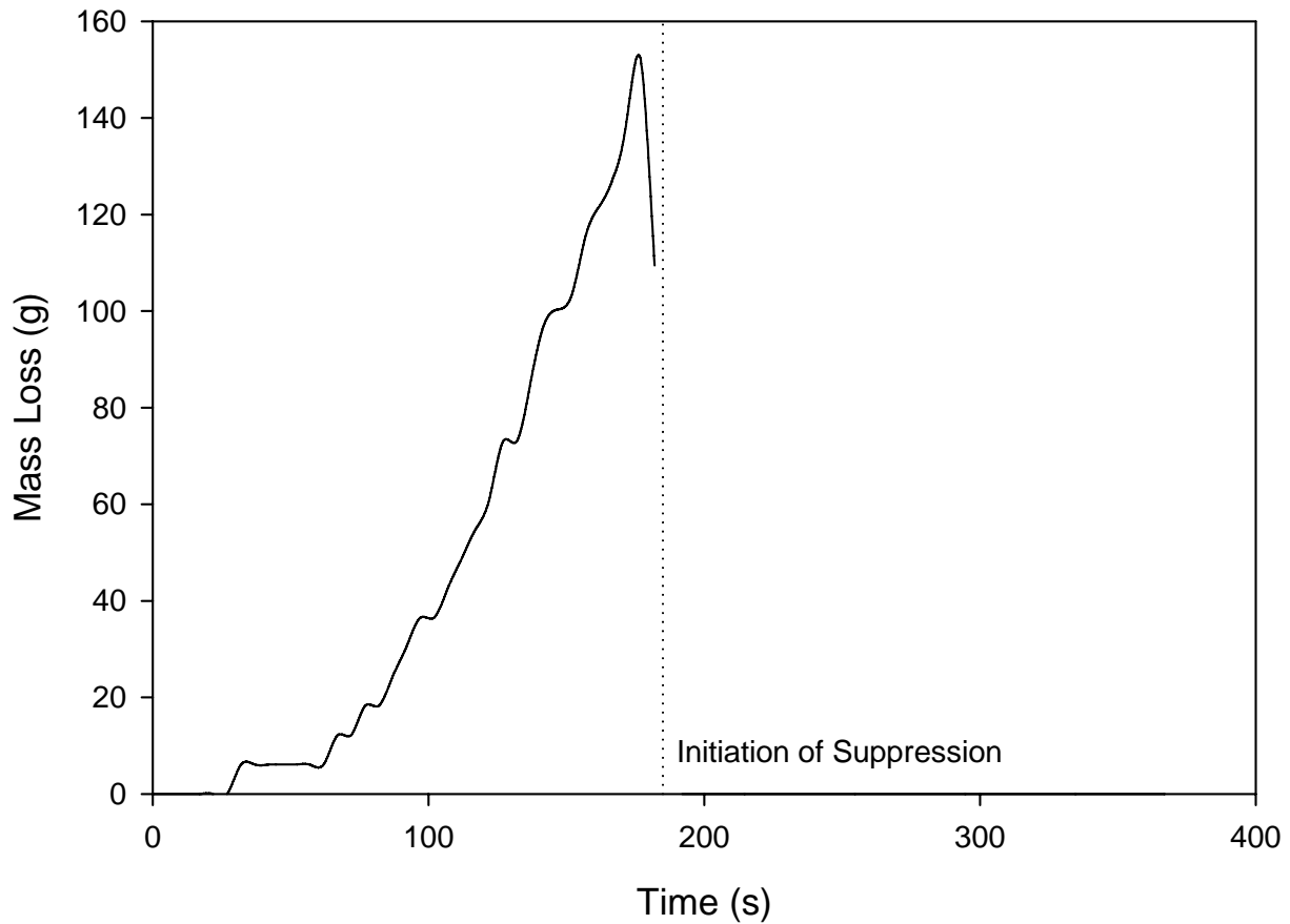
Figure 100. Mass loss of burning mattress during flaming ignition test of a mattress, test SDC05 (Note that the mass loss is averaged to minimize noise in the data. Thus, peak mass loss and initiation of suppression do not exactly coincide)
