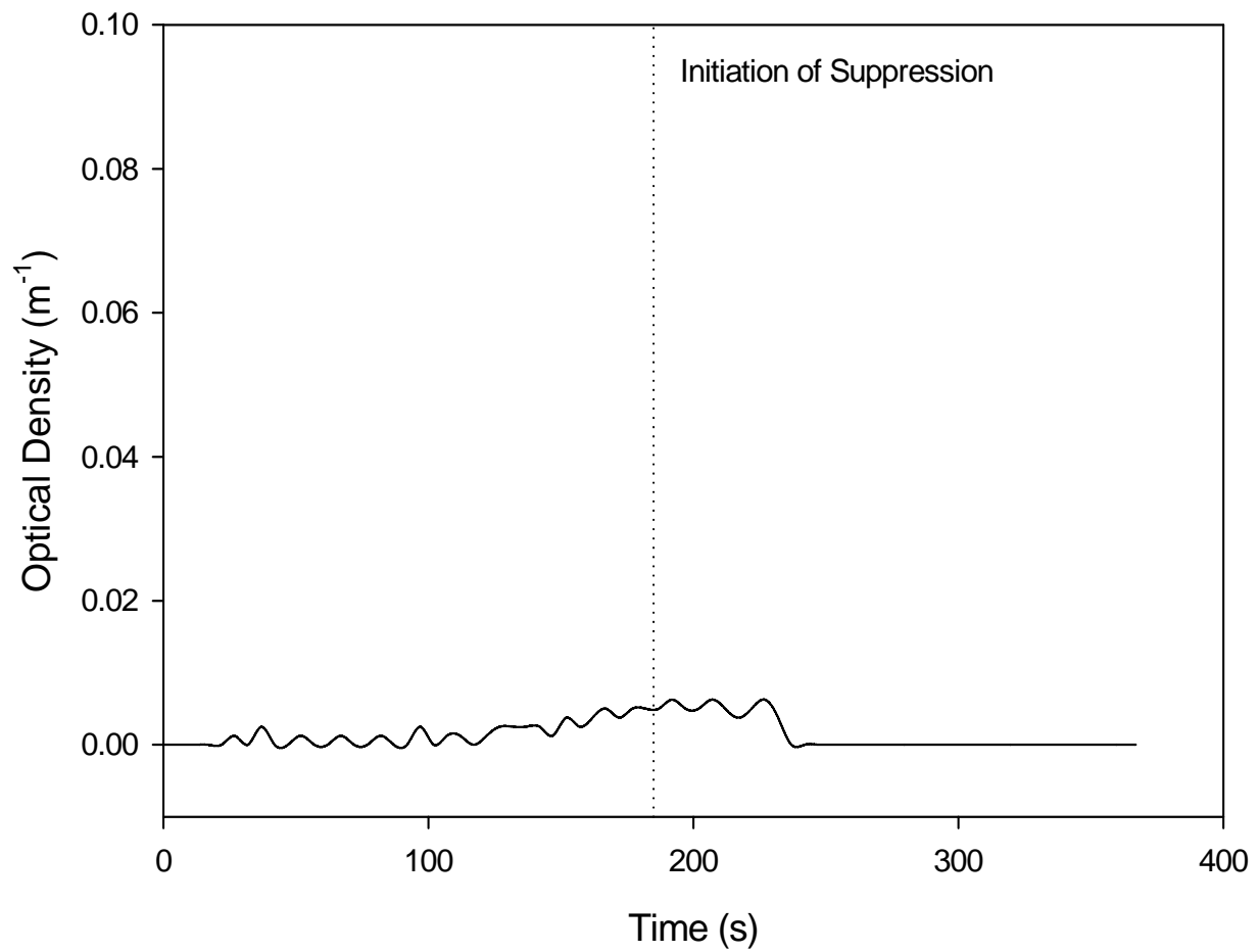
Figure 114. Smoke obscuration at 1520 mm below ceiling in closed bedroom during flaming ignition test of a mattress, test SDC05
