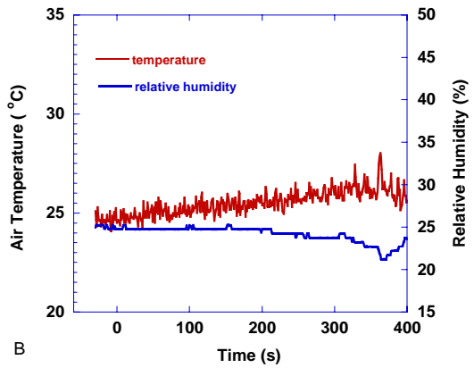
Figure 160. Frying butter scenario - cast iron pan, electric range, floor fan on, butter in pan at t=0
