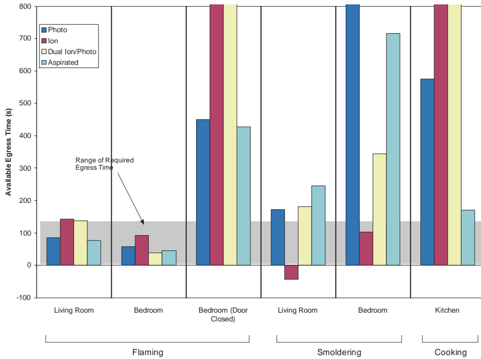
Figure 206. Average available egress time for several different alarm and fire types with alarms on every level for manufactured home tests
