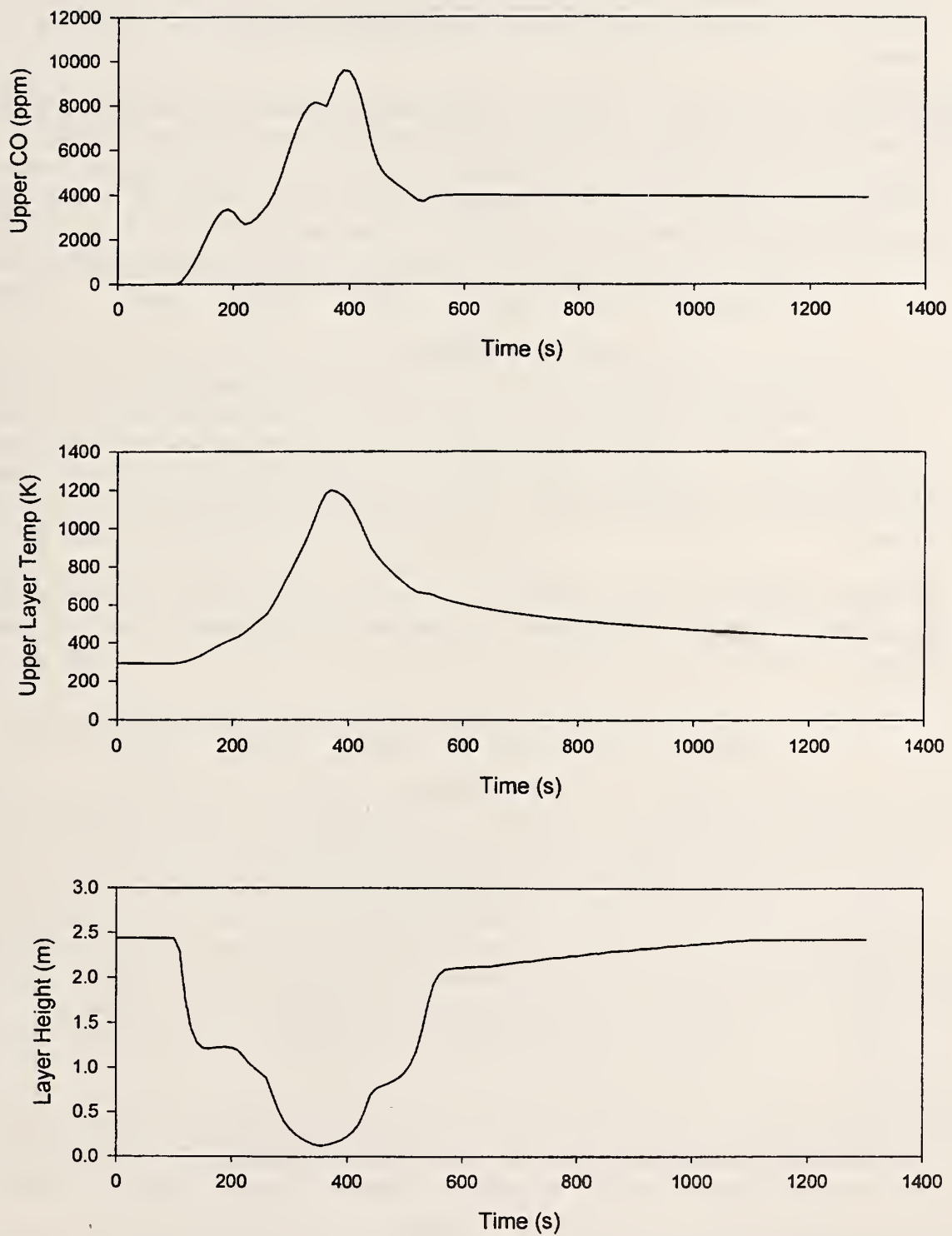
Figure 15a. CFAST calculated results for fire room with an M1 twin bed fire; 3.66 m by 3.66 m (12 ft by 12 ft) room with a fully open door. Top graph, ppm of CO in upper layer; middle graph, temperature of upper layer gases; lower graph, height of base of upper layer.
