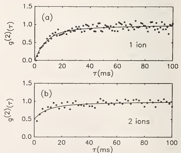
FIG. 2. Plots of g^{(2)}(\tau) for (a) one \text{Hg}^+ ion and (b) two \text{Hg}^+ ions. The dots represent the experimental data. The solid lines are calculated from Eq. (4).
