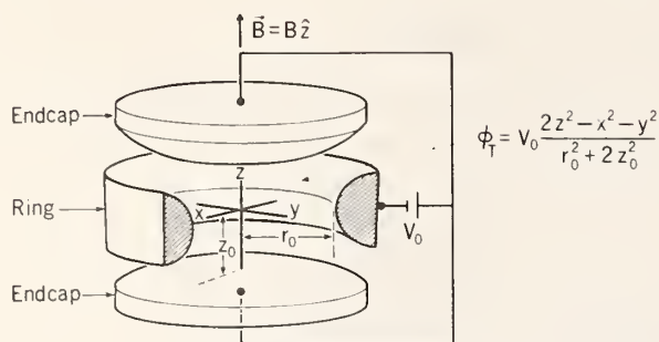
FIG. 1. Penning trap. The two endcap electrodes are biased with respect to the ring electrode by a voltage V_0 . The quadrupole trap potential is a consequence of the shape of the electrodes, which are hyperboloids of revolution. We neglect the distortion of the potential from the effects of truncation and holes in the electrodes. The motion of the ions in a direction perpendicular to the trap axis is constrained by the trap magnetic field. Ions are prevented from escaping along the magnetic field lines by the quadrupole electric field. Two coordinate systems are used in this paper: the Cartesian and cylindrical coordinate systems.
