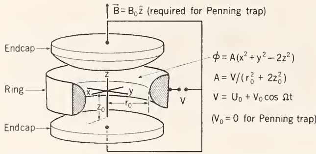
FIG. 2. Electrode configuration for an rf (Paul) or Penning trap. The inner surfaces of the electrodes are assumed to be equipotentials of \phi , and the effect of truncating the electrodes is neglected. r_0 is the inner radius of the ring electrode and 2z_0 is the endcap-to-endcap spacing.
