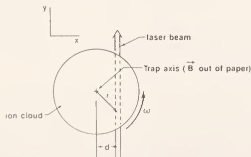
Fig. 3. Laser beam-ion cloud interaction geometry. The laser beam is assumed to be in the z = 0 plane; the radius of the ion cloud is r . For the rf trap, laser scattering will tend to cause the cloud to spin in the direction shown. For the Penning trap, the direction of rotation shown ( \omega > 0 ) is appropriate for negative ions; for positive ions, the rotation is reversed ( \omega < 0 ).
