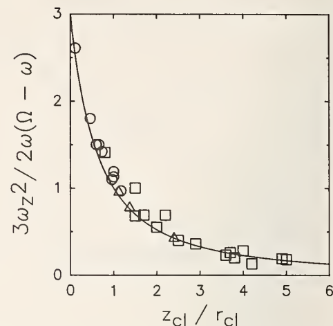
FIG. 12. Relationship between the plasma rotation frequency and the plasma aspect ratio is shown. The quantity 3\omega_z^2/[2\omega(\Omega - \omega)] is calculated from the measured values of \omega , \omega_z , and \Omega and plotted vs the measured aspect ratio z_{cl}/r_{cl} . The solid, theoretical curve is determined from Eqs. (14)–(16) and is independent of the trap voltage and magnetic field. Data were obtained for {}^9\text{Be}^+ plasmas with 2000 to 40 000 {}^9\text{Be}^+ ions. Three different sets of data from two different traps are plotted. The first set (○) was taken in trap I with 2 V trap voltage ( \omega_z/2\pi = 290 kHz). The second set (□) was taken at a trap voltage of 1.5 V ( \omega_z/2\pi = 212 kHz) on trap II. The third set (△) was taken at trap voltages of 0.9 V ( \omega_z/2\pi = 170 kHz) and 1.5 V on trap II. All data were taken at a magnetic field of 1.4 T.
