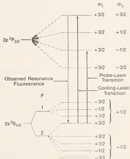
FIG. 2. Hyperfine structure of {}^9\text{Be}^+ in a magnetic field, showing the transitions pertinent to the analysis of the experiment. The cooling transition is from the 2s\,{}^2S_{1/2}(m_I, m_J) = (+\frac{3}{2}, +\frac{1}{2}) state to the 2p\,{}^2P_{3/2}(+\frac{3}{2}, +\frac{3}{2}) state. The probe depopulation transition is from the 2s\,{}^2S_{1/2}(+\frac{3}{2}, +\frac{1}{2}) state to the 2p\,{}^2P_{3/2}(+\frac{3}{2}, -\frac{1}{2}) state. The figure is not drawn to scale. The frequency splittings between the 2s\,{}^2S_{1/2}|\Delta m_I| = 1, |\Delta m_J| = 0 states are on the order of 300 MHz. Only the 2p\,{}^2P_{3/2}, m_I = +\frac{3}{2} states are shown because the frequency splittings between the 2p\,{}^2P_{3/2}|\Delta m_I| = 1, |\Delta m_J| = 0 states are on the order of 1 MHz.
