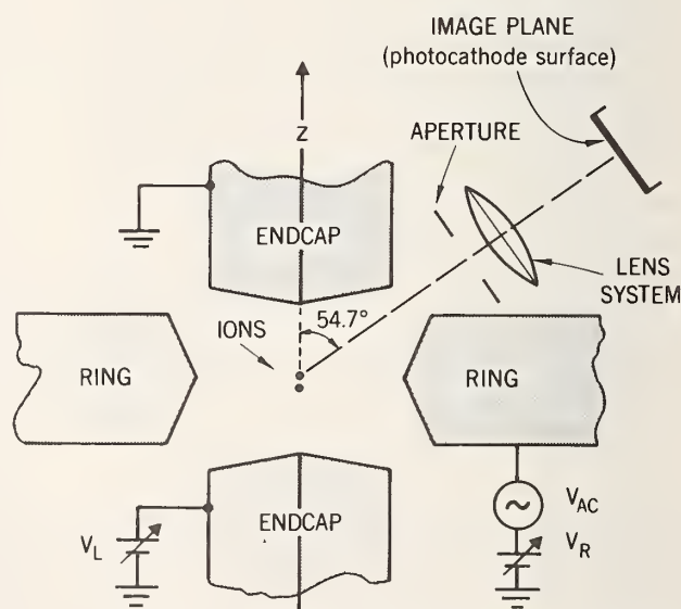
FIG. 1. Schematic drawing of the trap electrodes (to scale) and imaging system (not to scale). The end-cap to end-cap separation along the z axis is approximately 625 \mu\text{m} . The overall magnification of the lens system is 60\times . The laser beam used to illuminate the ions also enters the trap at an angle of 54.7^\circ with respect to the z axis and is perpendicular to the observation axis shown.
