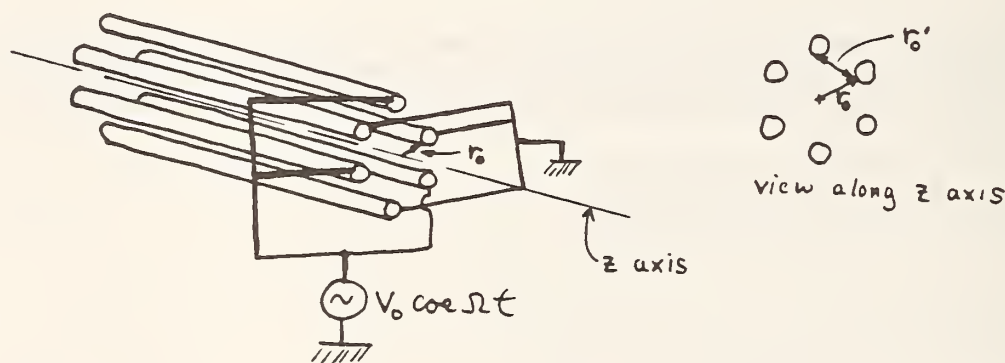
Fig. 4. Sketch of cylinder rf-type trap for k = 2 .
