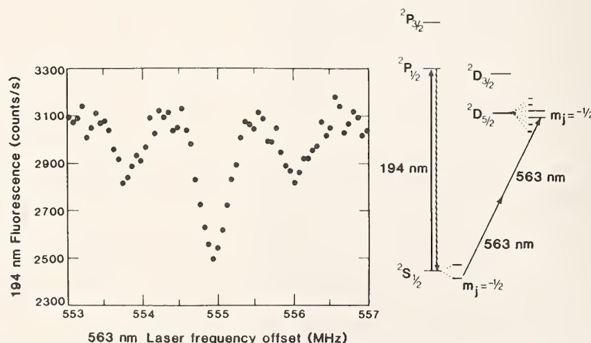
FIG. 2. Two-photon ^2S_{1/2} \rightarrow ^2D_{5/2} transition in ^{198}\text{Hg}^+ . Amplitude modulation by the harmonic secular motion of the ions is visible in this scan. The frequency scan is 4 MHz at the fundamental laser frequency ( \lambda \cong 563\text{ nm} ). The depth of the central component is about 25% of full scale. The integration time is 2 s/point. In the inset is a simplified energy-level diagram of ^{198}\text{Hg}^+ , depicting the levels of interest.
