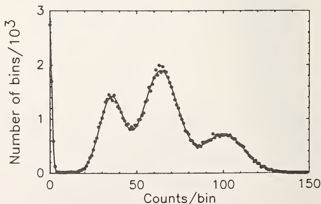
Fig. 6. Fluorescence intensity distribution for three \text{Hg}^+ ions (dots) and a least-squares fit (solid curve).
