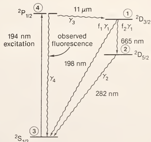
FIG. 1. Diagram of the lowest four energy levels of \text{Hg}^+ . Only the 194\text{-nm} fluorescence was observed directly.
