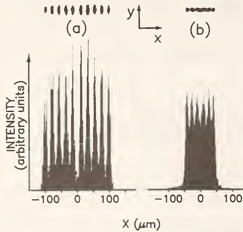
FIG. 3. Intensity plots along the imager x axis (parallel to the probe beam) through the center of the ion cloud with corresponding images (above). (a) \Gamma = 180 \pm 90 ( T = 6 \pm 4 mK, n_0 \approx 7 \times 10^7 ions \text{cm}^{-3} ). Cloud aspect ratio a_r \approx 3.5 . (b) \Gamma = 50 \pm 30 ( T = 33 \pm 13 mK, n_0 = 2 \times 10^8 ions \text{cm}^{-3} ), a_r \approx 5 . The clouds contained about 1000 ions in both cases.
