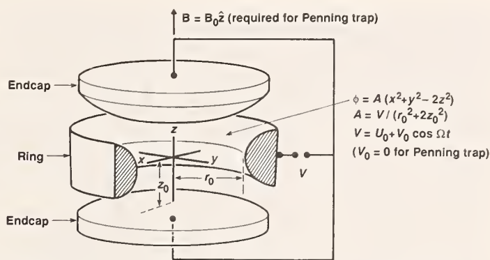
Fig. 1. Electrodes for a Penning or rf ion trap. The electric potential \phi is created by applying the voltage V between the endcap electrodes and the ring electrode. The uniform magnetic field B is required only for a Penning trap. [Adapted from (42) with permission from Plenum Press]
