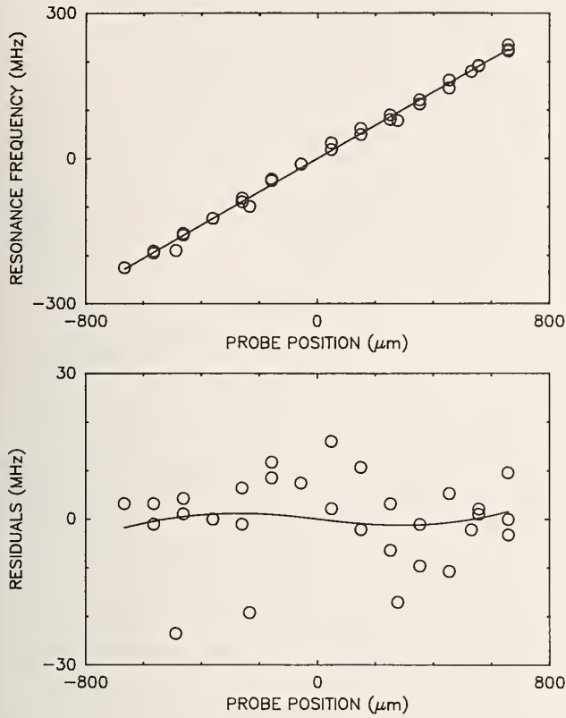
FIG. 9. A plot similar to Fig. 7. The {}^9\text{Be}^+ resonance frequency \nu'_0 is plotted vs d for a plasma of 25 000 {}^9\text{Be}^+ ions (density of 1.7 \times 10^7 ions/cm 3 ) stored simultaneously with {}^{198}\text{Hg}^+ ions. The result of the fit is \xi = 0.06 \pm 0.1 . The data were taken at a magnetic field of 1.4 T and a trap axial frequency of \omega_z/2\pi = 212 kHz.
