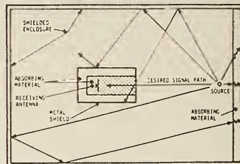
Fig. 2. Diagram of a hooded-antenna measurement setup in a shielded enclosure.
