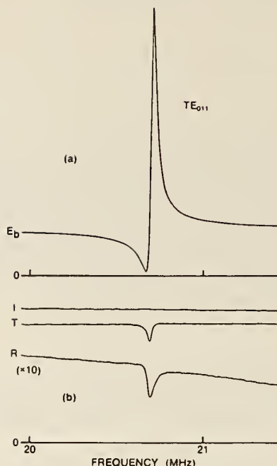
Figure 1 Detection of the TE_{011} resonance at 20.70 MHz by swept-frequency measurements. (a) Electric field ( E_b ) at position B1. (Field components and positions are defined in Fig. 3 and the text). (b) Incident (I), transmitted (T), and reflected (R) power. Ordinate scales are linear in (a) electric field, or (b) power, but otherwise arbitrary.
