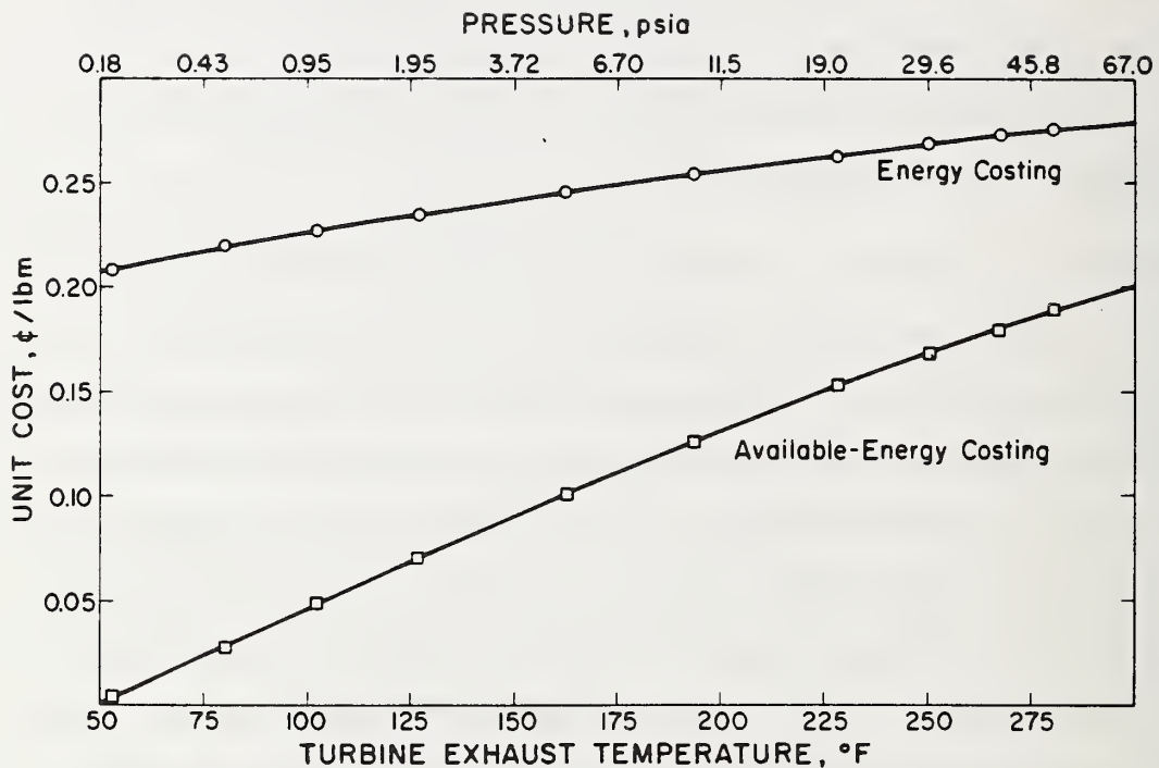
Figure 1. Cost of Cogenerated Steam (as presented in reference [14])
