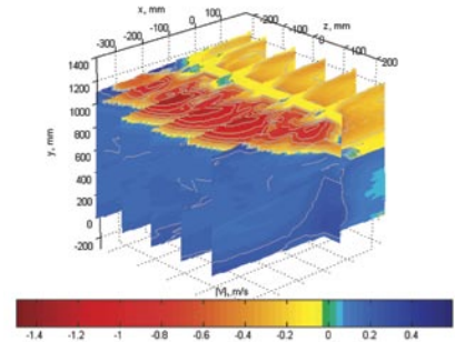
Volumetric mapping of SPIV measurements in the reduced-scale fluid flow analog experiment (inflow in blue, outflow in red).
