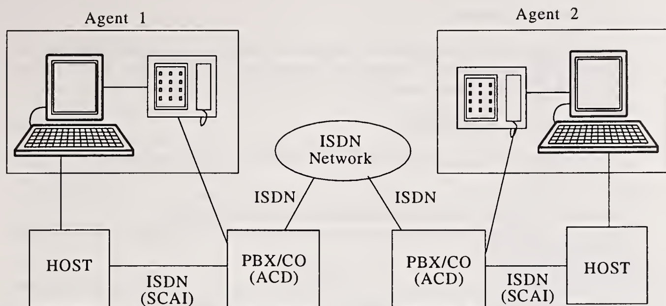
Figure 7-9. Call Transfer with Data Service Element Switch Host Interface — Network Signalling Requirements.
