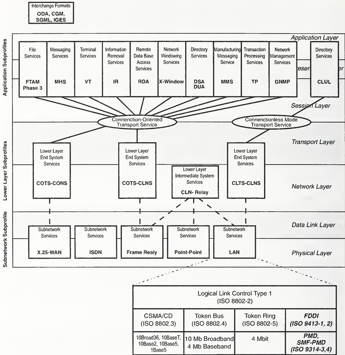
Figure 25 - IGOS Subprofiles and FDDI.
