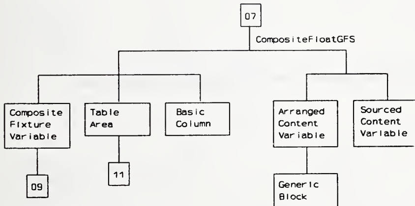
Figure 41 — CompositeFloat
