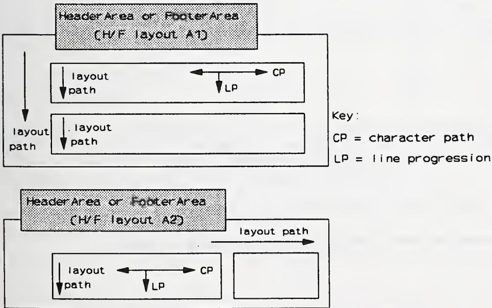
Figure 2 — Header and footer frame layouts corresponding to Figure 1
