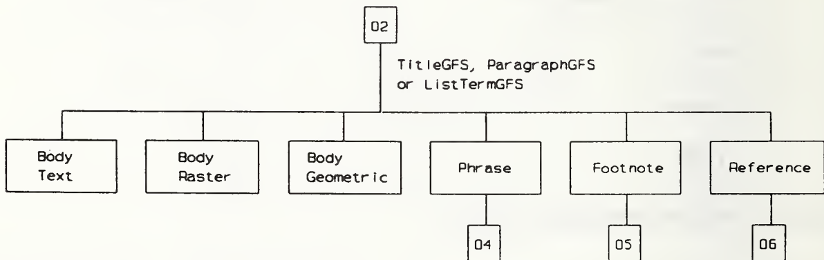
Figure 23 — Title, Paragraph and ListTerm
