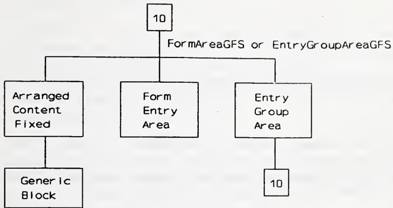
Figure 44 — FormArea and EntryGroup
