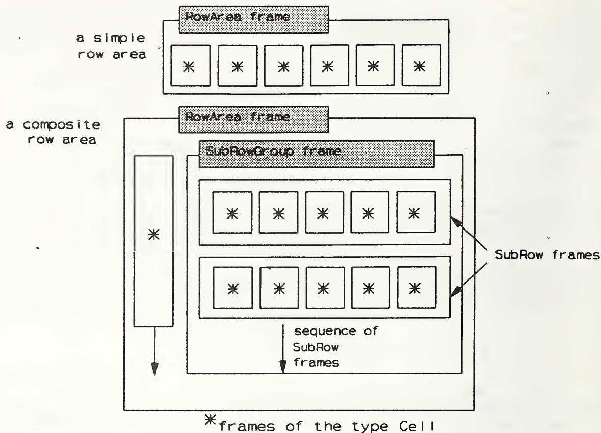
Figure 17 — Frames used to represent table rows
