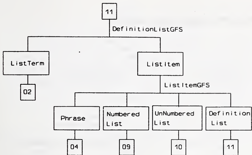
Figure 32 — DefinitionList
