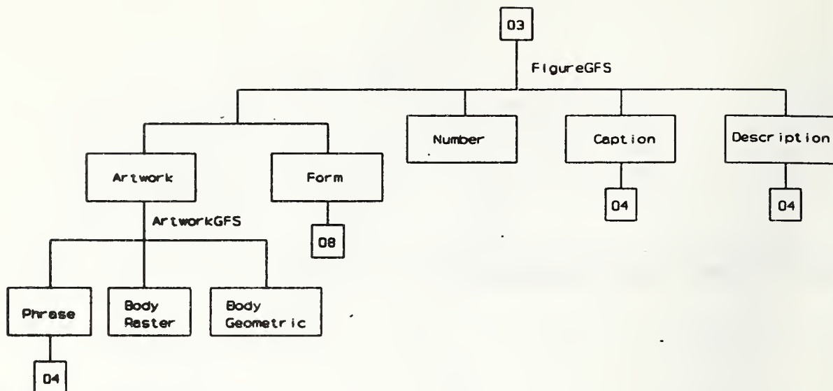
Figure 26 — Figure
