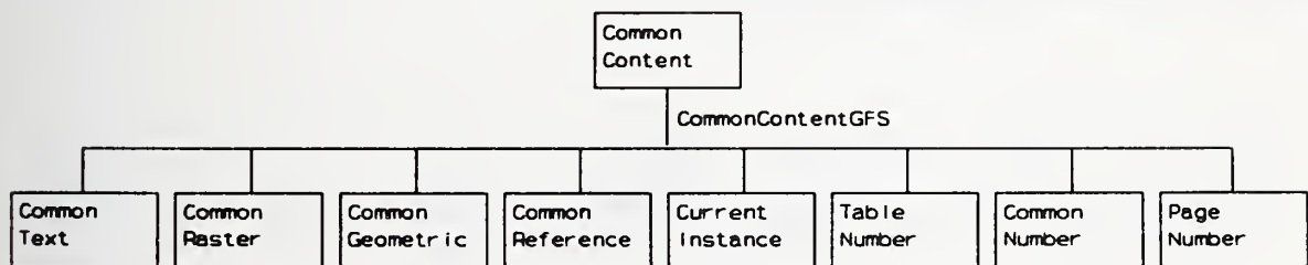
Figure 33 — CommonContent
