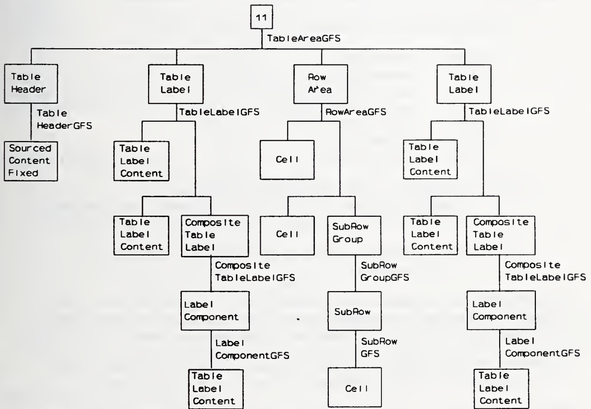
Figure 45 — TableArea
