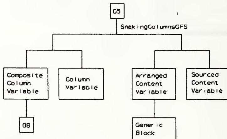
Figure 39 — SnakingColumns
