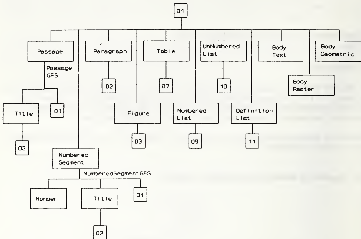
Figure 22 — DocumentLogicalRoot, 2nd level
