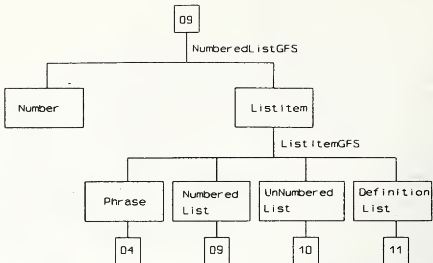
Figure 30 — NumberedList
