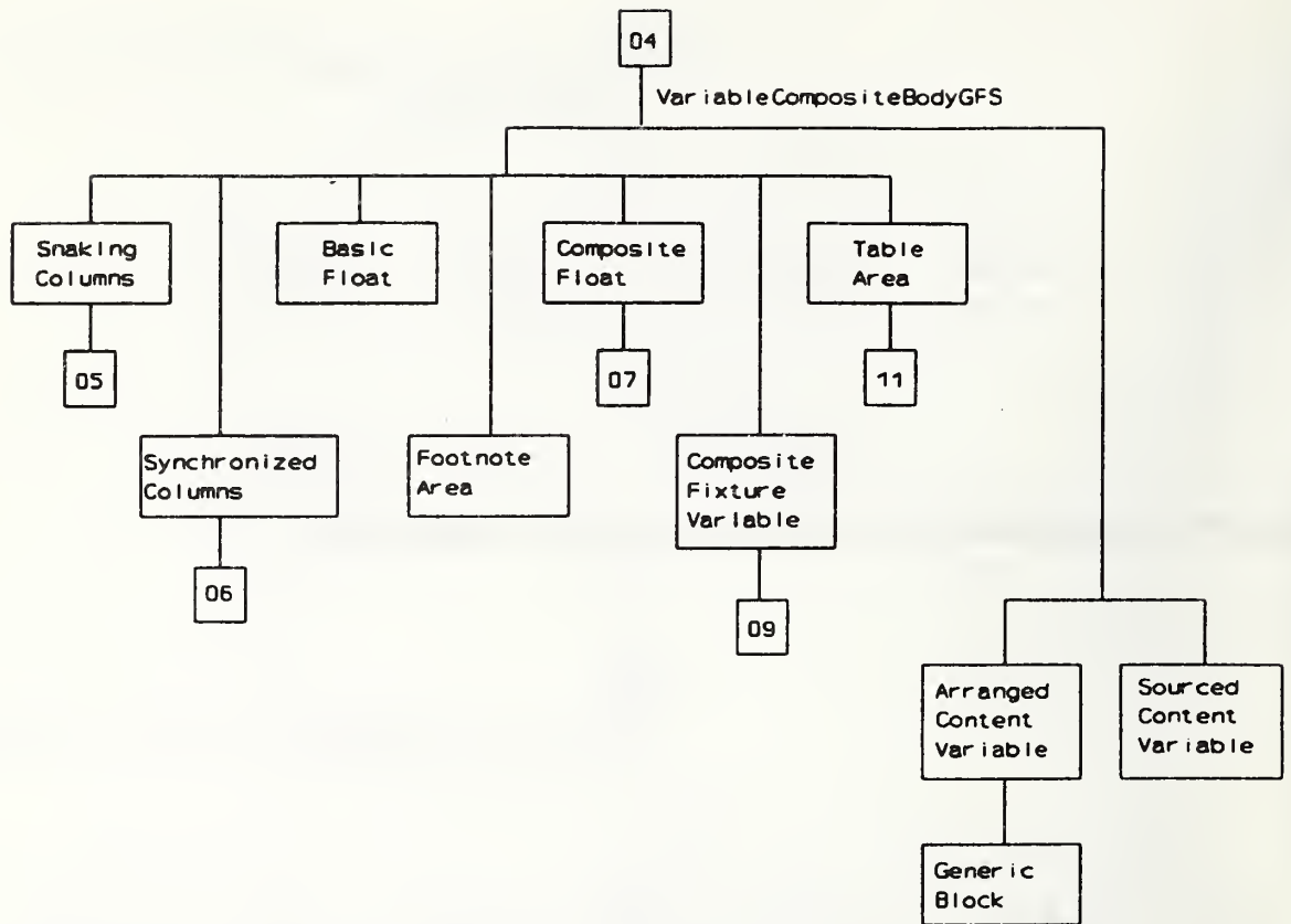
Figure 38 — VariableCompositeBody
