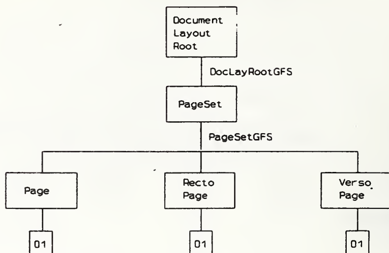
Figure 34 — DocumentLayoutRoot
