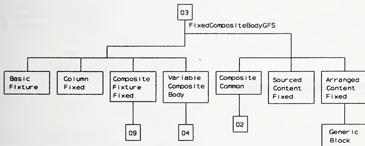
Figure 37 — FixedCompositeBody
