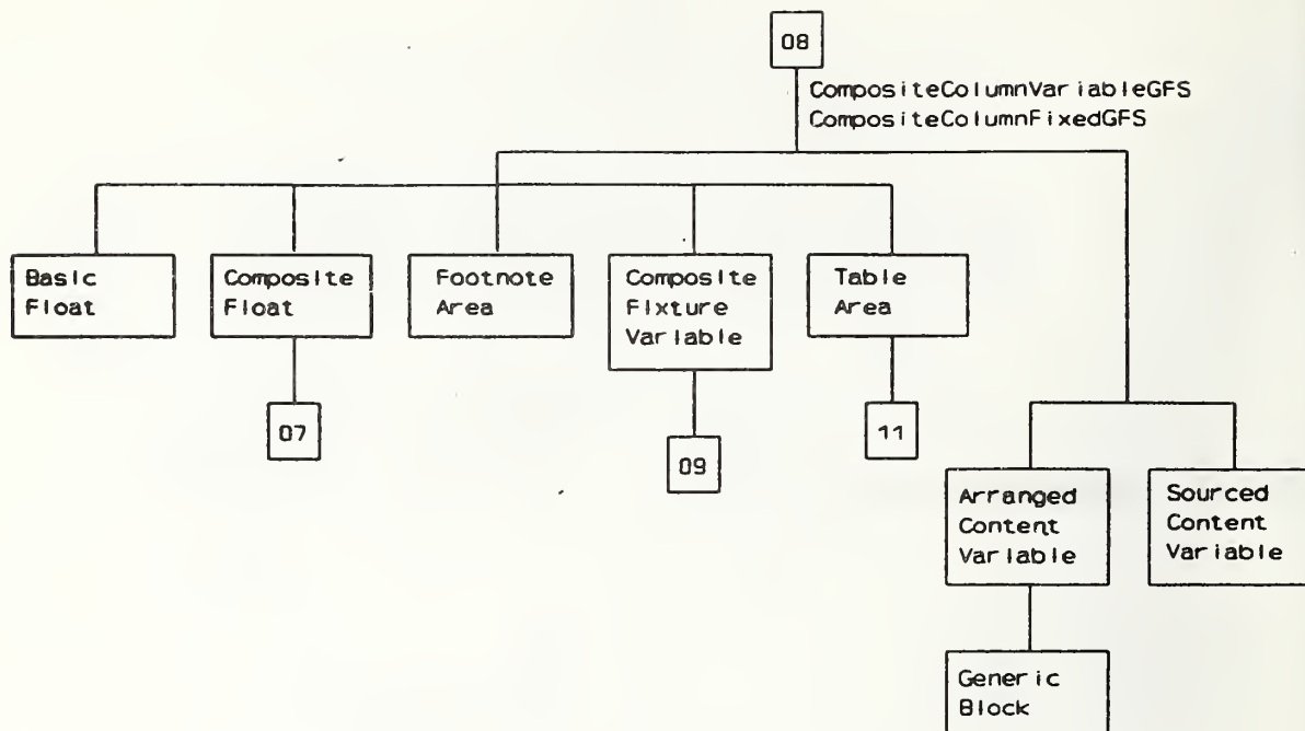
Figure 42 — CompositeColumnVariable and CompositeColumnFixed
