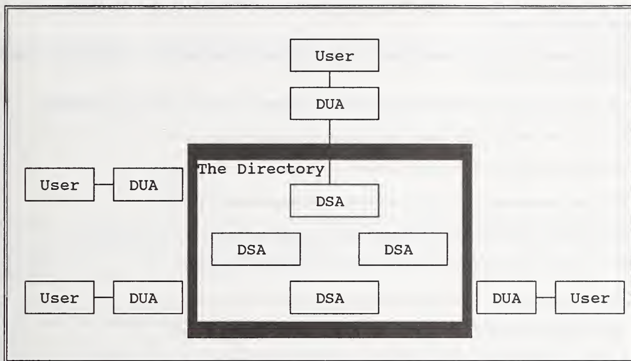
Figure 3 - Distributed directory model
