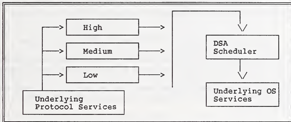
Figure 4 - Logical DSA application environment
