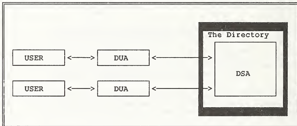
Figure 2 - Centralized directory model
