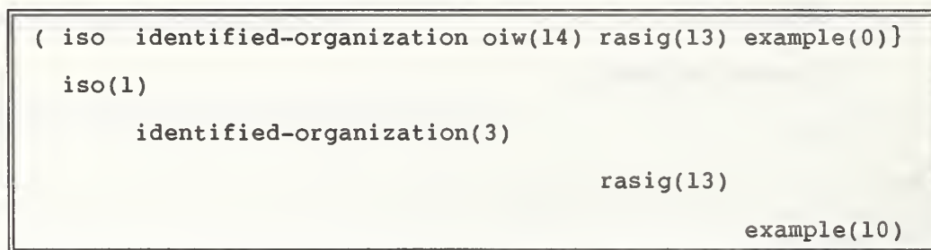
Figure 2 - Structure of an Object Identifier for an Example Object for the Registration Authority SIG of OIW.
