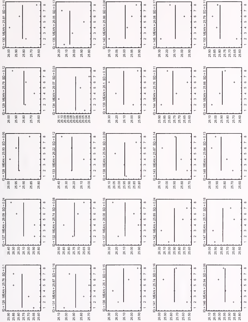
Figure 8 (3b). Panel ID=126-150: Thickness measurements (in millimeters) at locations 1 through 8 (Fig. 3b) for insulation panels 126 through 150. Mean is shown as solid line (with numerical values for mean and standard deviation (SD) in the title of each frame).
