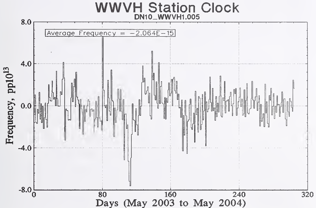
Figure 5.5. Daily frequency offset estimates for WWVH station clock.
