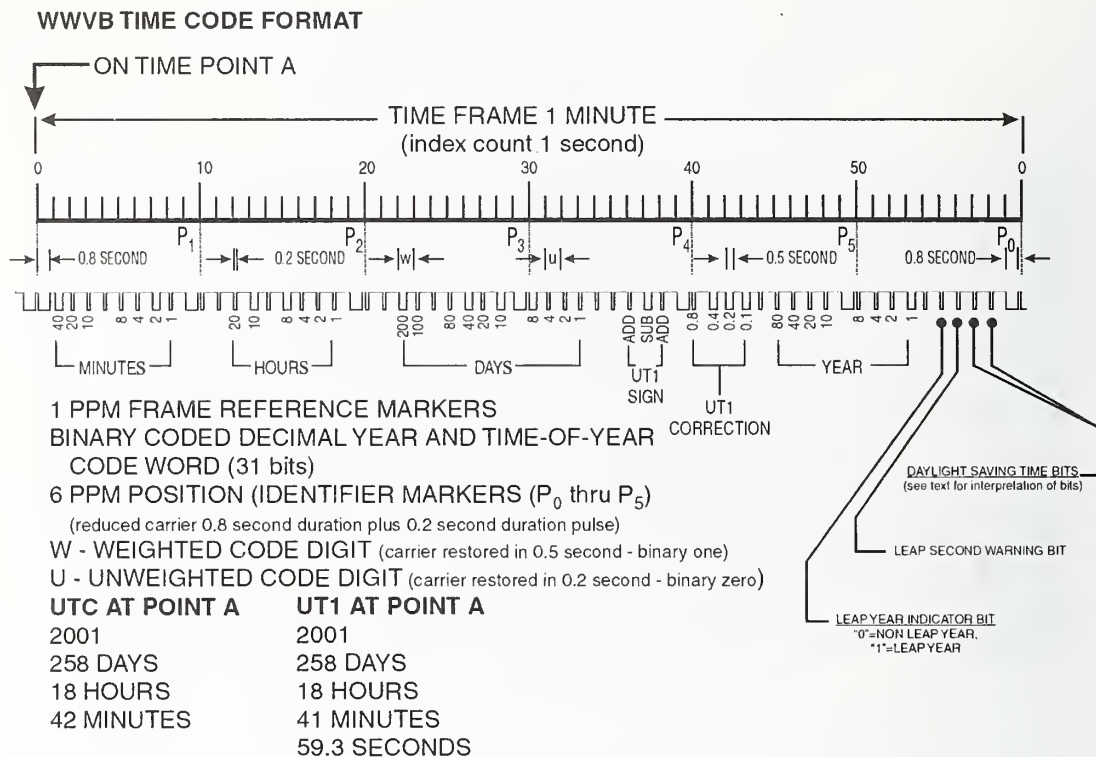
Figure 2.15. WWVB time code format.
