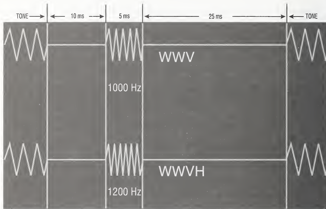
Figure 2.6. WWV and WWVH second pulses.
