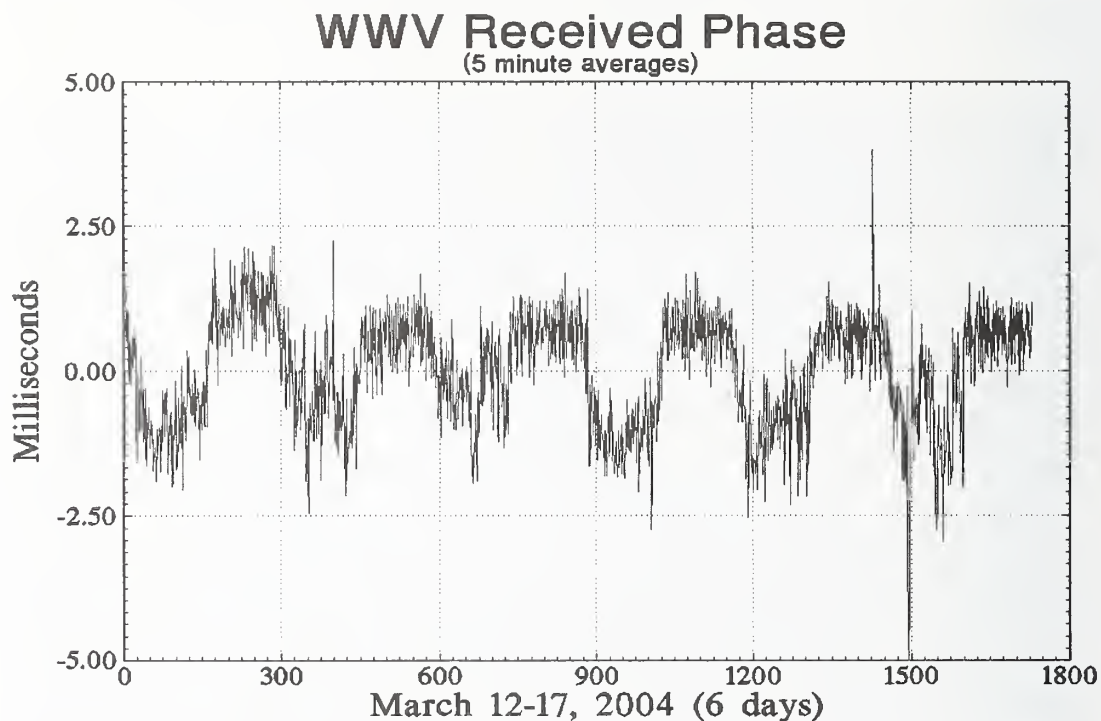
Figure 5.11. WWV phase comparison using 1 pps output from commercial timing receiver.
