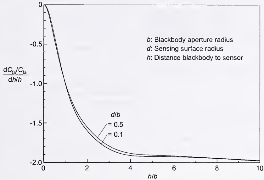
Figure 6. Incremental change in configuration factor with distance [8]
