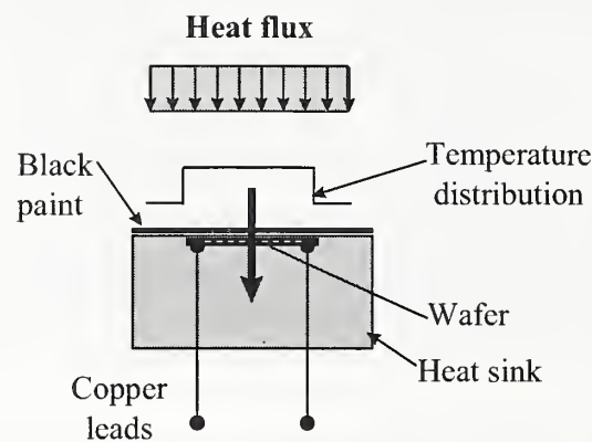
Figure 4. Schematic representation of a Schmidt-Boelter sensor
