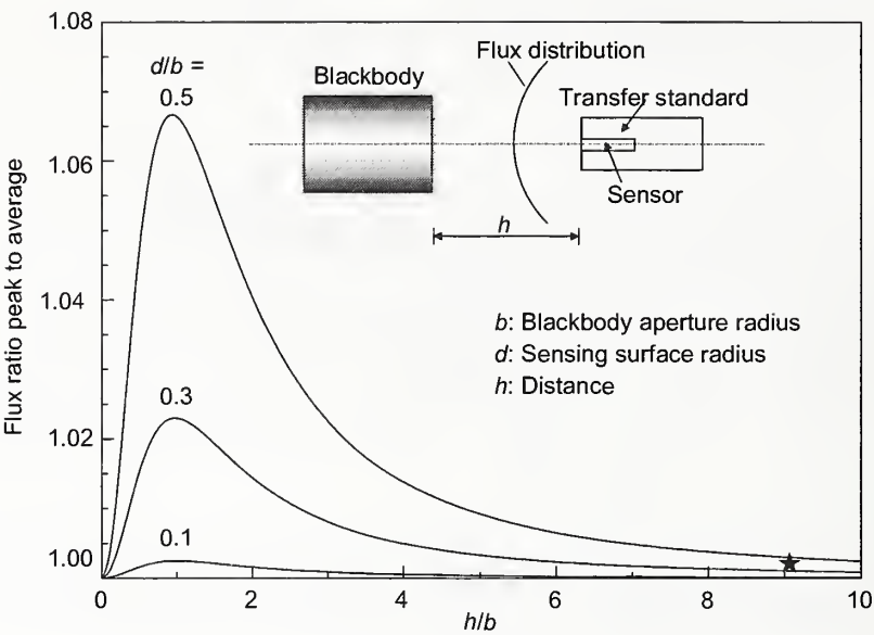
Figure 7. Ratio of peak to average irradiance at sensor location [8]
