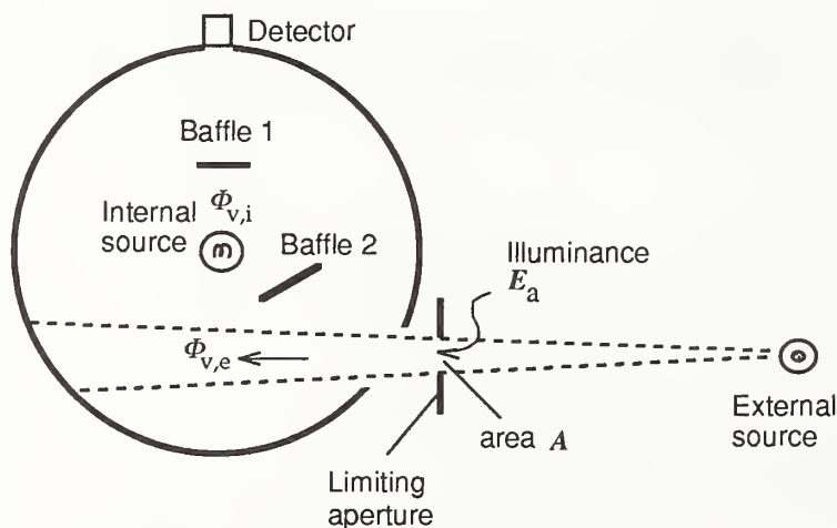
Figure 17 Geometry of the simulation model.
