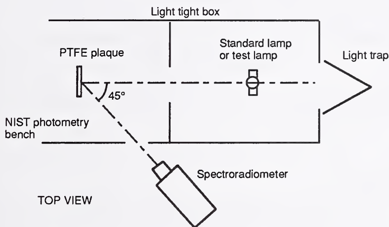
Figure 28 Configuration for color temperature calibration.
