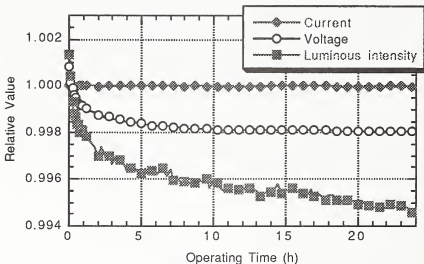
Figure 11 Aging characteristics of a typical Airway Beacon type lamp at 2856 K.
