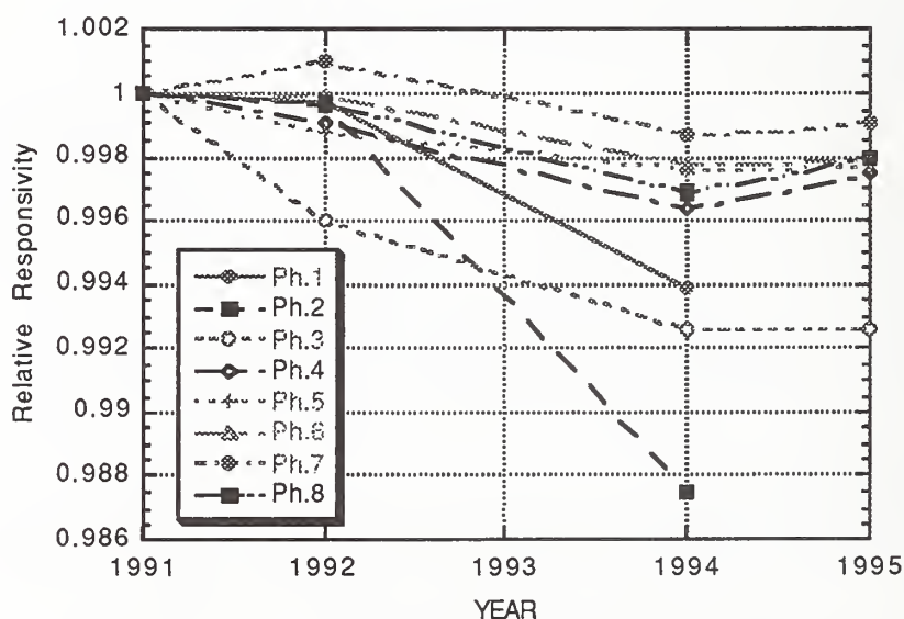
Figure 9 Drift of the illuminance responsivity of the NIST standard photometers over a 4 year period.
