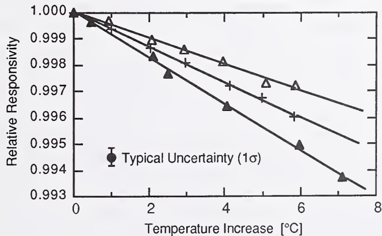
Figure 7 The temperature dependence of the photometers' illuminance responsivity.
