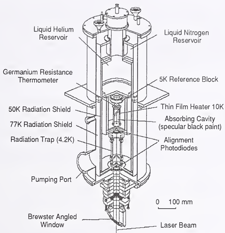
Figure 3 Construction of the High Accuracy Cryogenic Radiometer.
