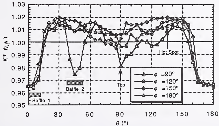
Figure 19 SRDF of the NIST integrating sphere. ( \theta = 0 is at the detector. \phi = 0 is the plane passing through the sphere bottom.)
