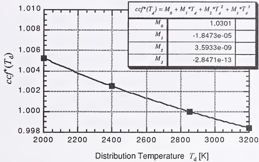
Figure 6 Polynomial fit for the spectral mismatch correction factors.
