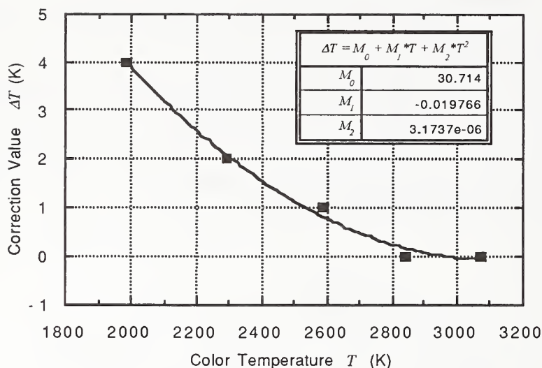
Figure 29 Color temperature correction values for the NIST diode-array spectroradiometer.
