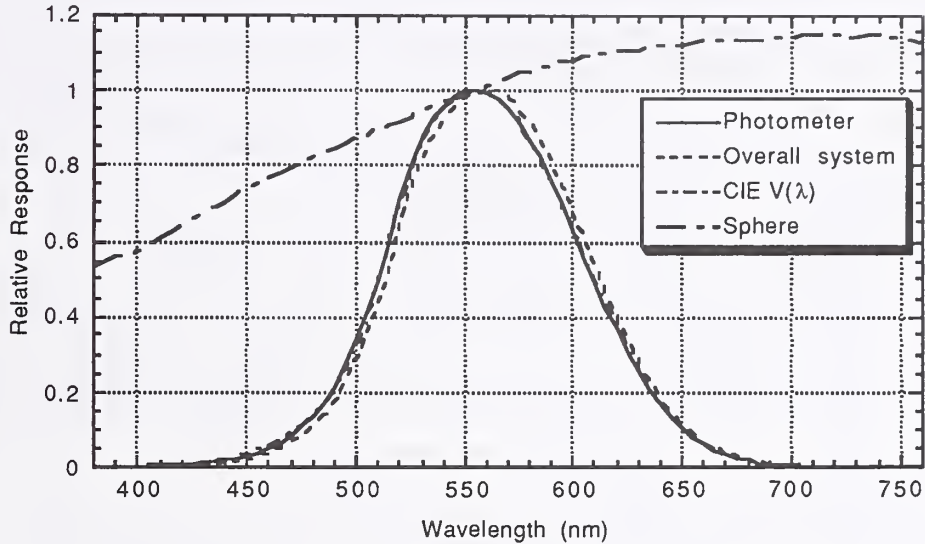
Figure 21 Spectral characteristics of the NIST integrating sphere.
