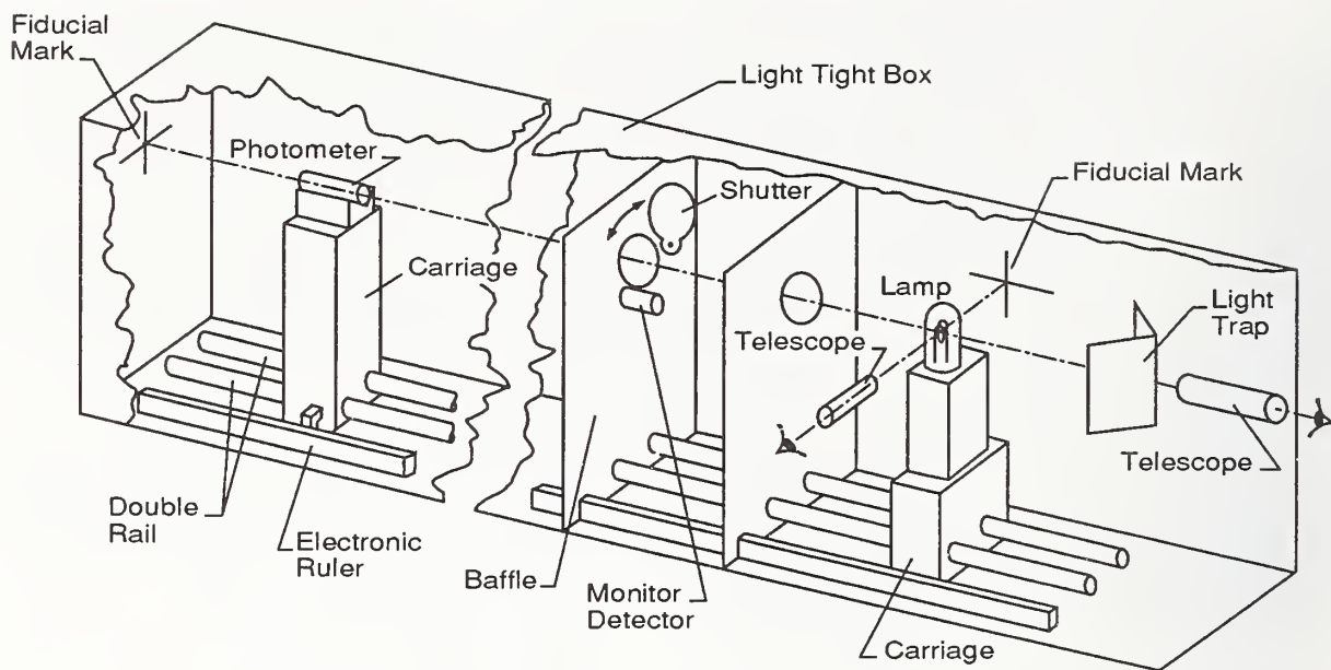
Figure 16 NIST Photometry Bench.
