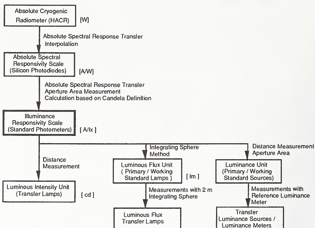
Figure 2 Realization and maintenance of the NIST photometric units.
