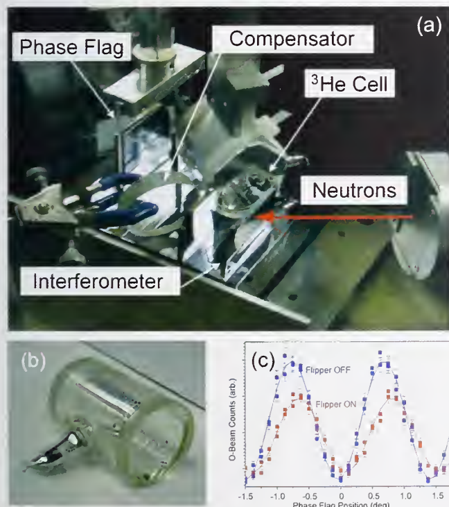
FIGURE 2: Experimental setup. (a) Neutrons enter from the right of the picture. One can see the compensation glass, the target cell, and the quartz phase flag. (b) One of the target cells used. Solid rubidium which is heated and used in Spin-Exchange Optical Pumping can be seen in the picture as dark spots along the cell walls. (c) A typical interferogram. The blue curve (lines are fits) is the O-beam intensity for when the neutron and ^3\text{He} spins are aligned parallel. The red curve is for when the neutron spin has undergone a spin flip. Lower intensity in the red curve is due to increased neutron absorption in that case. A phase shift around 30^\circ can be seen by comparing the two curves.
