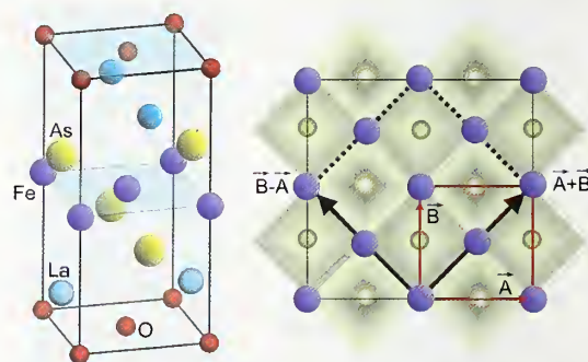
FIGURE 1: The crystal structure of LaOFeAs (left) and the top view of the FeAs-plane and the relations between primitive and \sqrt{2} \times \sqrt{2} -supercell used in our calculations. The dark and light shaded areas indicate the As atoms below and above the Fe-square lattice, respectively.
