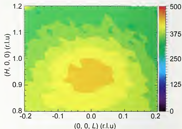
FIGURE 1: Neutron scattering intensity map measured at 300 K on a furnace-cooled single crystal of \text{Fe}_{0.81}\text{Ga}_{0.19} . The symmetry of the underlying matrix allows no \{1,0,0\} reflection. The broad diffuse scattering that peaks near (0.95, 0, 0) thus indicates the presence of a short-range ordered structure having a different symmetry and lattice spacing.
