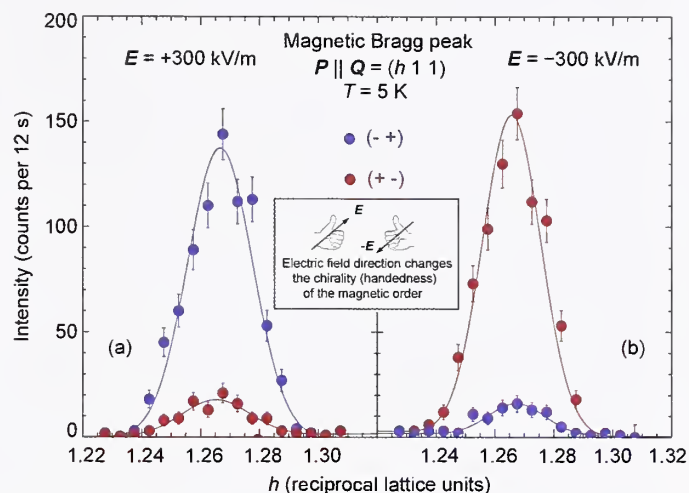
FIGURE 2: Full polarized neutron magnetic diffraction. The neutron polarization P is parallel to Q , [P||Q] , so that all the magnetic scattering is spin-flip. (a) A +300 kV/m electric field selects one chiral domain, and then the magnetic peak is only observed in the (- +) configuration; the small peak in the (+ -) configuration is due to the imperfect instrumental polarization. (b) With the ferroelectric polarization reversed by applying -300 kV/m, the magnetic Bragg peak is only observed in the (+ -) configuration.
