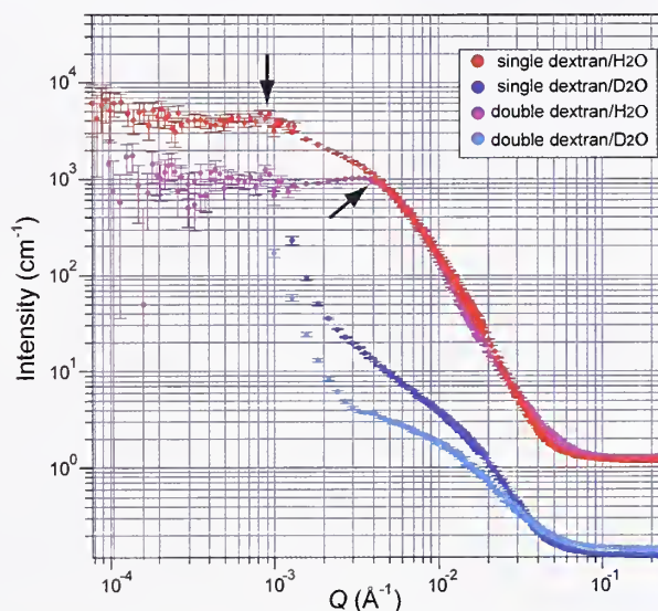
FIGURE 3: SANS/USANS data showing the interaction peak in the double dextran sample with a concentration of 25.6 \text{ mg/ml} at Q = 4 \times 10^{-3} \text{ Å}^{-1} (radius = 157 \text{ nm} ), and the possible interaction peak in the single dextran layer sample with a concentration of 21.8 \text{ mg/ml} at Q = 9 \times 10^{-4} \text{ Å}^{-1} (radius = 698 \text{ nm} ).
