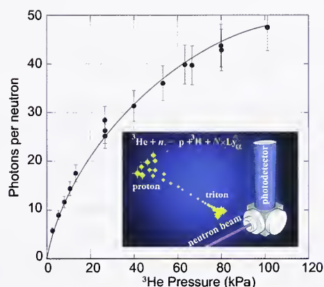
FIGURE 1: Lyman alpha photon yield per reacted neutron as a function of ^3\text{He} pressure. The inset states the nuclear reaction and the cartoon indicates photon production and the experimental setup.
