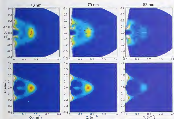
FIGURE 2: Rotational SANS reciprocal-space reconstructions for three different film thicknesses (top row) show varying intensity of the vertical peak. The associated best-fit models (bottom row) provide insight into the angular distribution of the lamellae.
