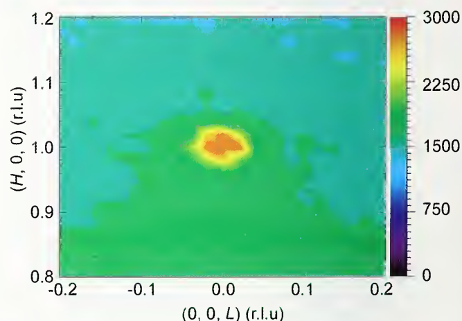
FIGURE 2: Neutron scattering intensity map measured at 300 K on a slow-cooled single crystal of \text{Fe}_{0.81}\text{Ga}_{0.19} . Under slow-cooled conditions, \text{Fe}_{0.81}\text{Ga}_{0.19} exhibits a long-range ordered structure with DO_3 symmetry, for which a \{1,0,0\} reflection is allowed. The diffuse scattering observed in the quenched crystal is absent. The diffuse scattering located below the line H = 1 and shown in green is believed to be size-effect scattering.
