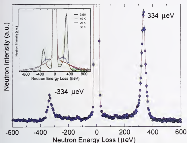
FIGURE 2: ZIF8 tunneling spectrum at 1.4 K using the DCS spectrometer with 7 Å neutrons ( \approx 18 \text{ } \mu\text{eV} resolution). (inset) Evolution of the tunneling spectrum with temperature using the FCS spectrometer with 6 Å neutrons ( \approx 70 \text{ } \mu\text{eV} resolution).
