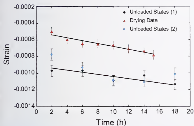
FIGURE 2: Comparison of strains from a drying test with the strains of the unloaded states. The measured \text{Ca}(\text{OH})_2 lattice strains characterize the behavior of a minority constituent; the behavior of the cement paste aggregate as a whole is better captured with surface attached strain gages. The comparison of suitably normalized lattice strains and macroscopic strains is shown in Fig. 3.
