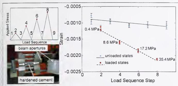
FIGURE 1: Compressive tests of cement paste prisms (10 mm \times 10 mm \times 15 mm) in loading-unloading cycles. The strain follows the applied load in linear dependence. However, with increasing time and water evaporation the strains in the unloaded states (0.43 MPa) become more compressive. A subsequent drying measurement of an unloaded sample during water evaporation revealed that the strains in the unloaded states exhibit a similar rate as the shrinkage strains originating from dehydration/evaporation only (Fig.2).
