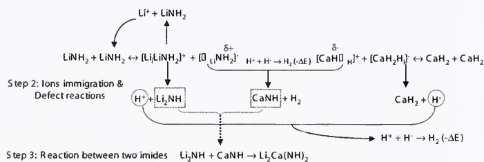
Scheme 1: Dehydrogenation of 2\text{LiNH}_2 + \text{CaH}_2 with a total of 2\text{H}_2 released and products of \text{CaNH} , \text{Li}_2\text{NH} and/or \text{Li}_2\text{Ca}(\text{NH})_2 observed at various desorption steps.
