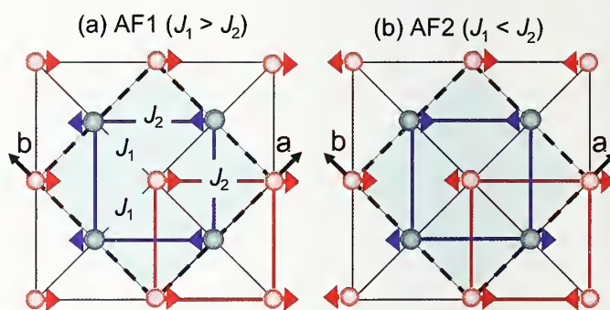
FIGURE 2: Two antiferromagnetic configurations considered in this study.
