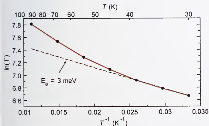
FIGURE 3: A plot of \ln(I) vs. T^{-1} for ZIF8 between 30 K and 90 K, where I (in \mu\text{eV} ) is the full-width-at-half-maximum quasielastic linewidth.
