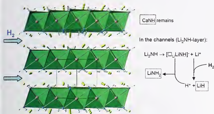
FIGURE 2: Structure of \text{Li}_2\text{Ca}(\text{NH})_2 viewed as an "intercalated" layered structure consisting of 2D slabs of \text{Ca}[\text{NH}]_6 -octahedra separated by Li ion motifs. Ca, Li, N and H atoms are colored as in Fig. 1. The facile motion of Li assists the hydrogenation process with totally 1 \text{H}_2 absorbed and final products of \text{CaNH} , \text{LiNH}_2 and \text{LiH} .
