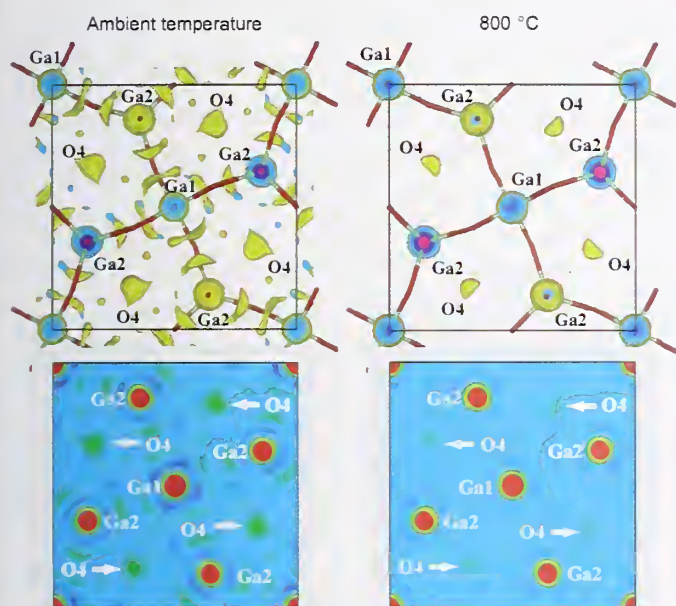
FIGURE 2: Comparison of the nuclear scattering density of \text{La}_{1.54}\text{Sr}_{0.46}\text{Ga}_3\text{O}_{7.27} as obtained from maximum entropy analysis maps. The [001]_c projections (top) and corresponding scattering density at z = 0 (below) are shown at ambient (left) and 800 °C (right).
