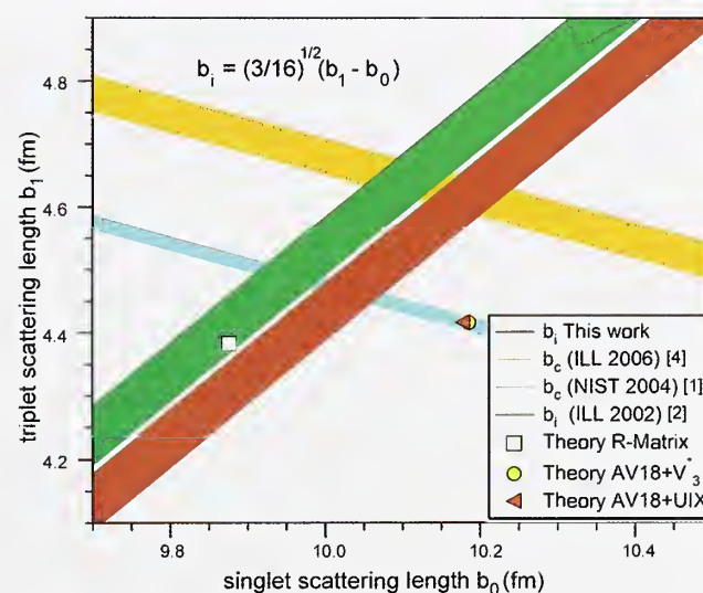
FIGURE 3: Experimental results found in [1], [2], and [4] compared with predicted values of some NN+3NI theoretical models [5]. The coherent scattering length measured in Refs. 1 and 4 is given by b_c = \frac{3}{4} b_1 + \frac{1}{4} b_0 . The results are shown as bands representing the result \pm one standard deviation, \sigma .
