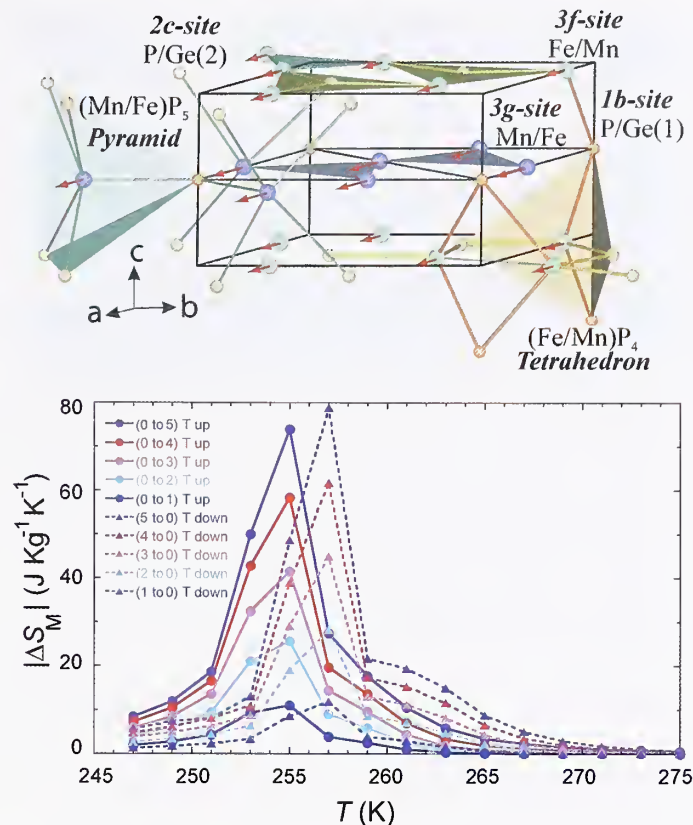
FIGURE 2: The Magnetocaloric Effect. Temperature dependence of the entropy change of the bulk \text{Mn}_{1.1}\text{Fe}_{0.9}\text{P}_{0.8}\text{Ge}_{0.2} compound as a function of applied magnetic field up to 5 T. The upper panel shows the crystal structure for the FM-phase which differs from that in the PM-phase in the ordering of the spins and the lengths of a , b , and c .
