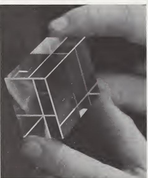
Thomas Proctor determined the velocity of sound in this borosilicate block by measuring the time required for a sound pulse to cross the block and be reflected back to a transducer opposed to one of the faces.
