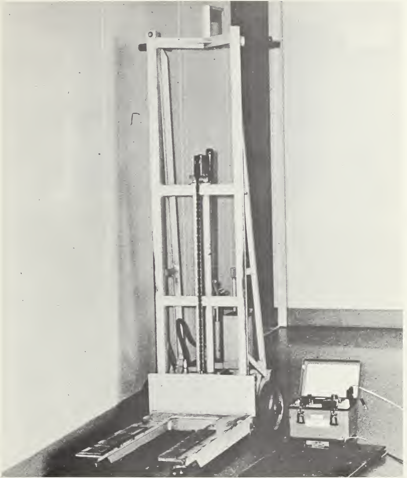
FIG. 5 FORKLIFT ACTUATED THROUGH HYDRAULIC PUMP SYSTEMS.
