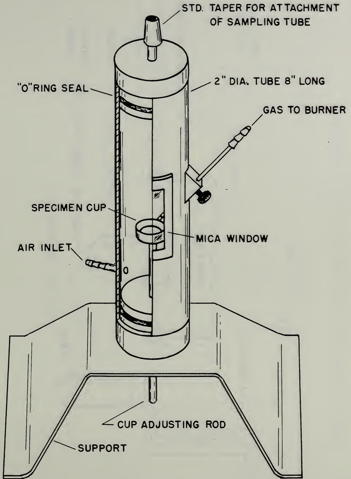
FIG. I- ENCLOSED BURNER
