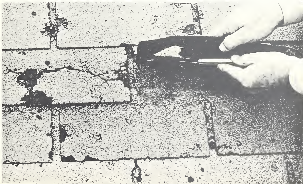
Figure 34. Hail damage where reroofing is mandatory.
