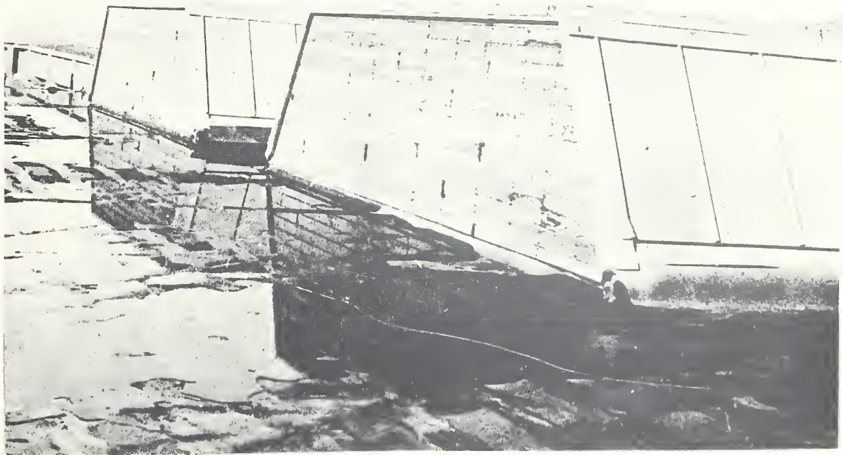
Figure 8. Wide selvage roll roofing on practically flat roof.
