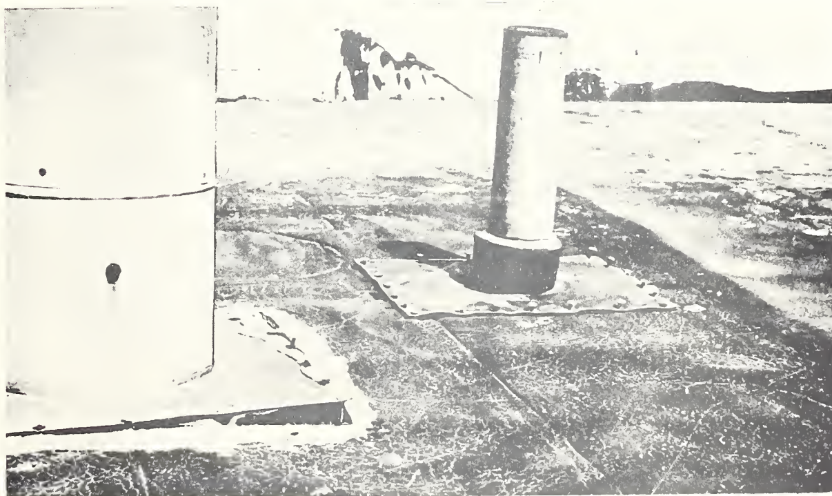
Figure 43. Separation of metal flashing flange from roof caused by exposed nails working loose.
