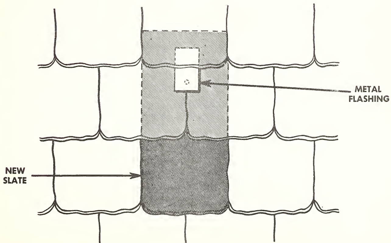
Figure 41. Method for inserting new slate.
