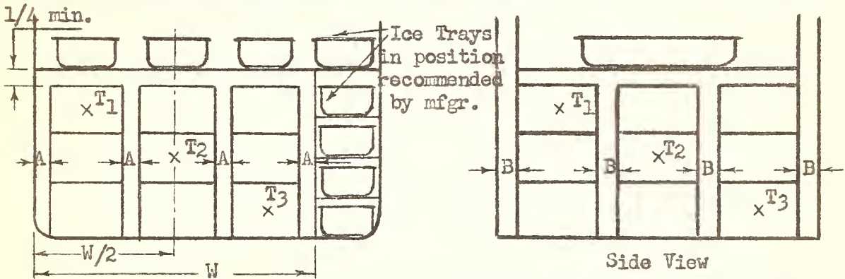
VERTICAL FROZEN FOOD STORAGE COMPARTMENT (Width greater than 8 inches)
