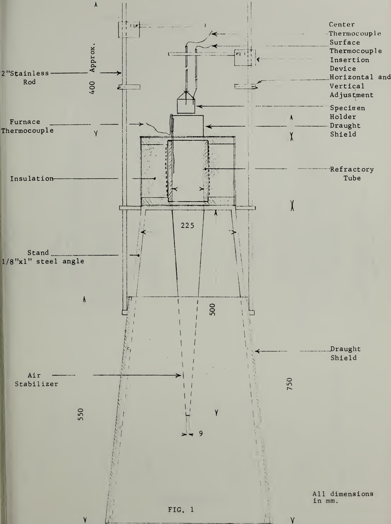
General Arrangement - Non-combustibility Apparatus
