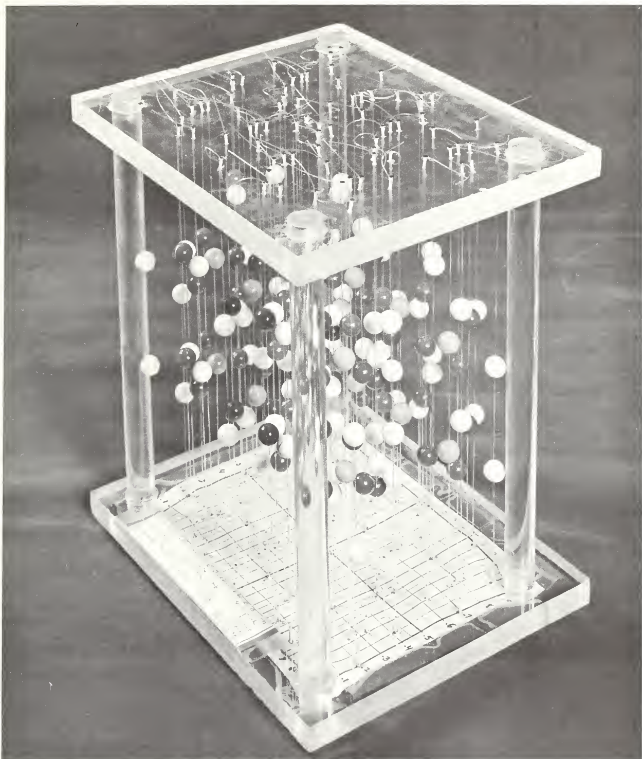
Figure 1 A Model of the Crystal Structure of \text{Na}_2\text{CO}_3 \cdot \text{H}_2\text{O}
