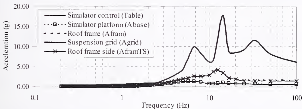
b) horizontal response spectra
