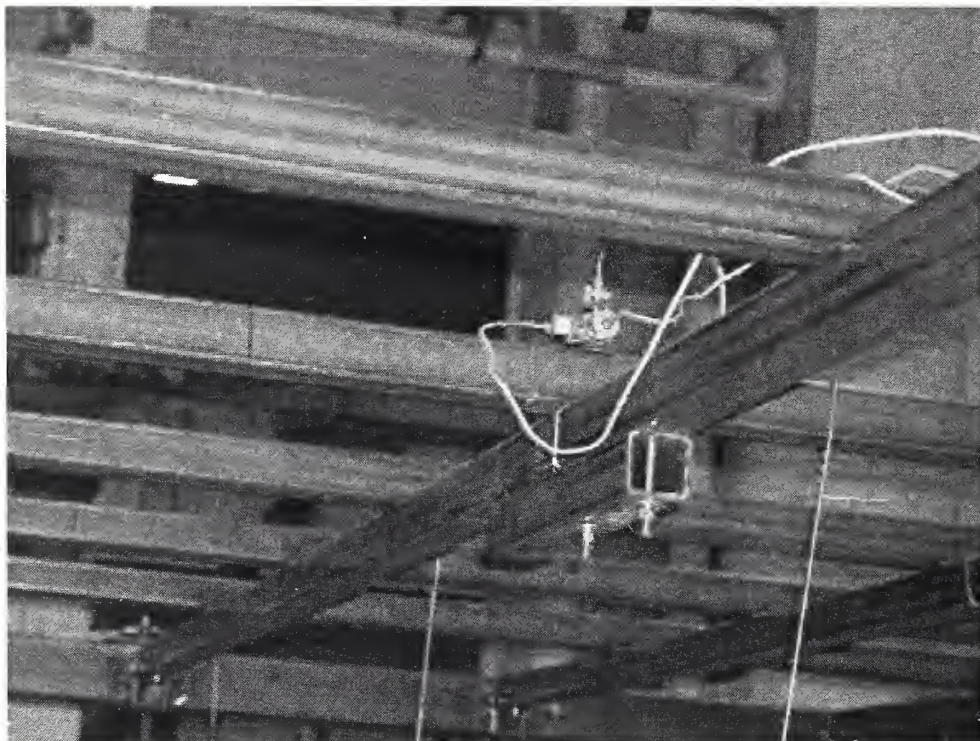
Figure 2–12a. Accelerometers monitoring the response of the test assembly in the center at the top of the test frame.
