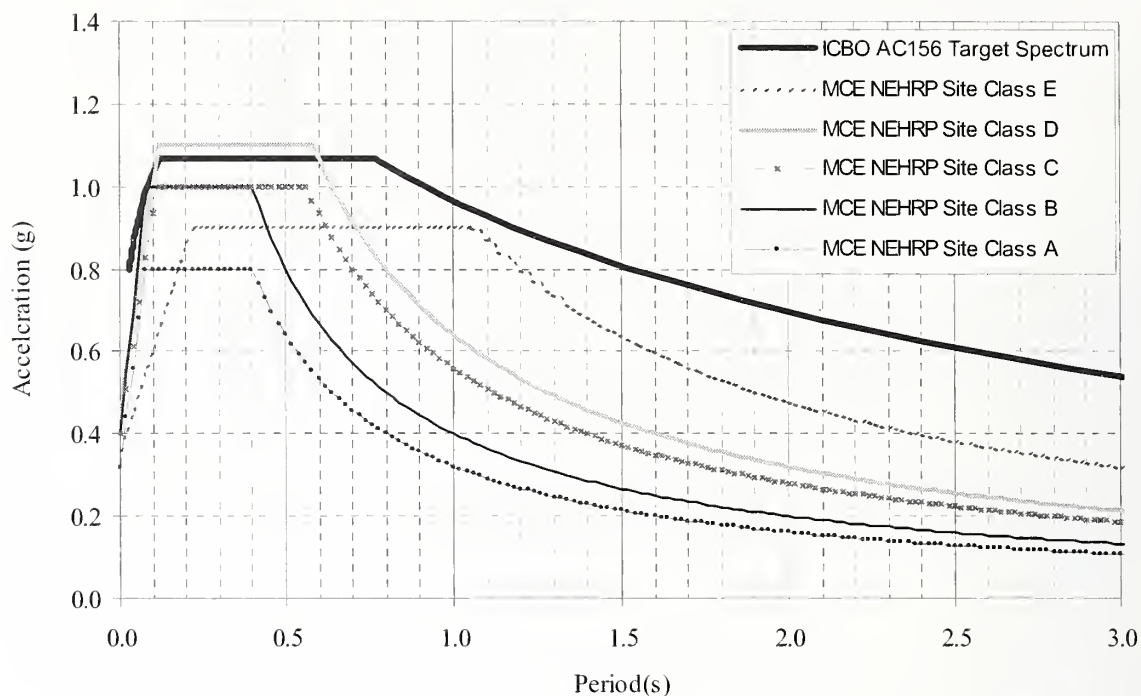
Figure 2-53. Relationship between MCE NEHRP spectra and target qualification spectrum ( S_S=1.0g , S_I=0.4g ).
