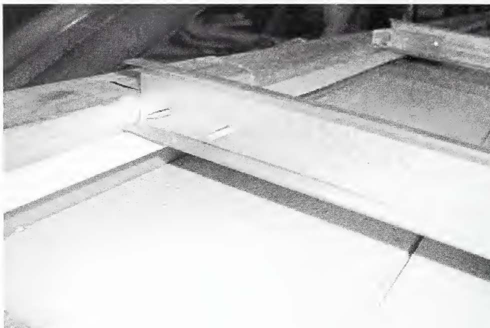
Figure 2–20. Channel section runner connection to edge of test frame in suspension system 1.
