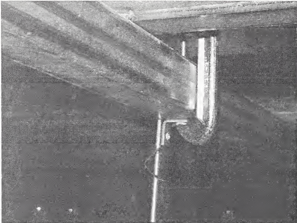
Figure 2–16. C-clamp and top CADDY fastener in suspension system 1.
