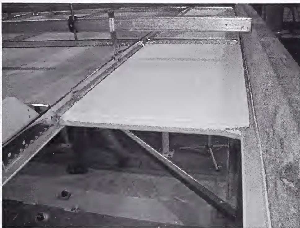
Figure 3–15. Damage to south perimeter of ceiling system CS4 after 1.75g earthquake excitation.
