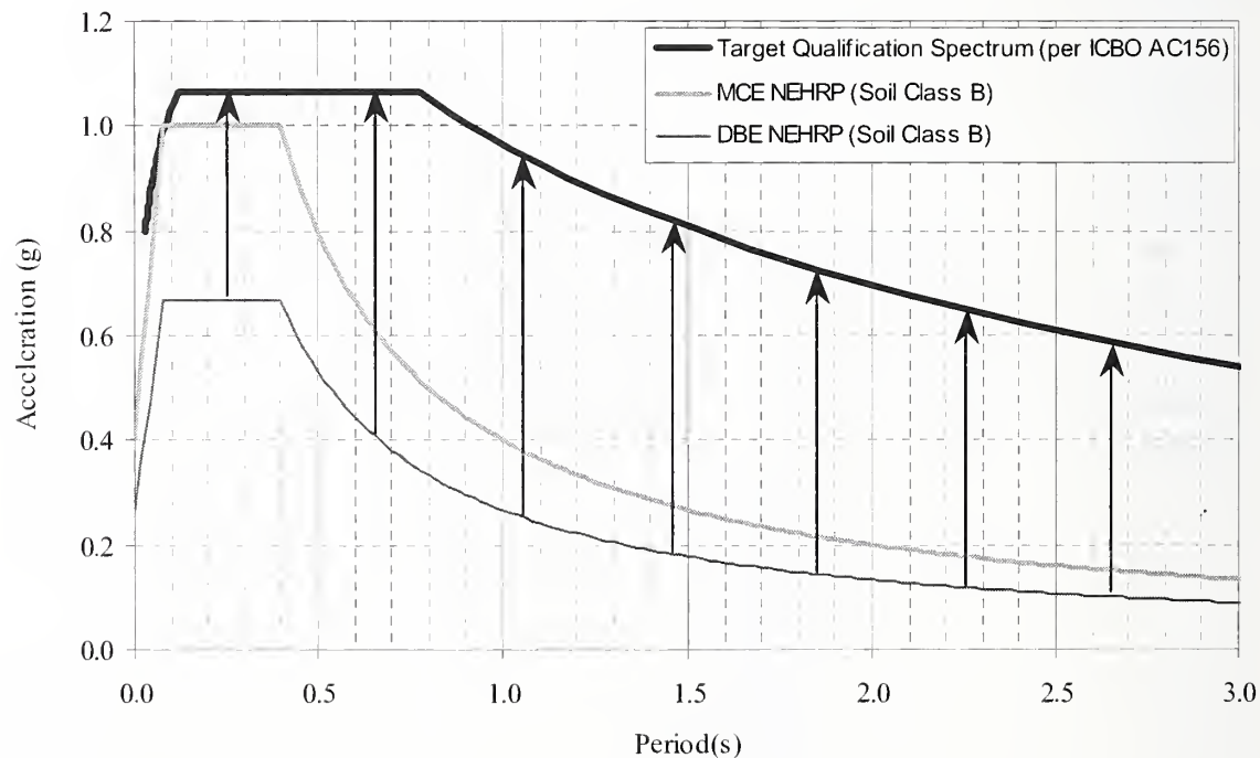
Figure 2-54. Relationship between NEHRP MCE and DBE spectra and target spectrum ( S_S=1.0g , S_I=0.4g ).
