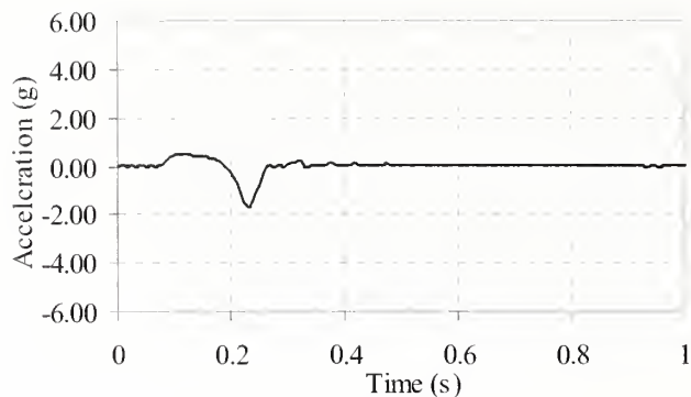
a) vertical acceleration ( Table )
