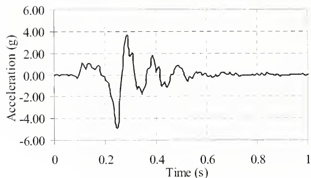
c) vertical acceleration ( Afram )
