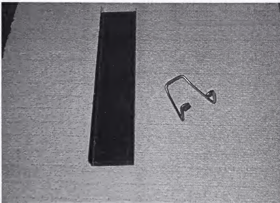
Figure 2–18. Z-bar section (left) and C-15 wire clip (right) in suspension system 1.
