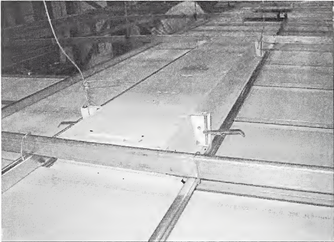
Figure 2–28. 12 in. by 48 in. (0.30 m by 1.22 m) fixture with safety clip and wires in ceiling system CS1.
