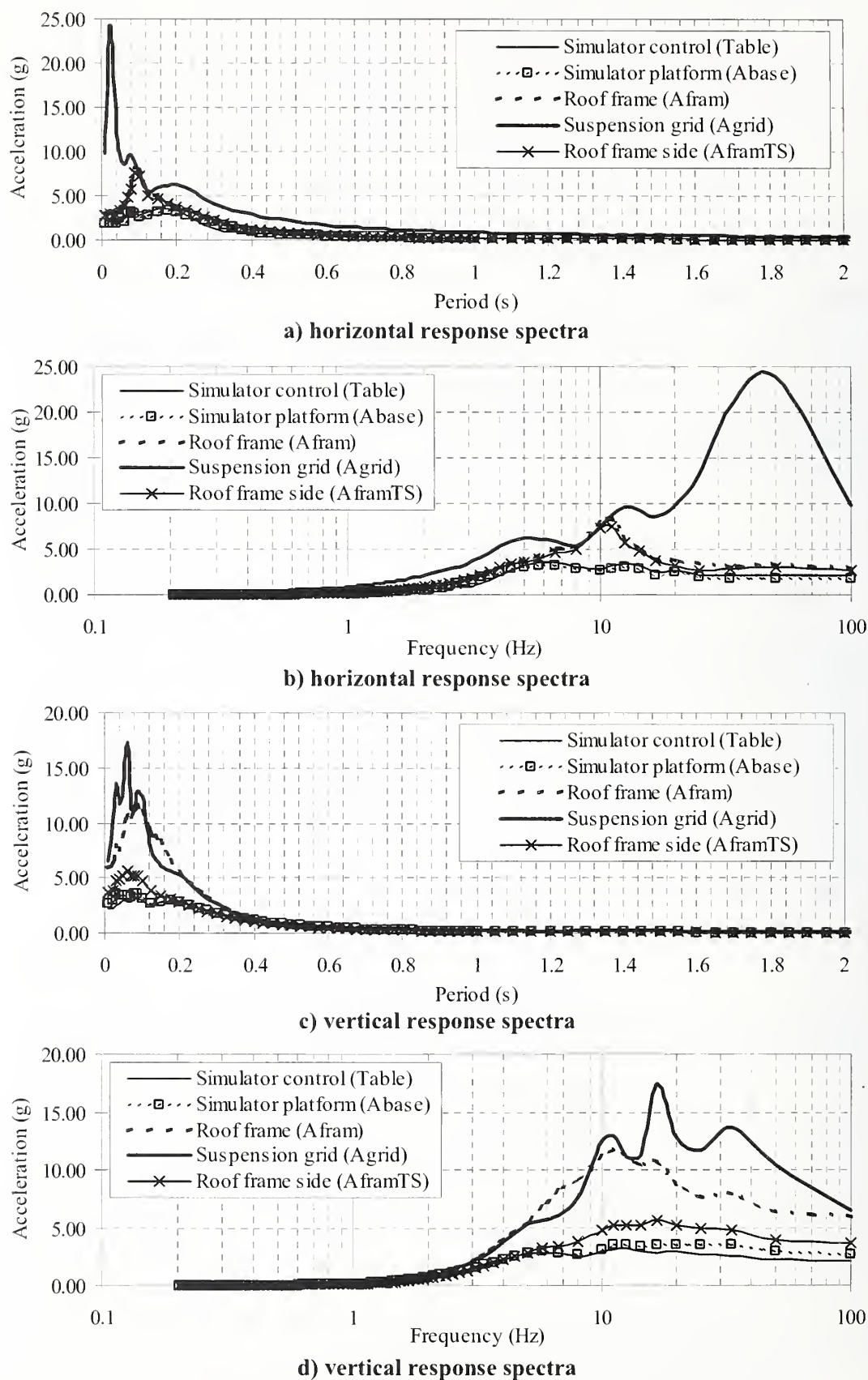
Figure A-15. Response spectra for Test 23 on ceiling system CS2.
