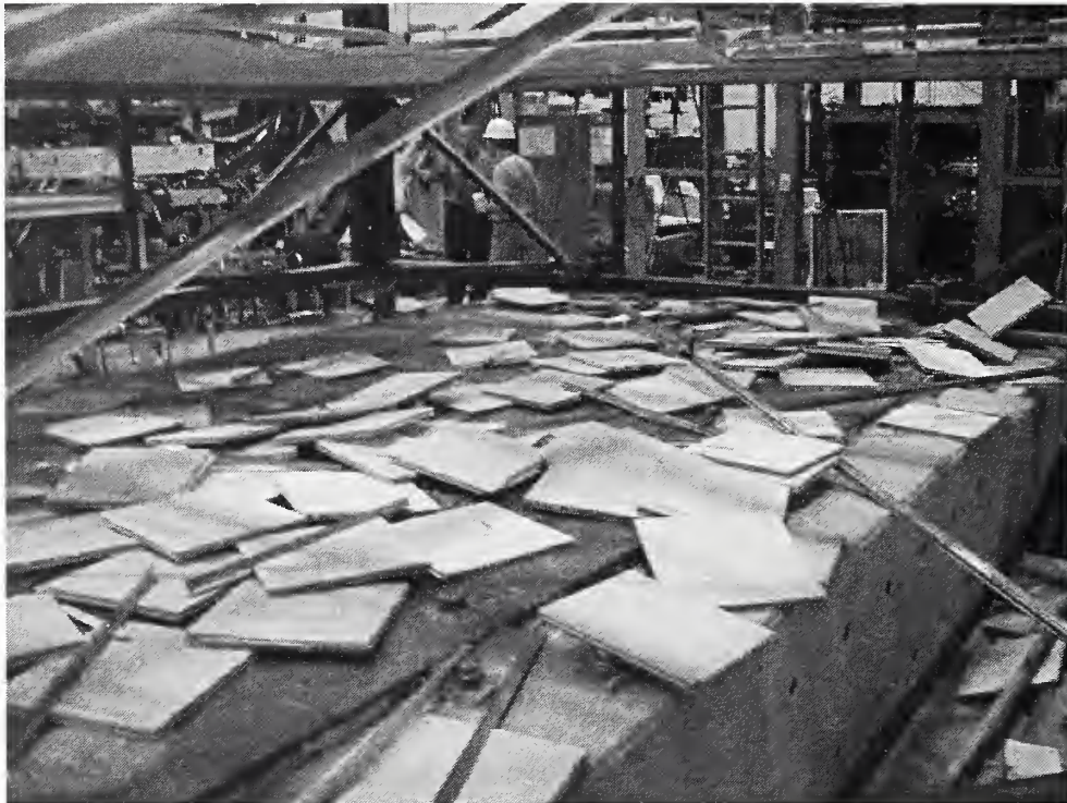
Figure 3–13. Collapse of ceiling system CS3 after 2.5g earthquake excitation.
