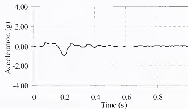
d) vertical acceleration ( AframTS )
