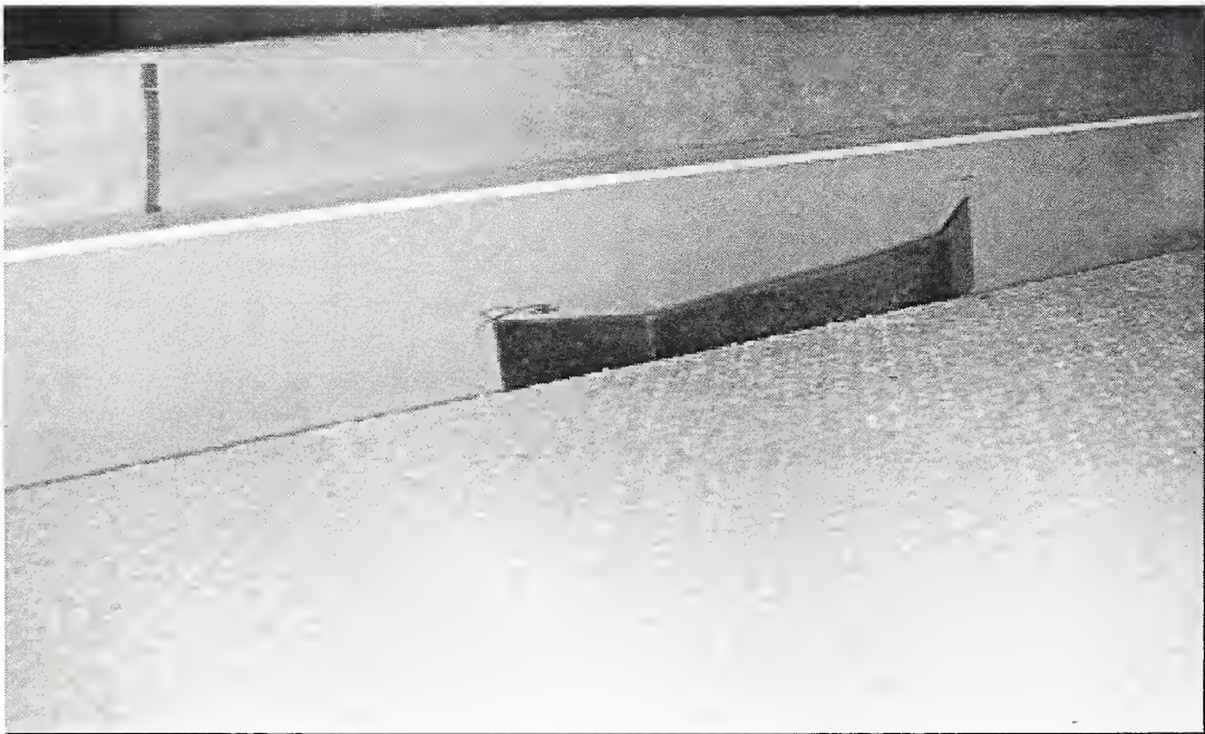
Figure 2–29. Panel perimeter spring clips in ceiling system CS1.
