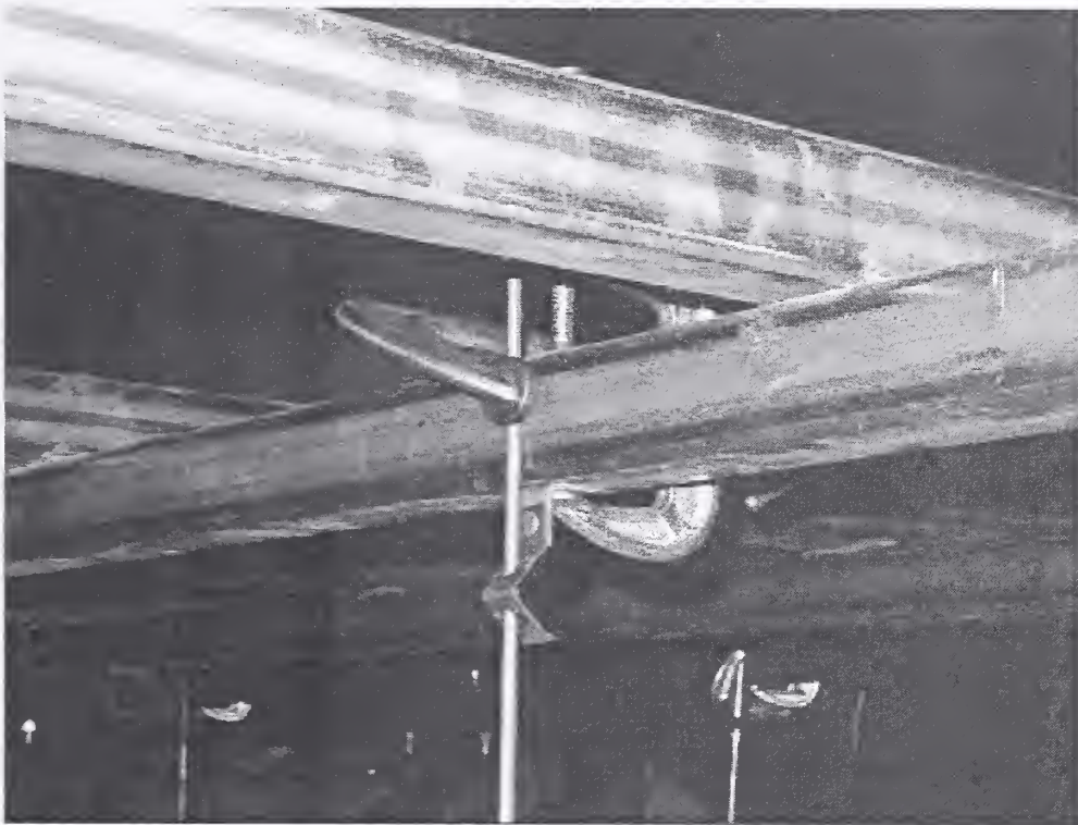
Figure 2–23. C-clamps and top CADDY clip in suspension system 2.
