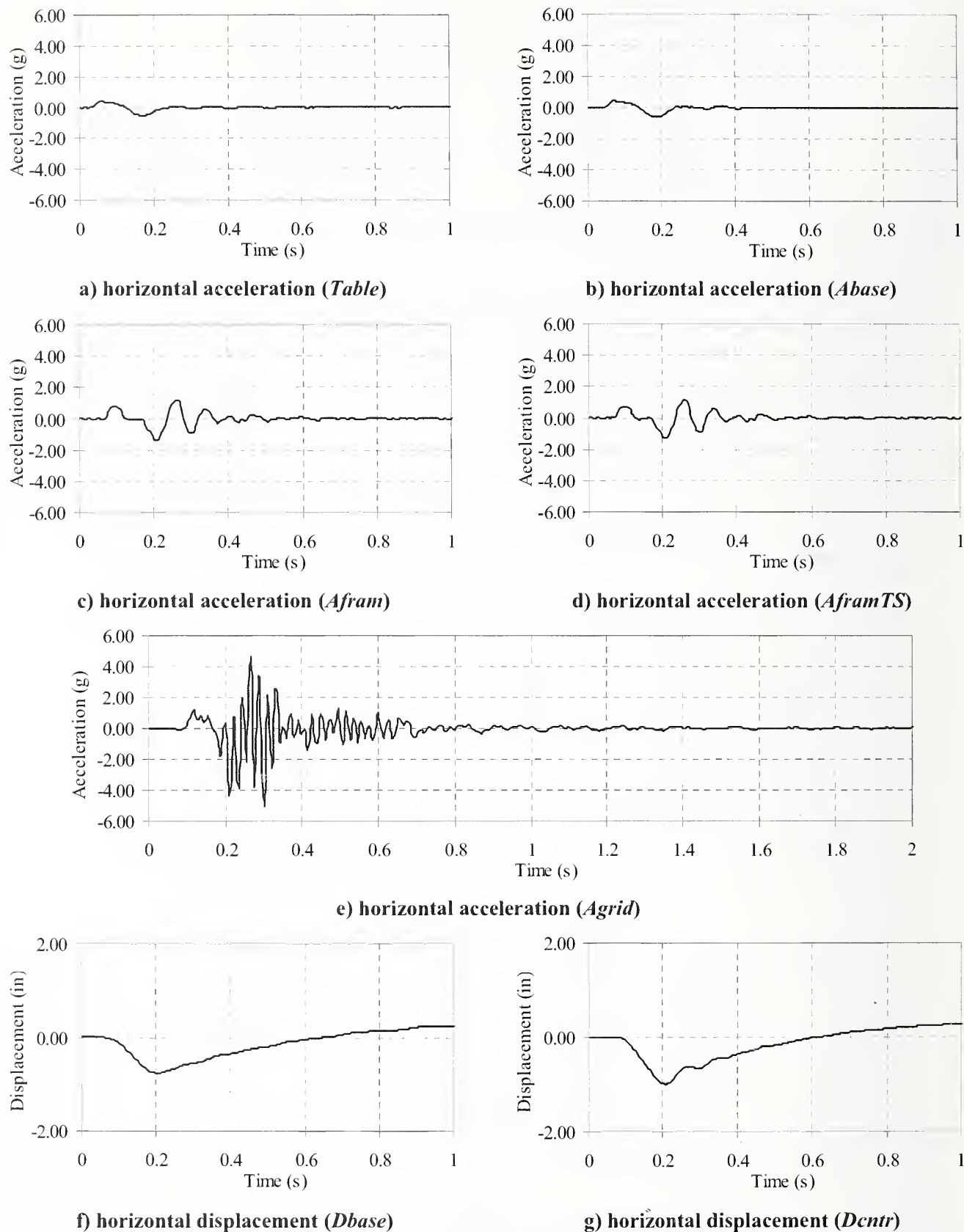
Figure A-7. Horizontal displacement and acceleration histories for Test 14 on ceiling system CS2.
