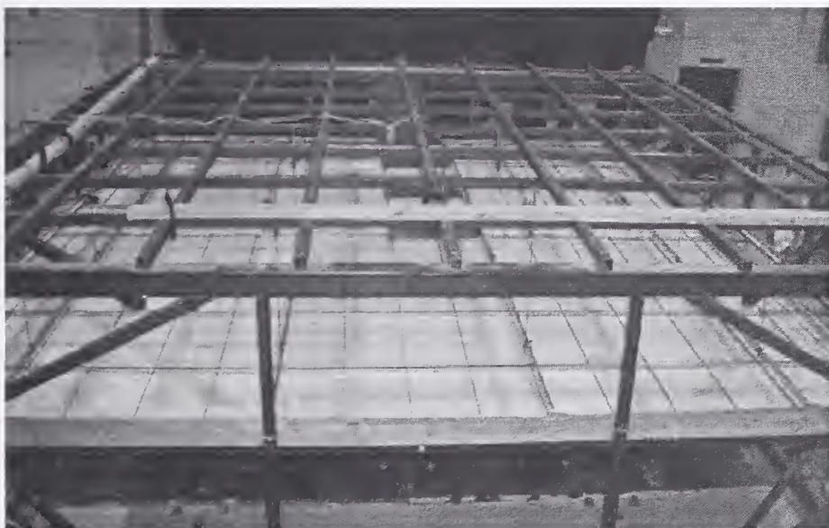
Figure 2–27. Top view of ceiling system CS1.
