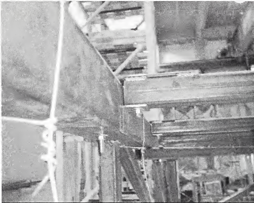
Figure 2–9. Connection of the roof to the main beams on the north side of the frame.
