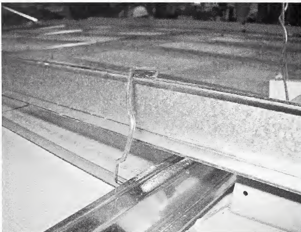
Figure 3–8. Stretching of Z-bar clips located at northern light fixture corner in ceiling system CS3 following Test 20.
