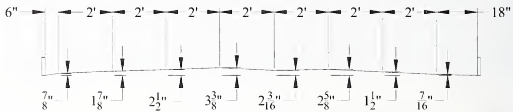
Figure 3–4. Permanent vertical displacements of Z-bars in the east-west direction following Test 20 for ceiling system CS1.
