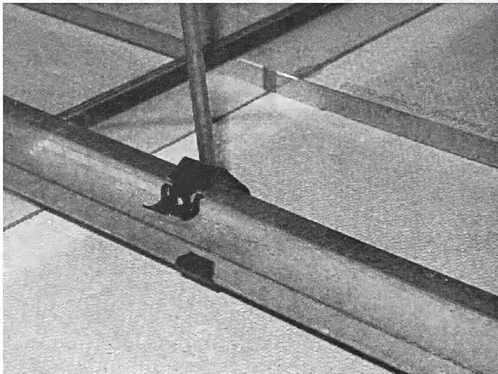
Figure 2–17. Bottom CADDY fastener in suspension system 1.
