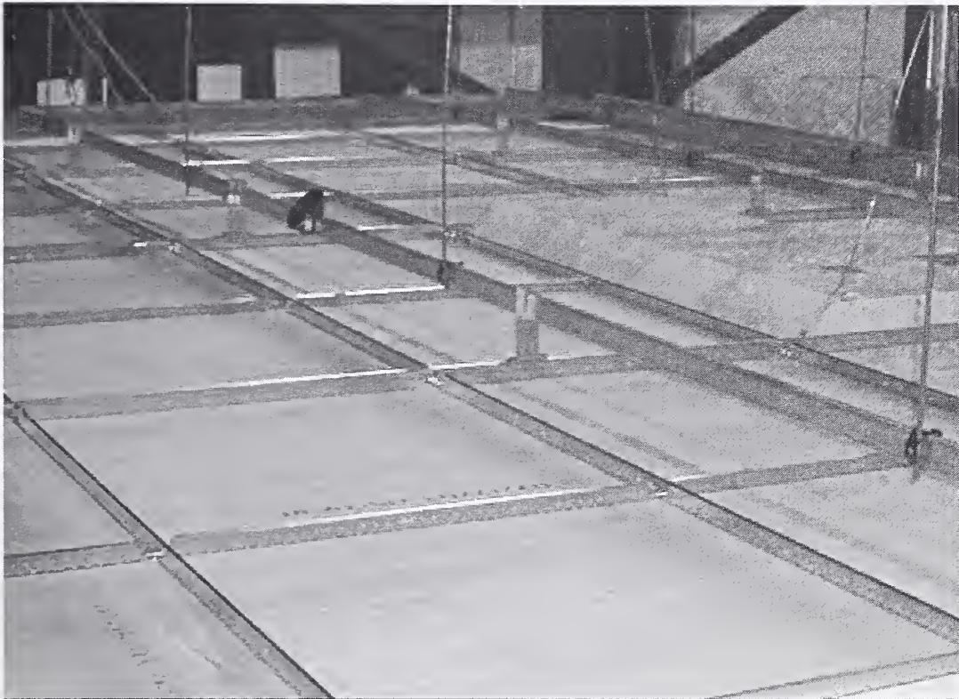
Figure 2–32. Top view of ceiling system CS2.
