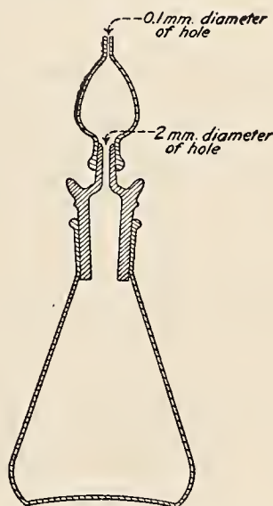
FIG. 2.—Pyknometer for viscous liquids (one-half actual size).
