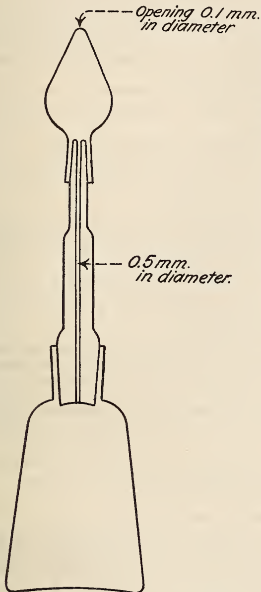
FIG. 1.—Pyknometer for very fluid liquids (actual size).
