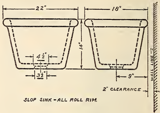
FIGURE 184.—Slop sinks, all roll rim
