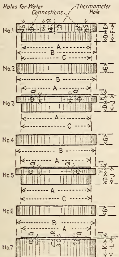
FIGURE 57.—Press-platen assembly
