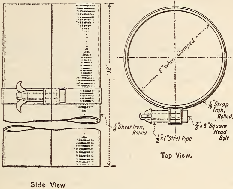
FIGURE 97.—Cement mold
