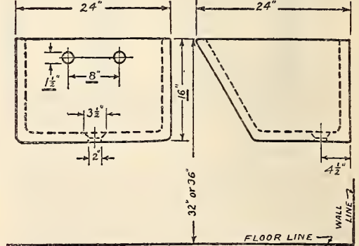
LAUNDRY TRAY - FLAT RIM. FIGURE 186.—Laundry trays, flat rim
