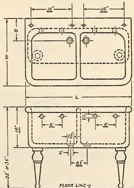
FIGURE 191.—Double laundry trays with extended ledge
