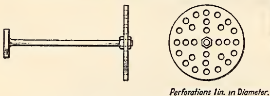
FIGURE 29.—Churn dasher type of stirrer
