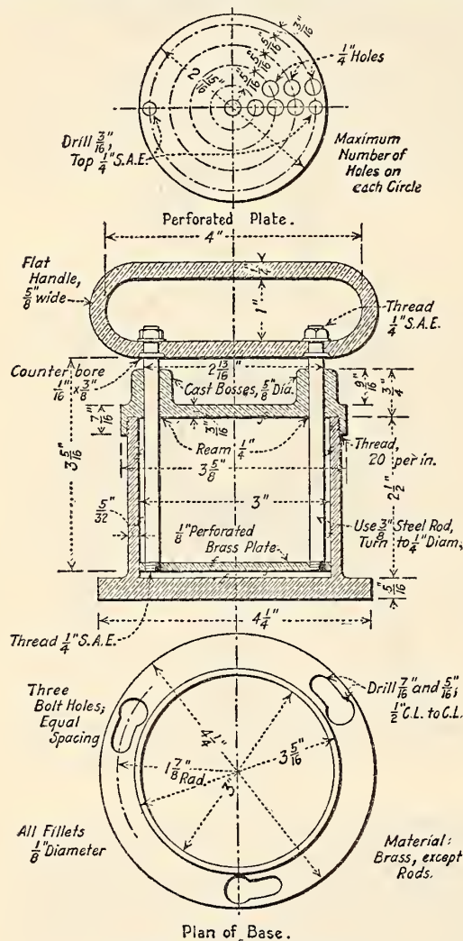
FIGURE 53.—Grease worker
