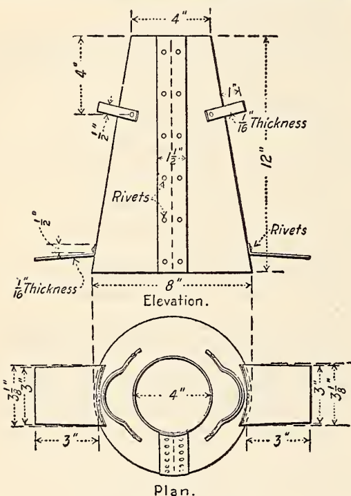
FIGURE 99.—Cement mold
