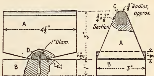
FIGURE 78.—Knife-edge
