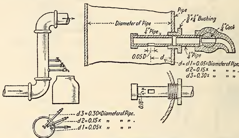
FIGURE 28.—Continuous sampling connection
