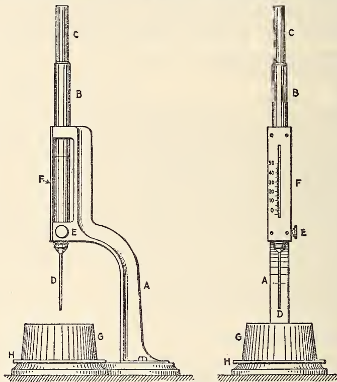
FIGURE 100.—Vicat apparatus
