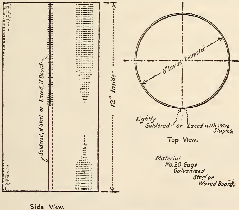
FIGURE 98.—Cement mold
