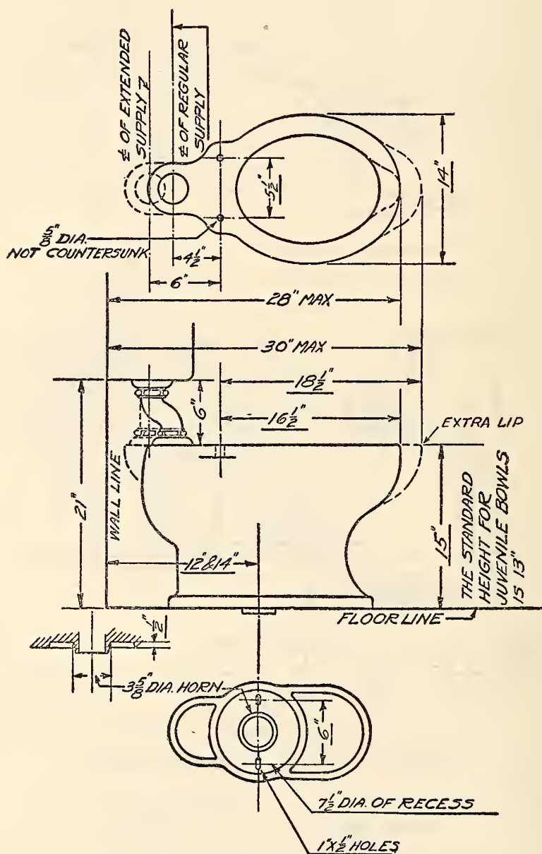
FIGURE 203.—Siphon jet water-closet bowls
