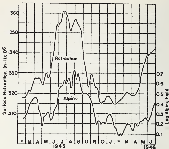
FIGURE 6.4. Field reception of W2XMN on 42.8 Mc/s at Needham, Mass., 1945-1946. (After Pickard and Statson, 1947).
