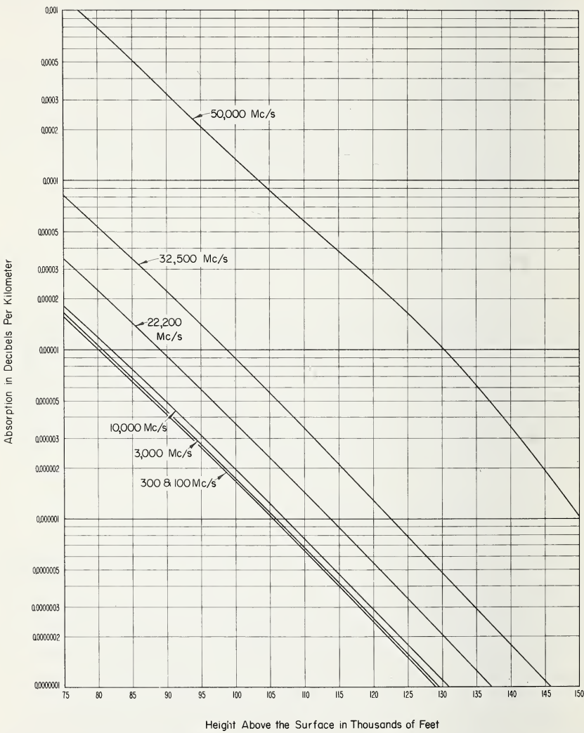
FIGURE 7.11. Common values of total gaseous atmospheric absorption for elevations greater than 75,000 feet.
