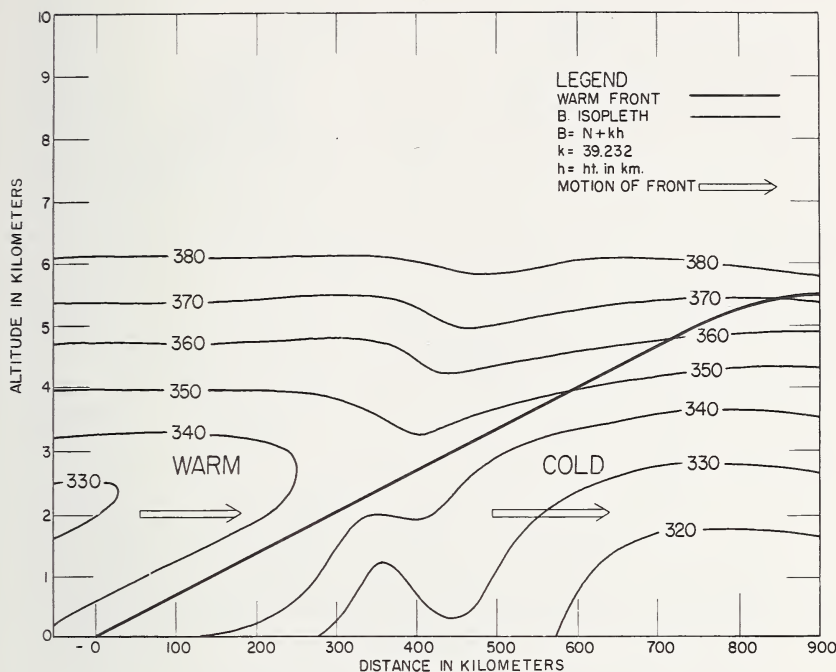
FIGURE 5.14. Idealized warm front in B units.
