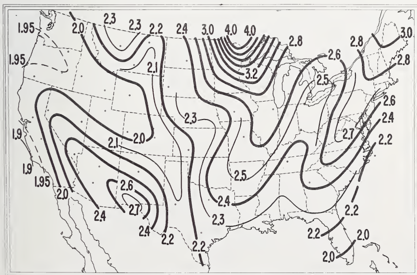
FIGURE 8.6. Wet term scale height, H_w , in kilometers for February.
