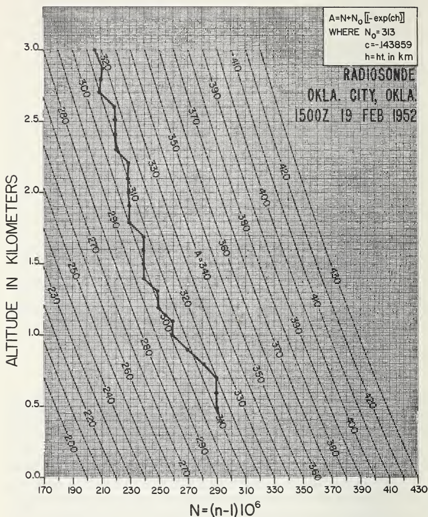
FIGURE 5.17. Potential refractivity chart.
