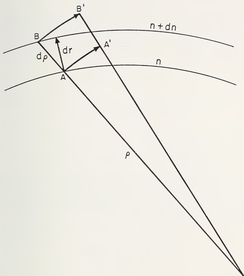
FIGURE 3.2. Differential geometry used in the derivation of the effective-earth's-radius-model atmosphere.
