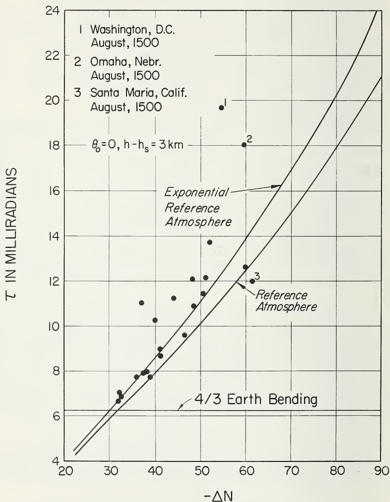
FIGURE 3.12. Comparison of \tau versus \Delta N as obtained from CRPL reference atmospheres—1958 and 5-year mean radiosonde data for \theta_0 = 0 , h - h_s = 3 km.
