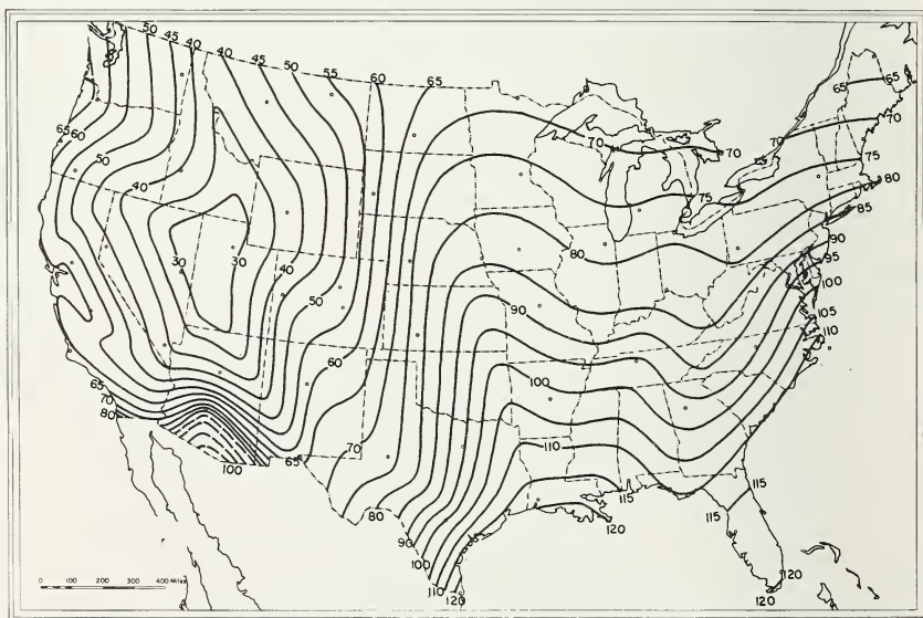
FIGURE 4.3. Mean W_s , August 0200 local time.
