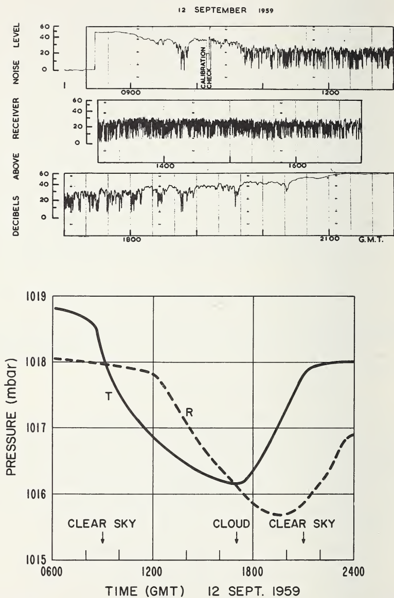
FIGURE 6.9. Signal records and pressure variations at transmitter, T, and receiver, R, on a 140 km path; f = 186 Mc/s.
