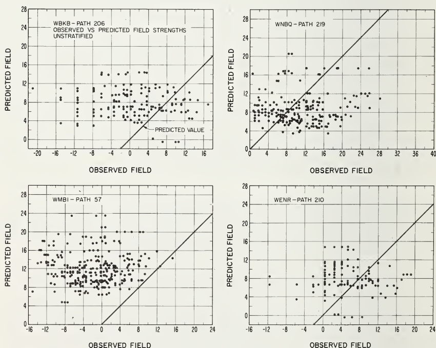
FIGURE 6.14. Comparison of observed radio field strengths and values predicted for wintertime afternoon hours.
