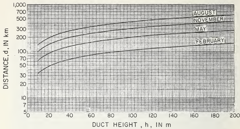
FIGURE 4.46. Shadow zone half-lengths for minimum ducting conditions at Washington, D.C.
