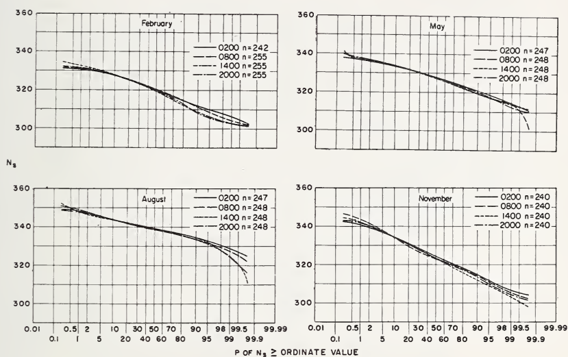
FIGURE 9.20. Cumulative probability distribution of N_s , Tatoosh Island, Wash.
