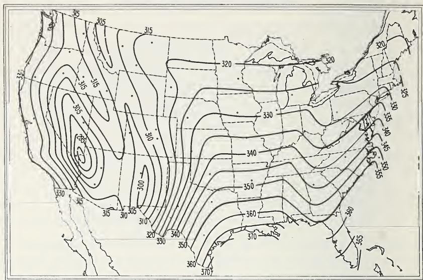
FIGURE 9.3. Mean N_0 , May 0200.
