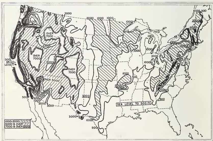
FIGURE 5.8. Ground elevation above sea level.
