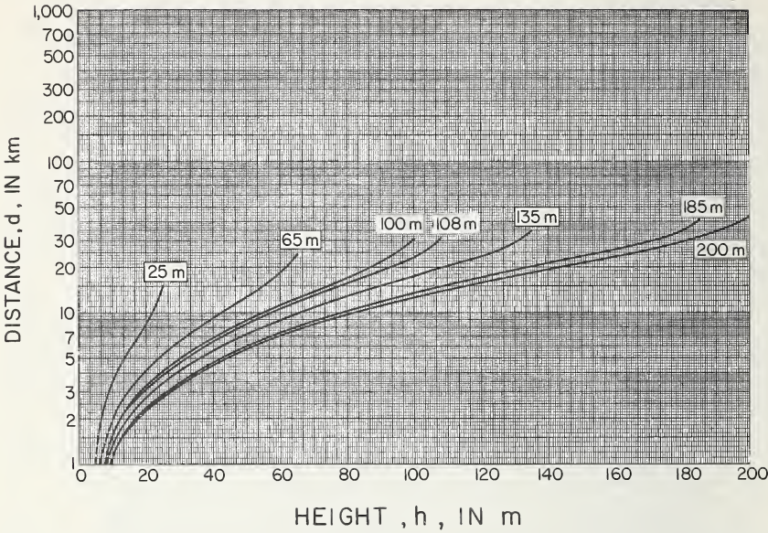
FIGURE 4.49. Height versus distance at Washington, D.C., for maximum midspring (May) ducting conditions.
