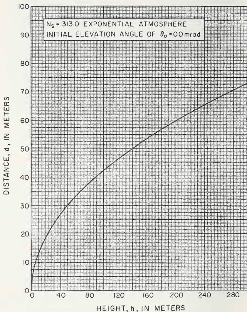
FIGURE 4.48. Distance versus height above duct representing average Washington, D.C., and Fairbanks, Alaska, atmosphere.
