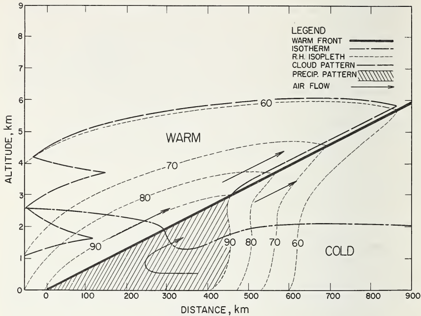
FIGURE 5.10. Idealized diagram of a warm front.
