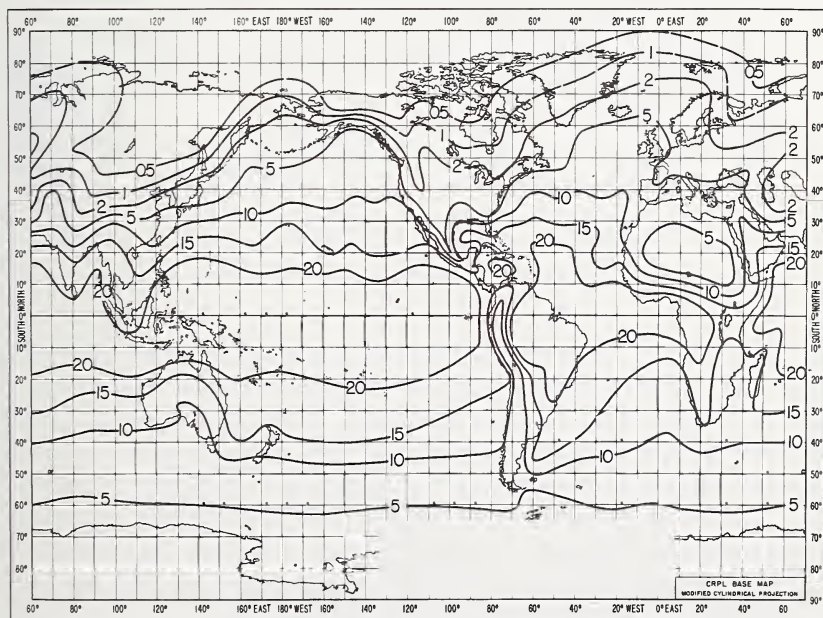
FIGURE 7.15. Average absolute humidity ( \text{g}/\text{m}^3 ), February.
