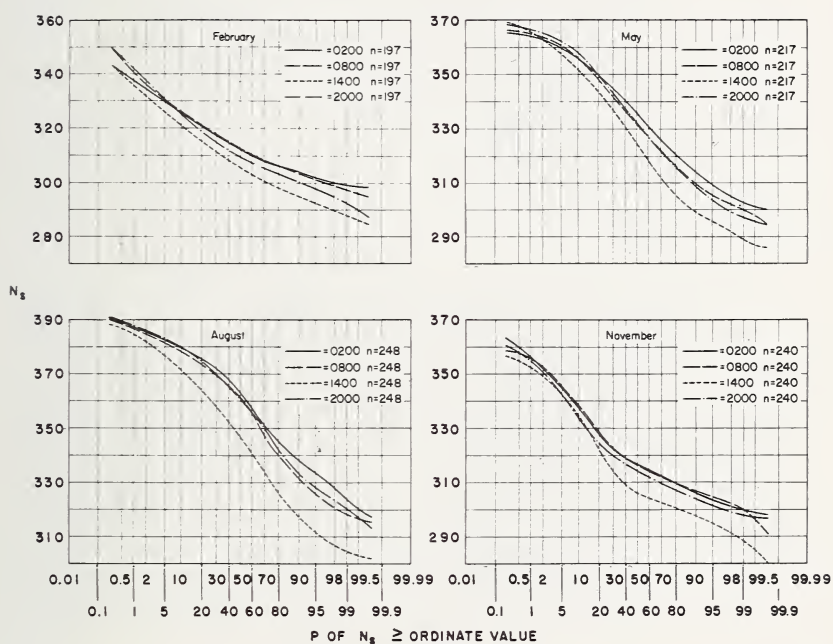
FIGURE 9.15. Cumulative probability distribution of N_s , Washington, D.C.
