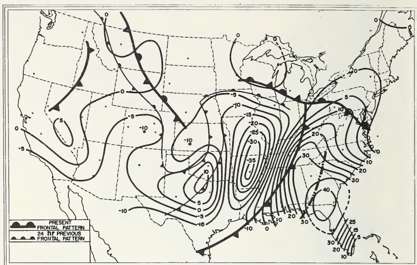
FIGURE 5.39. 24-hour \Delta N_{850} chart, 1000E 20 Feb. 1952.
