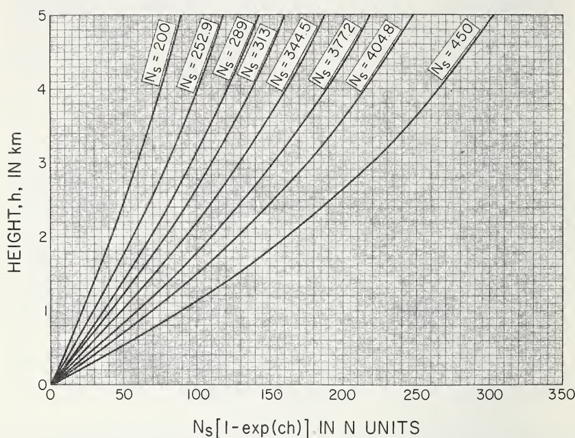
FIGURE 3.17. Graphic representation of N_s[1 - \exp(-ch)] in N units versus height.
