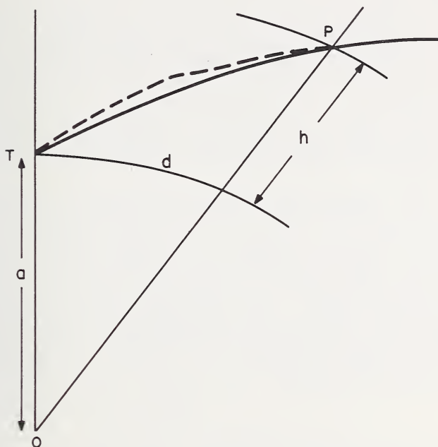
FIGURE 6.7. Geometry of the equivalent gradient.
