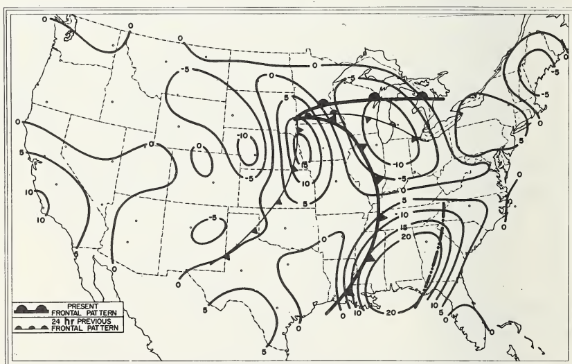
FIGURE 5.40. 24-hour \Delta N_{700} chart, 1000E 20 Feb. 1952.
