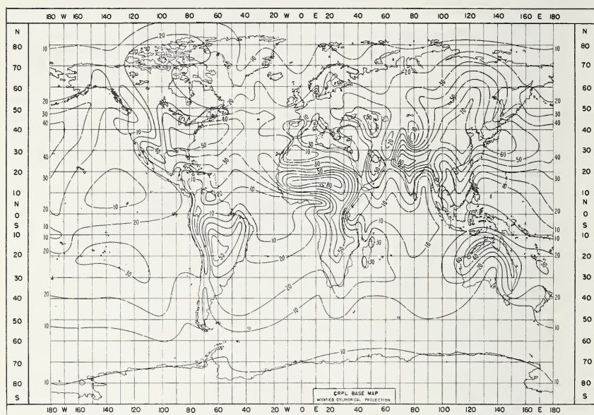
FIGURE 4.10. Annual range of monthly mean N_s .
