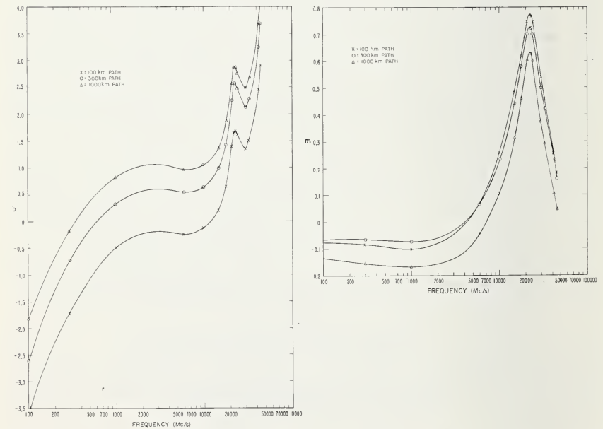
FIGURE 7.14. Values of b and m in the regression line y = mx + b , where y is the logarithm of the total path absorption, x is the logarithm of the absolute humidity, b is the value of y when the absolute humidity is 1 g/m 3 .
