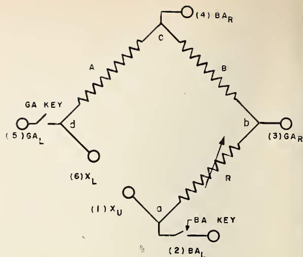
FIGURE 40. Identification of bridge binding posts with the post numbers of figure 35.
