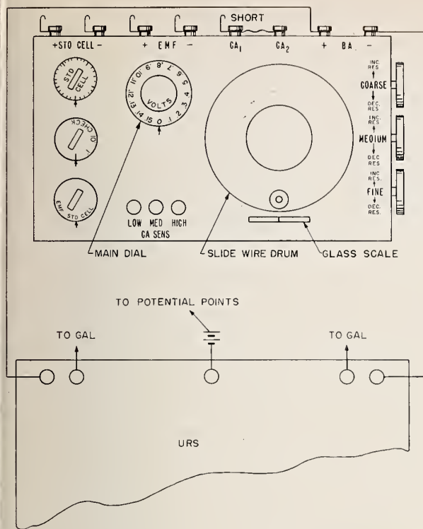
FIGURE 53. URS connected to a Crompton type potentiometer for testing.
