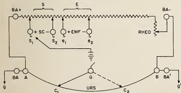
FIGURE 51. Testing a potentiometer with URS (schematic).
