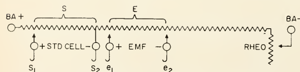
FIGURE 50. Simplified schematic diagram of potentiometer.
