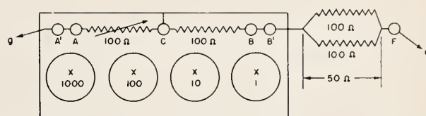
FIGURE 24. Adaptation of DRRS for 2:3 ratio.
