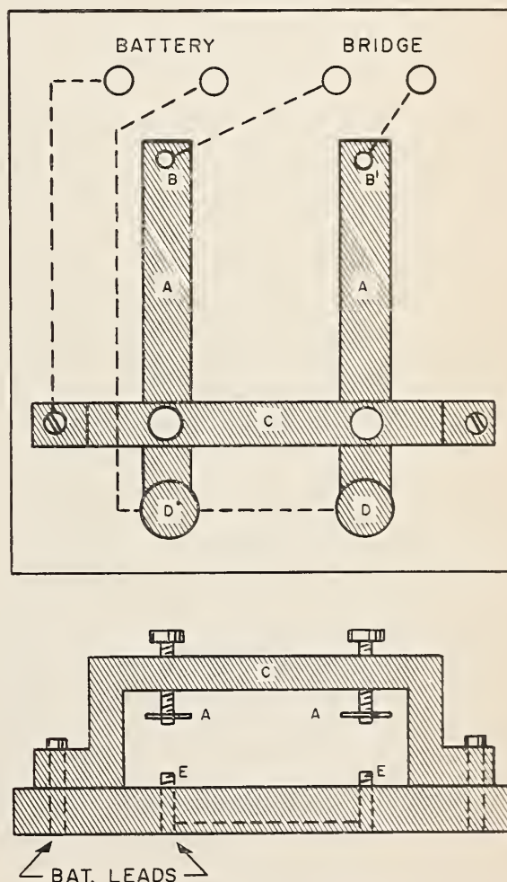
FIGURE 10. Reversing key.
