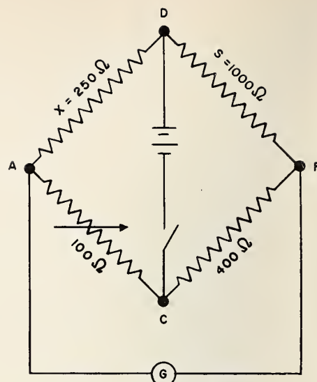
FIGURE 27B. Schematic circuit with the unknown, X, and the standard, S.
