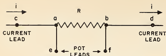
FIGURE 4. Four-terminal resistance.
