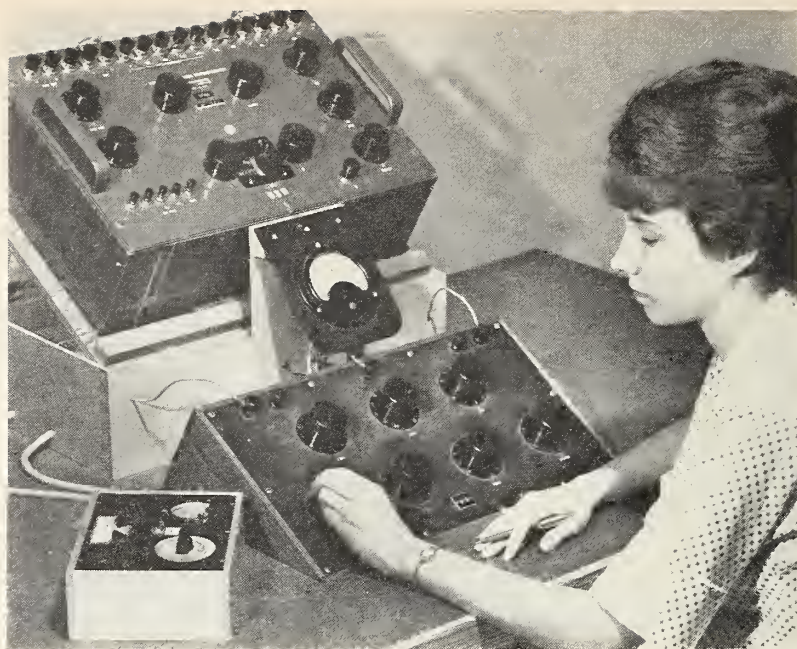
Universal Ratio Set connected for calibration of a potentiometer.
