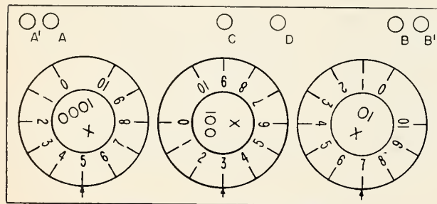
FIGURE 12. Three-dial DRRS.
