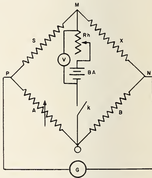
FIGURE 37. Recommended test circuit.
