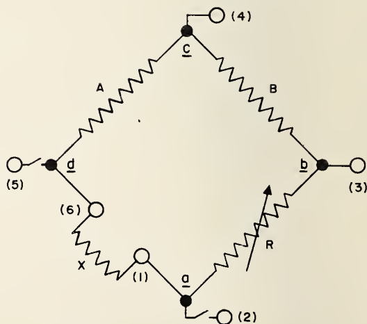
FIGURE 35. Generalized diagram of laboratory bridge.
