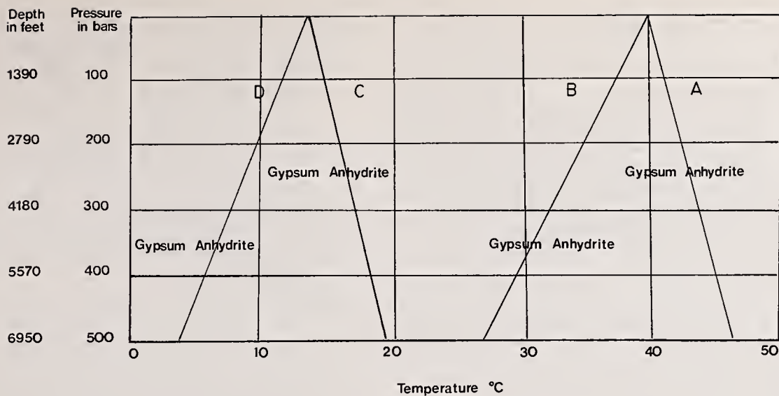
FIGURE 2.16. Pressure-temperature relations for the reaction \text{gypsum} = \text{anhydrite} + \text{water} .
