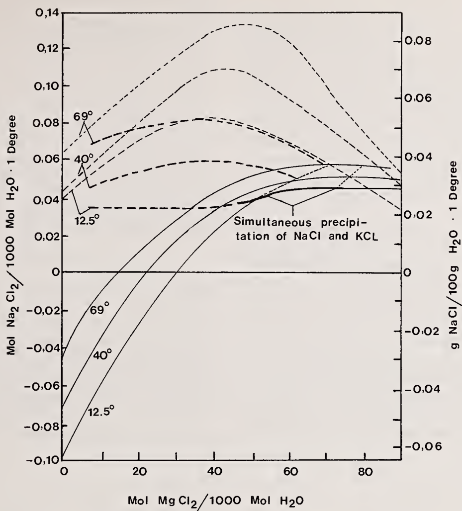
FIGURE 2.7. Ref. [44]. Temperature coefficient of NaCl solubility at temperatures from 0-70°C and \text{MgCl}_2 concentrations — — — system \text{NaCl-MgCl}_2\text{-H}_2\text{O} saturated in NaCl; ——— system \text{NaCl-KCl-MgCl}_2\text{-H}_2\text{O} saturated in NaCl and KCl; - - - \text{MgSO}_4 free seawater, NaCl-saturated, KCl-unsaturated; ——— the same, simultaneous precipitation of NaCl + KCl; following by simultaneous precipitation of NaCl + carnallite.
