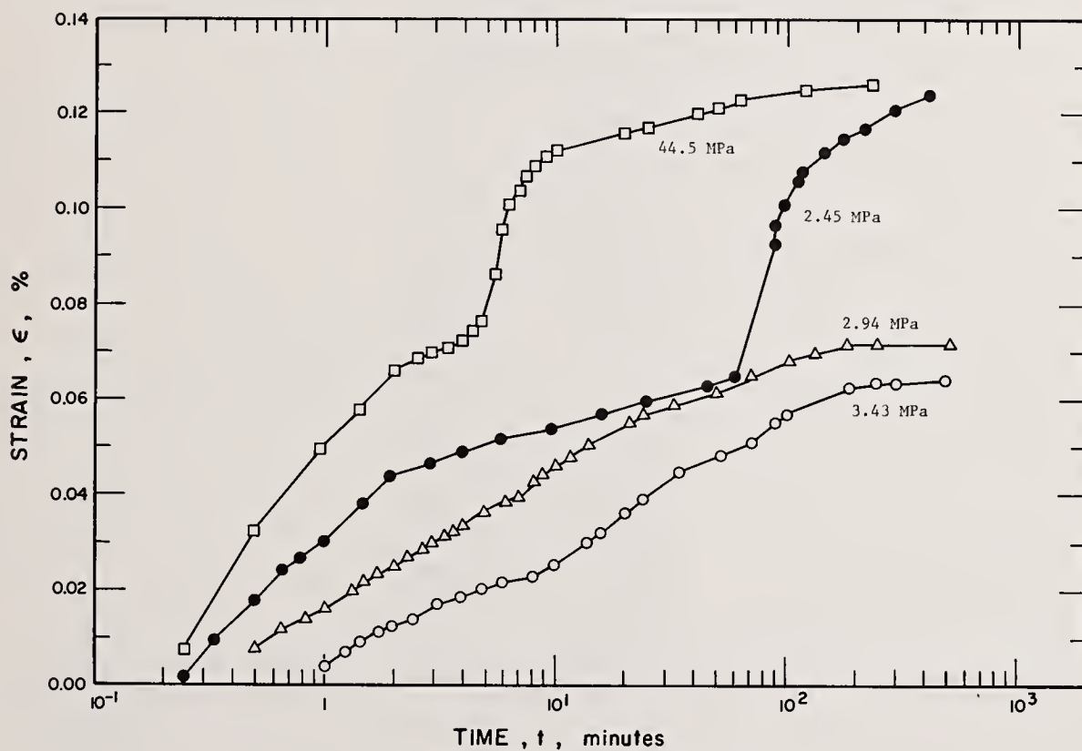
FIGURE 3.26. Nonuniform creep of NaCl.
