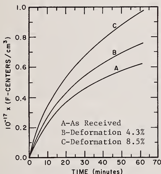
Figure 5.9. Early stage of F-band growth for irradiated NaCl crystals [68].
