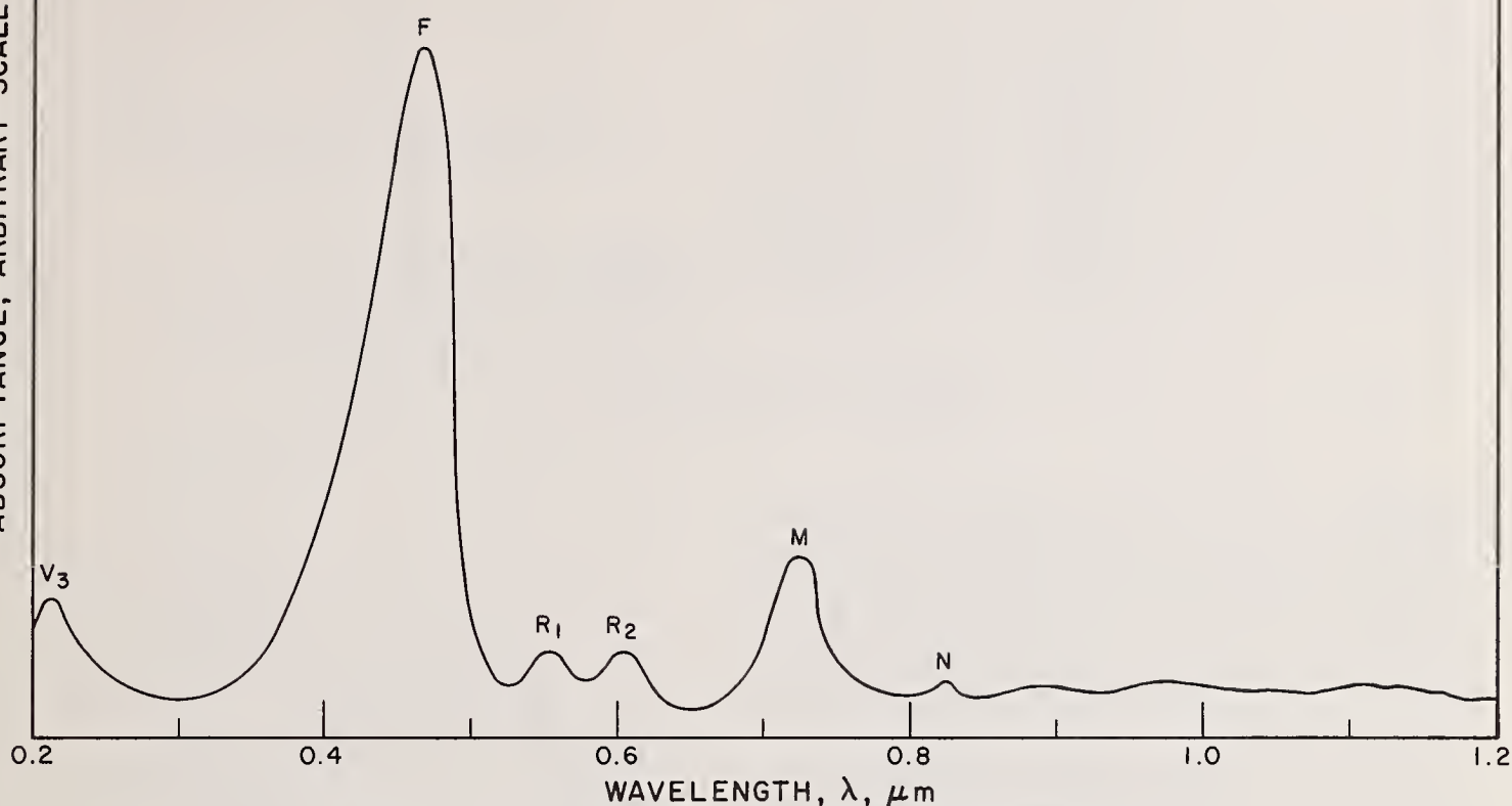
Figure 5.5. Typical Absorption Spectrum of Irradiated Rock Salt
