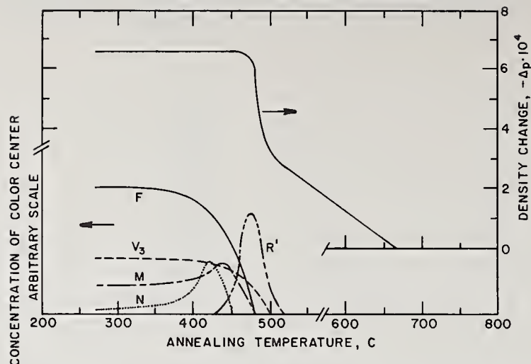
Figure 5.6. Annealing out of absorption bands and of density change in proton irradiated NaCl as a function of increasing temperature [64].
