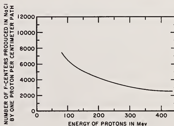
Figure 5.11. Number of F-centers produced by one proton per cm path in NaCl irradiated with 10^{16} protons/ \text{cm}^2 [70].
