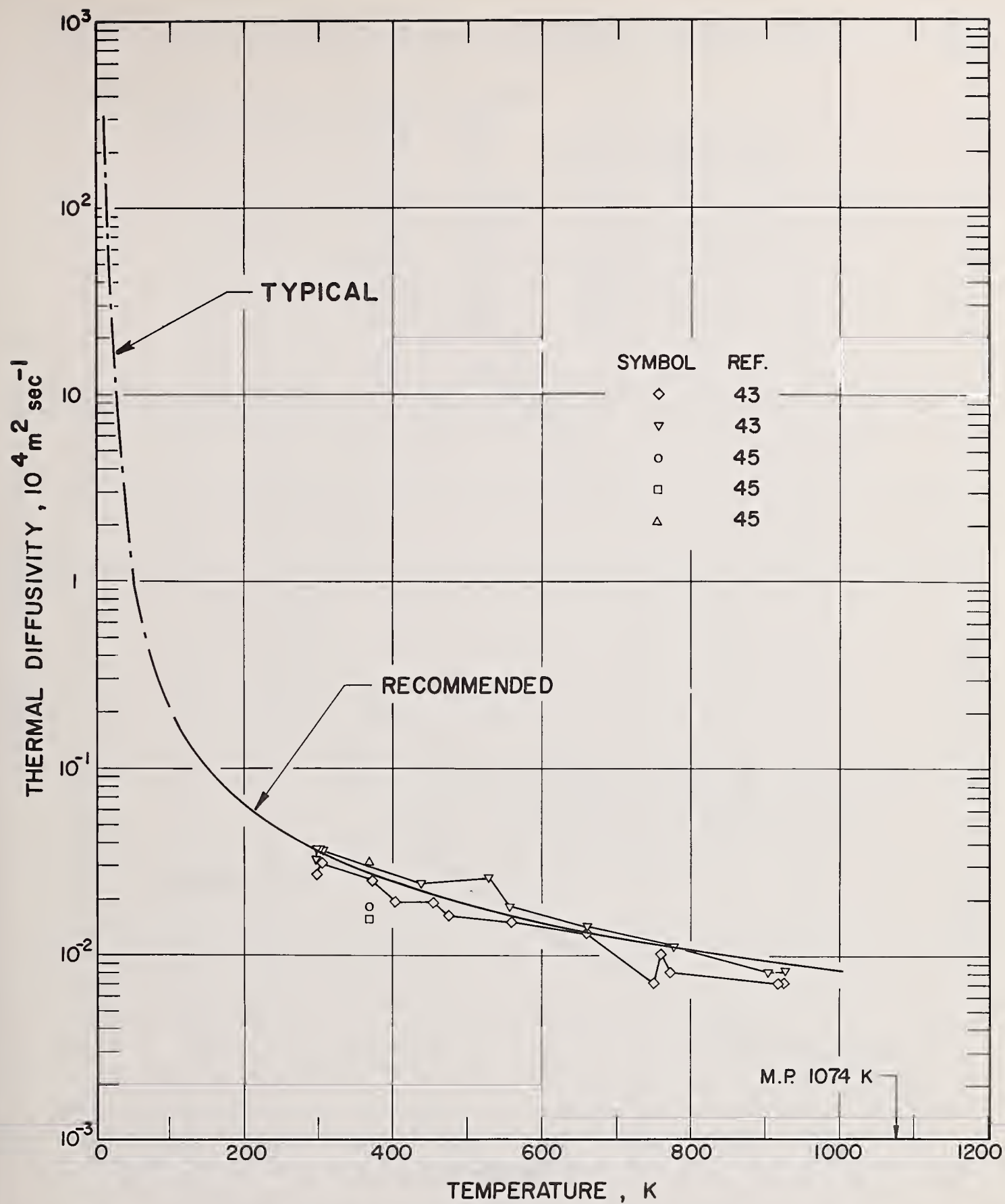
Figure 4.2. Thermal Diffusivity of Rock Salt.
