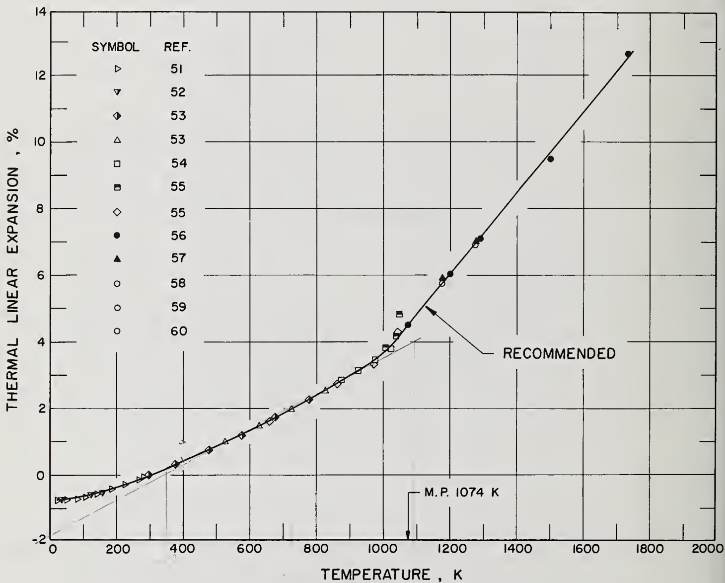
Figure 4.3. Thermal Linear Expansion of Rock Salt.
