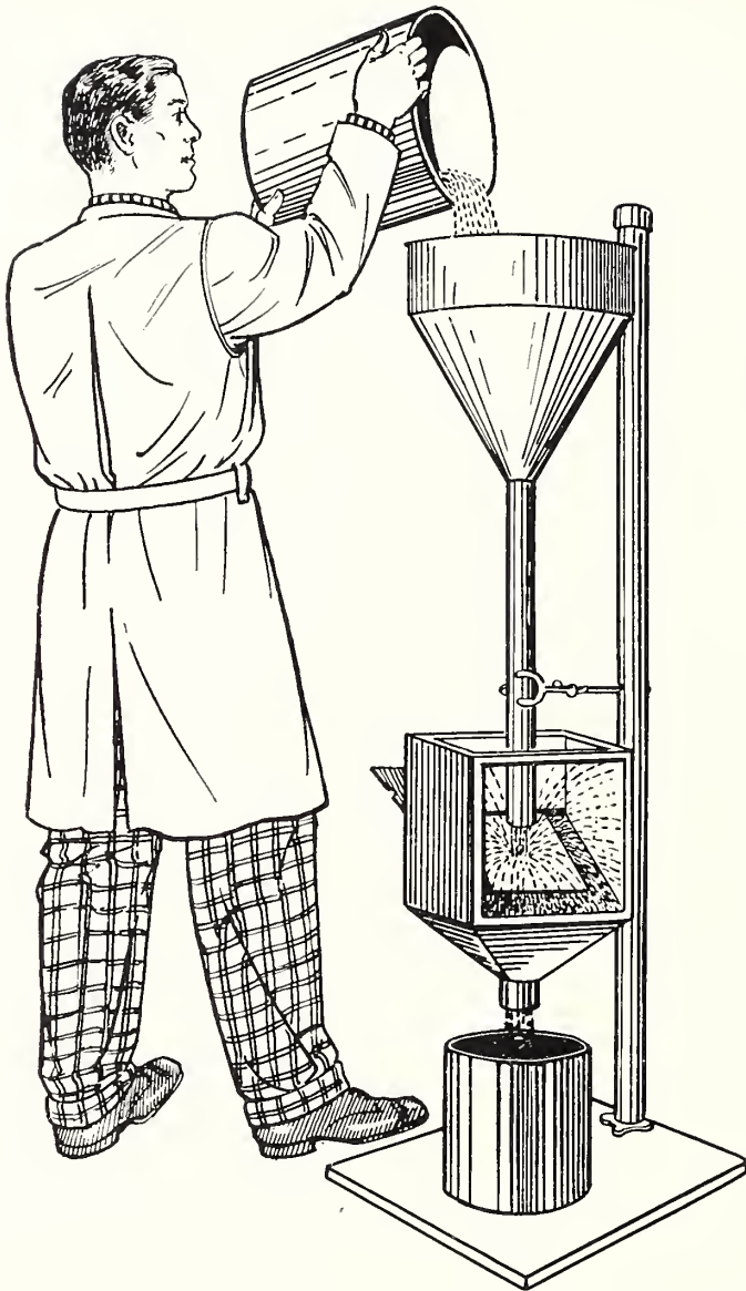
WEAR TEST FOR FLOOR FINISHES. Floor finishes were tested for their abrasion resistance by placing a coated panel in the abrasion resistance apparatus. Particles of sand impinge upon the surface, and the weight of sand in grams required to wear the coating through to the metal panel is an index of the wearability of the floor finish.
