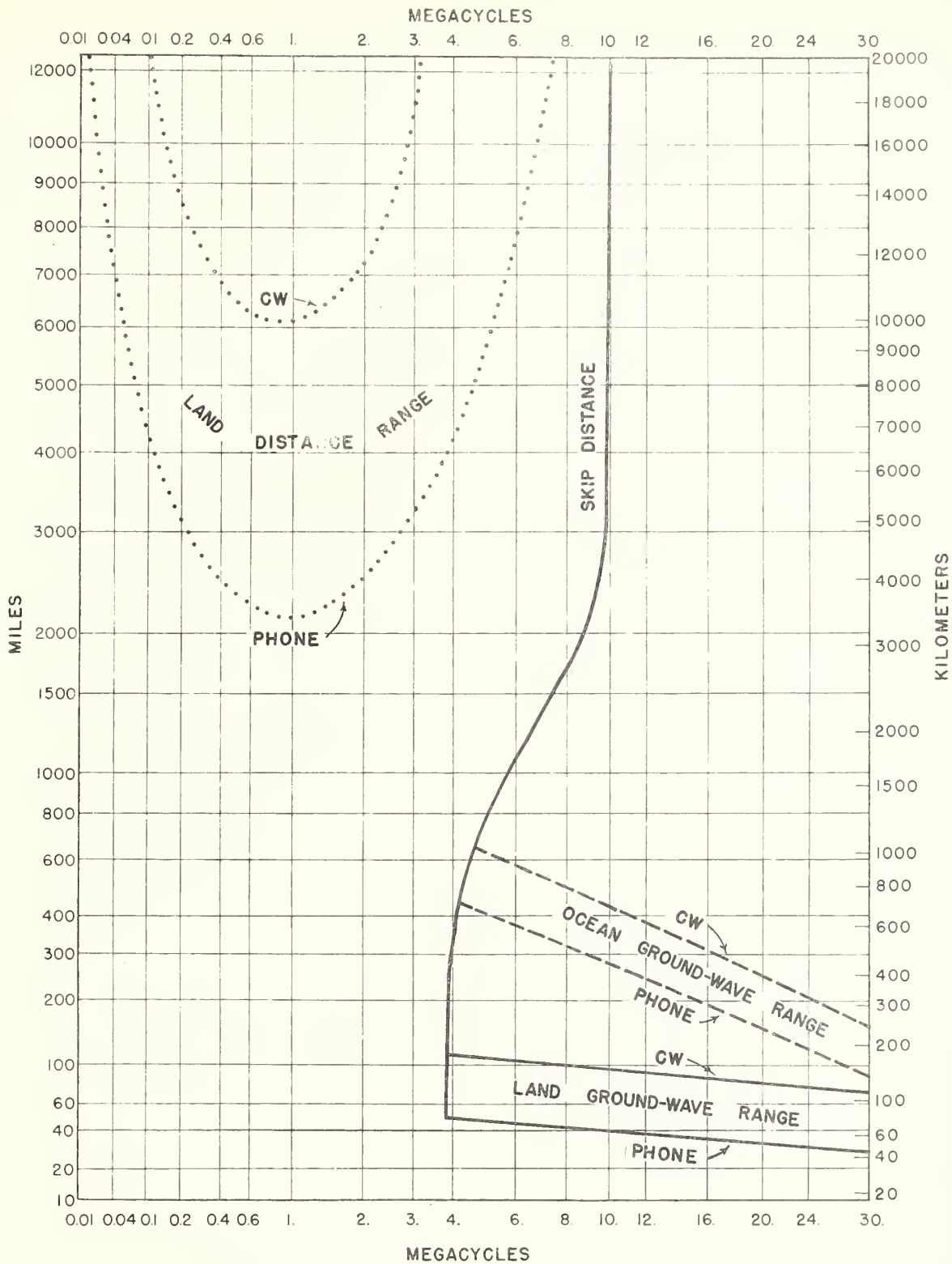
FIG. 4. WINTER 1941-42, NIGHT, (1 kw).
