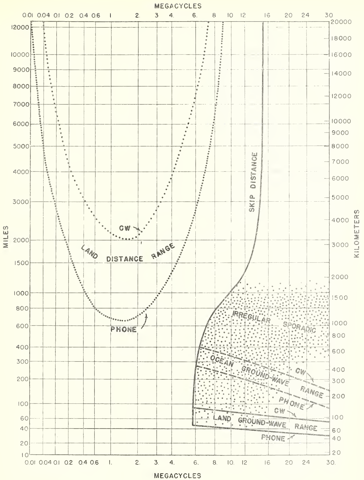
FIG. 2. SUMMER 1941, NIGHT, (1 kw).
