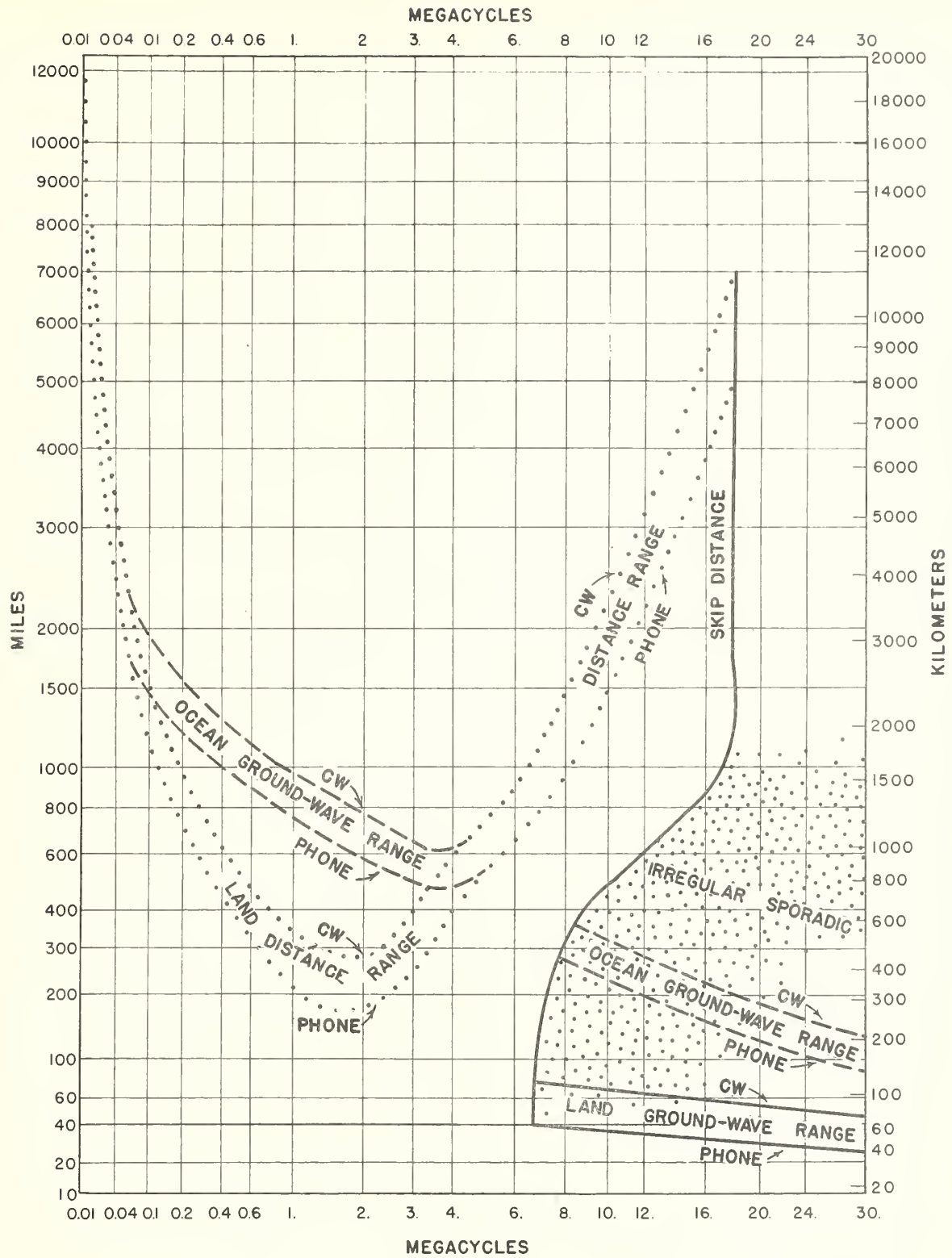
FIG. I. SUMMER 1941, DAY, (1 kw).
