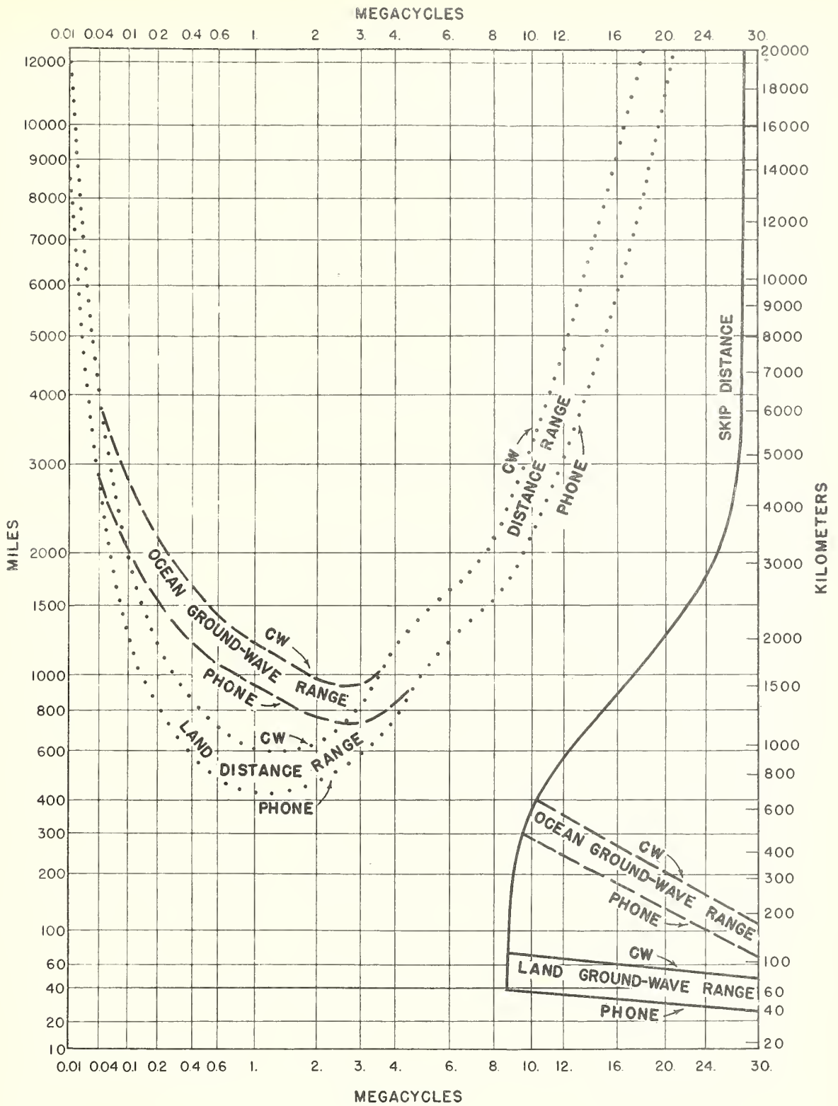
FIG. 3. WINTER 1941-42, DAY, (1 kw).
