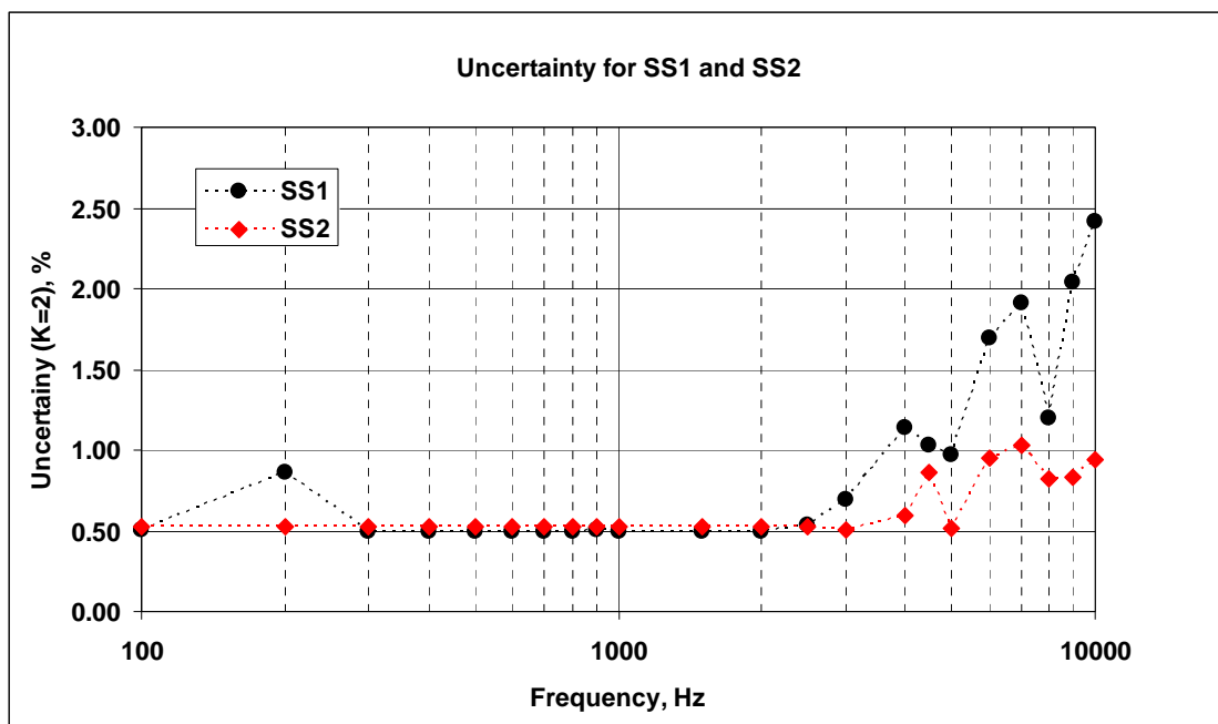
Figure 15. Calculated uncertainties for SS1 and SS2
