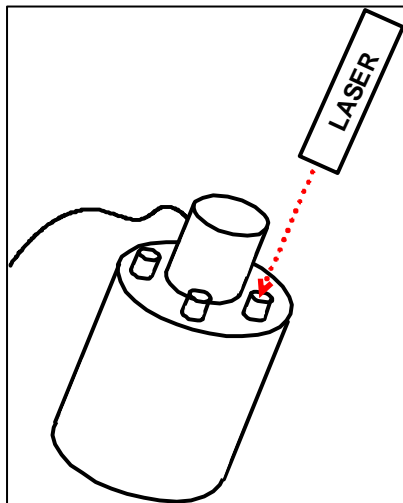
Figure 12. Conventional three-mirror method for calibration using a single coil or piezo-electric shaker for interferometric calibration
