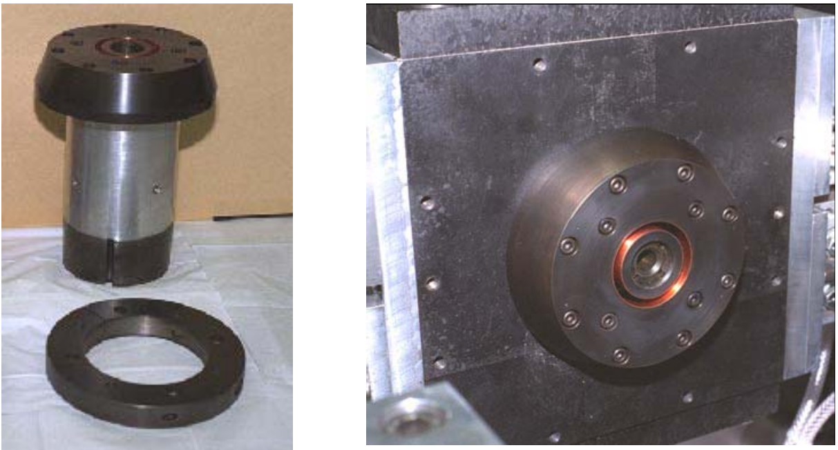
Figure 4. Inner gap assembly (left) and complete magnet assembly (right)
