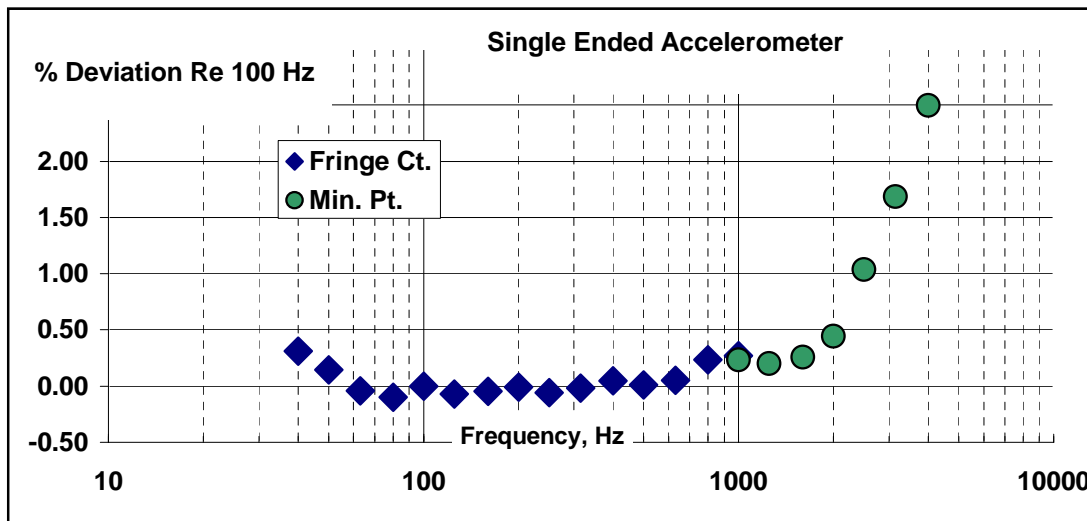
Figure 11. Calibration data for a single-ended accelerometer using fringe-counting and minimum-point methods
