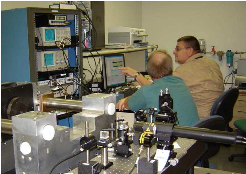
Figure 1b. SS1 with instrumentation and optical components of laser interferometer at AFMETCAL, Heath, OH
