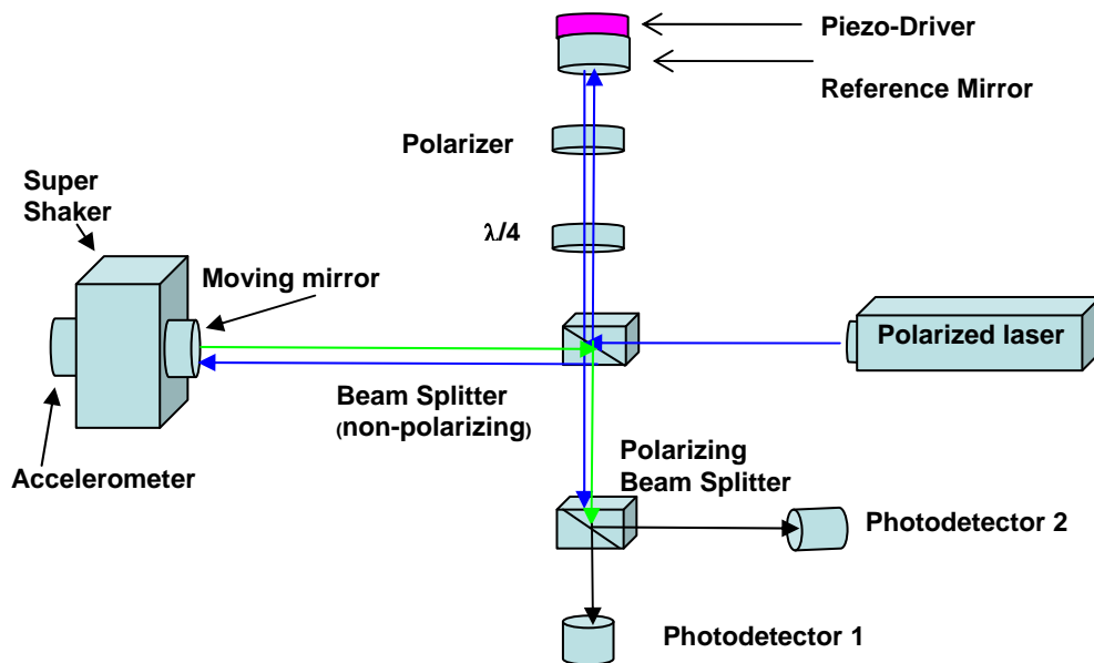
Figure 13. Setup using quadrature laser interferometer for sine-approximation, minimum-point, and fringe-counting methods
