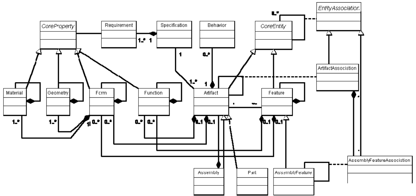
Figure 9: CPM and OAM classes relevant to PDS linking
