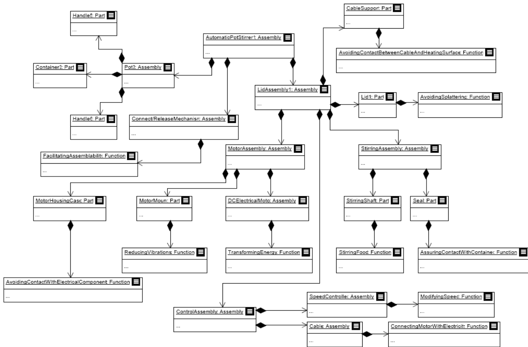
Figure 11: Assemblies and Functions of the Automatic Pot Stirrer
