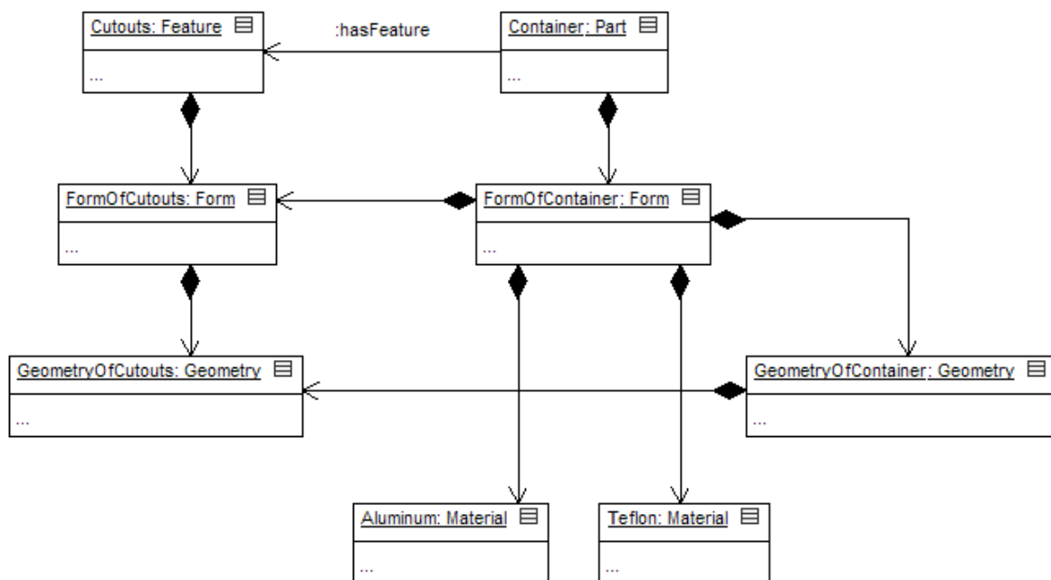
Figure 13: Form of the Container and form of its feature
