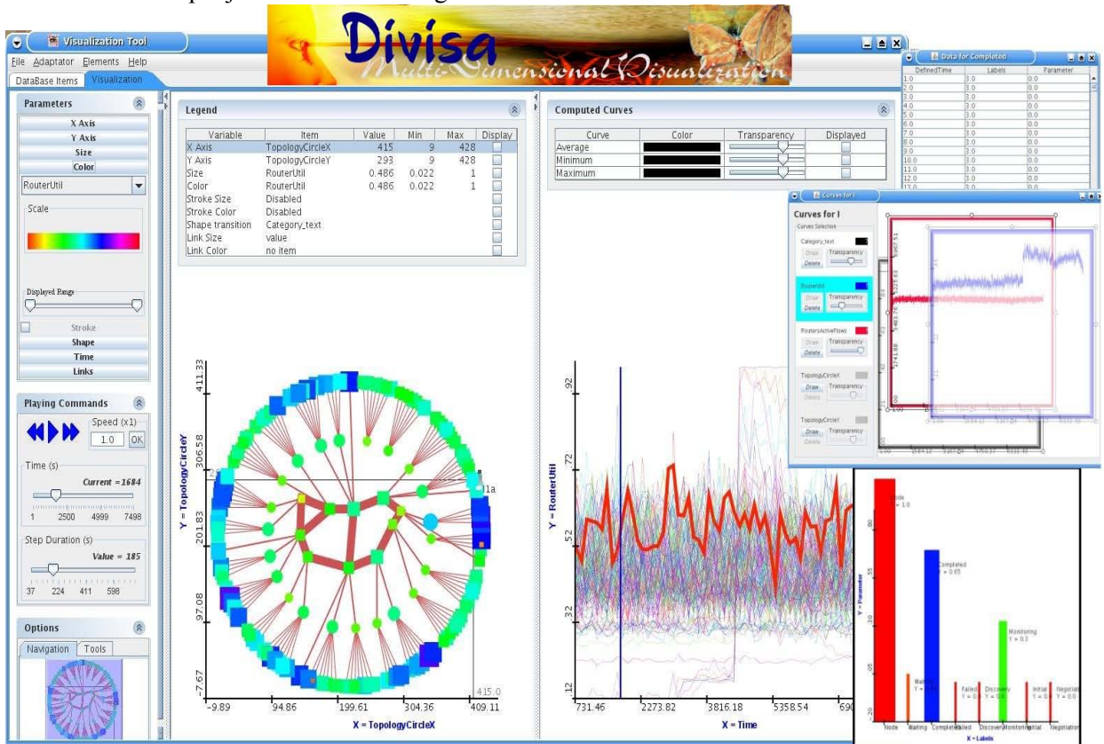
One frame from an animated visualization of a simulation of the “Abilene” network. On the left panel, the innermost nodes are the backbone routers, the next ring represents the subnet routers, and the outermost ring shows the leaf routers. On the right panel, the time series curves of the routers (one is currently selected) are displayed. On the right side, different options are available: numeric data display (top), superposed time series curves (middle); and diagram view (bottom).
