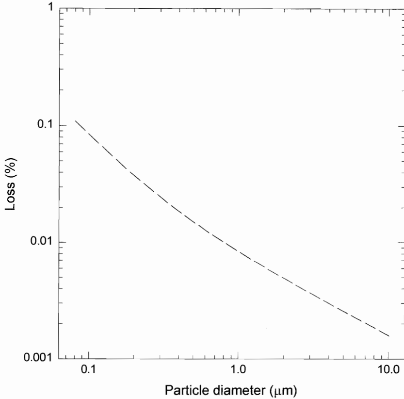
Figure A1. Diffusion loss as a function of particle diameter in the entrance tube.
