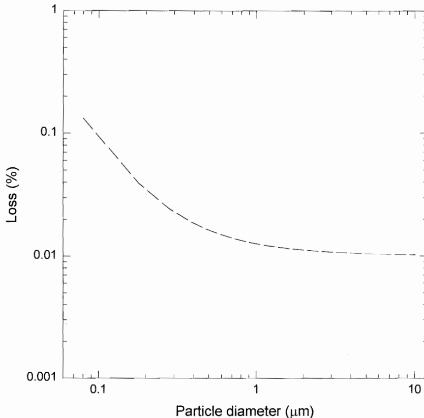
Figure A2. Diffusion loss as a function of particle diameter in the saturator with no insert.
