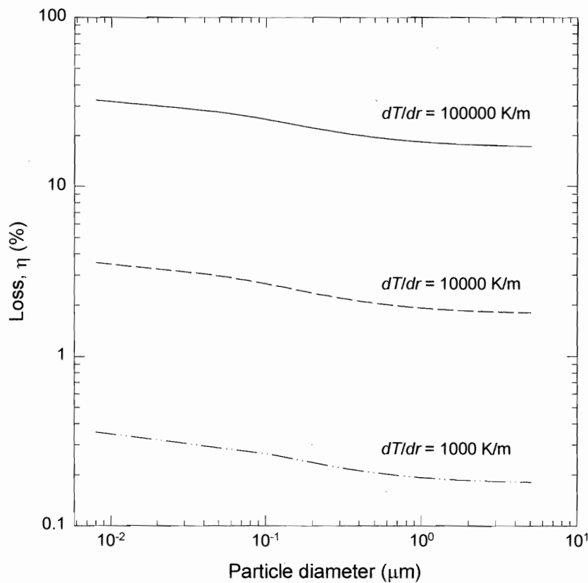
Figure A5. Particle loss due to thermophoresis as a function of particle diameter at various temperature gradients.
