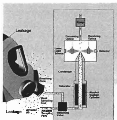
Figure 1. Schematic of the M41. (Courtesy of TSI)
