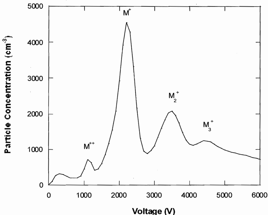
Figure 5. DMA voltage scan of 80 nm polystyrene spheres nebulized from water suspension. M^{++} , M^+ , M_2^+ and M_3^+ are the doubly charged monomer peak, the singlet monomer peak, the singlet dimer peak, and singlet triplet, respectively.
