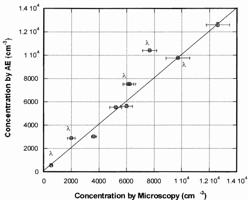
Figure 15. Comparison of the aerosol concentration determined by microscopy and AE where \lambda denotes counts determined for agglomerated particles. The uncertainty bars correspond to the expanded uncertainty. The data (two points) at approximately 6000 \text{cm}^{-3} corresponds to the concentration derived from two independent sets of images collected on the same filter. A 1:1 line is drawn for comparison.
