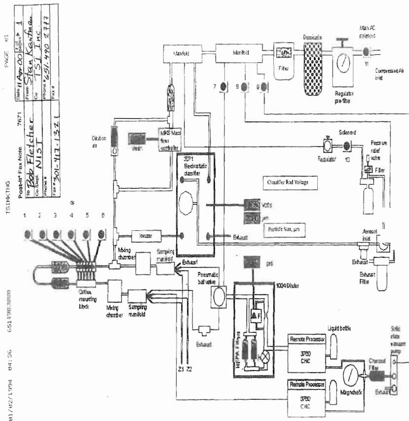
Figure 2. Schematic of the TSI built test stand used to verify M41 performance. (courtesy of TSI)
