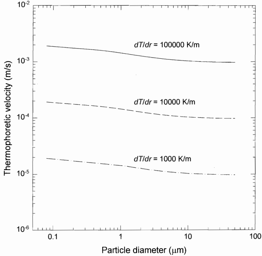
Figure A4. Thermophoretic velocity and particle loss as a function of particle diameter
