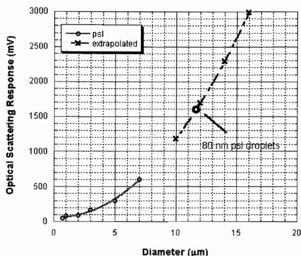
Figure A10. Plot of CPC optical scattering response as a function of particle diameter. The top part of the curve is extrapolated and the bottom is fitted to polystyrene spheres.
