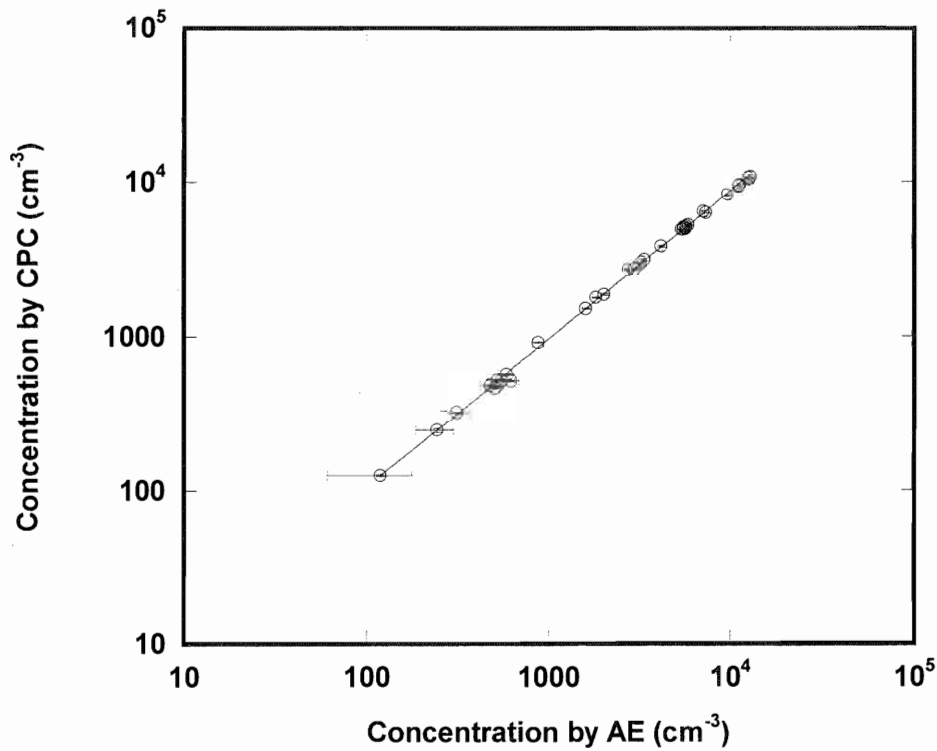
Figure 13. Plot of AE to CPC comparison for original uncorrected CPC data. The fit is per equation 5. The uncertainty bars represent the expanded uncertainty ( k=2 ) associated with AE calibration, flow rate and particle counting.
