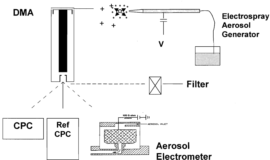
Figure 6. Schematic of test stand used to compare the test CPC and AE. A low sample volume reference CPC was operated through out the experiments and filter was collected for certain aerosol concentrations.
