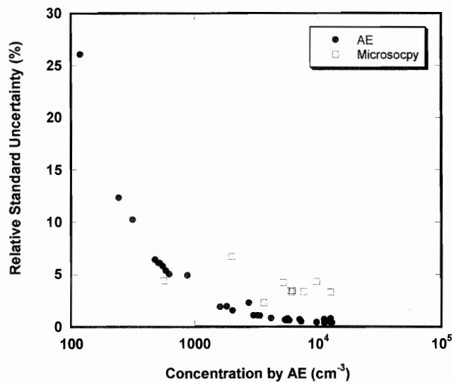
Figure 17. The total sum of the relative standard uncertainty ( k = 1 ) expressed as percent in the AE and microscopy measurements as a function of aerosol concentration.
