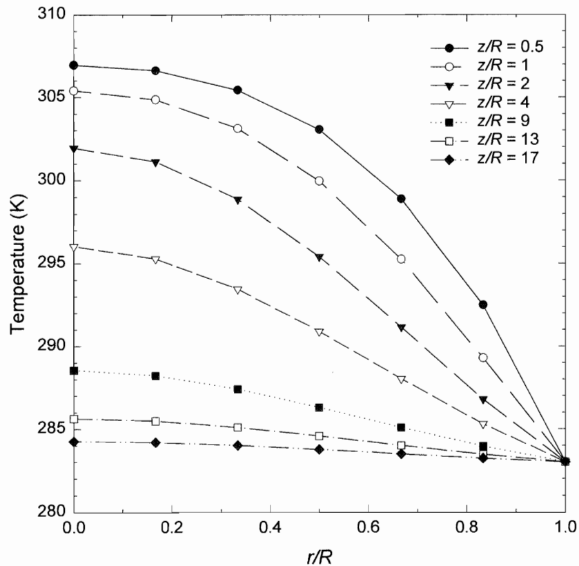
Figure A3. Steady-state temperature profiles in the condenser tube.
