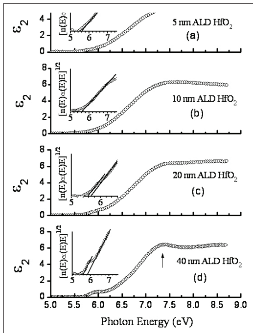
Figure 2. The imaginary part of the dielectric function, determined from VUV-SE data, for 5, 10, 20, 40 nm thick ALD \text{HfO}_2 films. All MOCVD \text{HfO}_2 spectra (not shown) are similar to that of the polycrystalline 40 nm ALD \text{HfO}_2 sample. All MOCVD \text{HfSiO} spectra (not shown) are similar to that of the amorphous 5 nm ALD \text{HfO}_2 sample.
