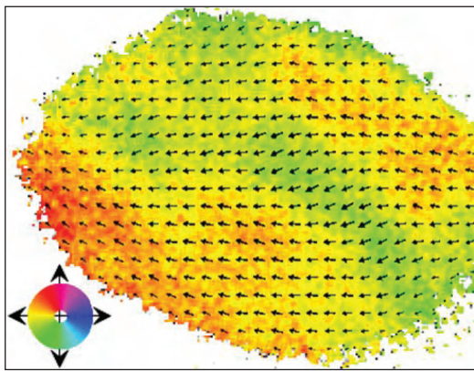
Figure 4. SEMPA image of an 0.5\ \mu\text{m} MRAM element. Although the element is nominally magnetized in one direction, variations of the magnetization direction within the element are seen both in the variations in color (related to magnetization direction by the colorwheel) and by the overlaid arrow field.
