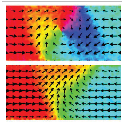
Figure 5. SEMPA images of current induced domain wall transitions in a 300\ \text{nm} wide ferromagnetic wire. The spin torque associated with the current moves the domain walls along the wires, but it also causes the walls to switch from vortex to transverse wall structures.
