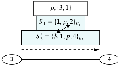
Figure 3: This figure sketches how S-BGP would stop an attempt by AS 3 to forge a route announcement. AS 1 had told AS 2 it would accept messages to p , and AS 2 told that to AS 3. However, AS 3 is trying to strip away 2 and fool AS 4 into believing a fraudulent 2-hop route. However, since AS 1 included the name of AS 2 in its signed statement about that link, AS 4 will detect the forgery.
