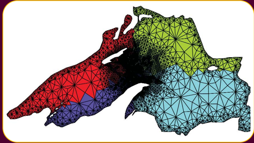
ITL's PHAML software for the parallel adaptive solution of partial differential equations has recently been extended to deal with complicated spatial domains. This image shows an adaptive grid computed by PHAML for Lake Superior.
