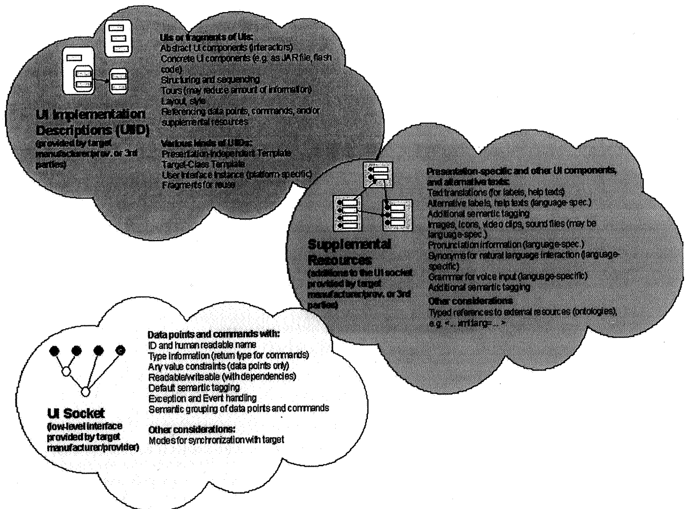
Figure 3: Early version of Overview of AIAP architecture.
