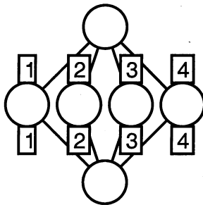
Figure 2: Nominal lattice
