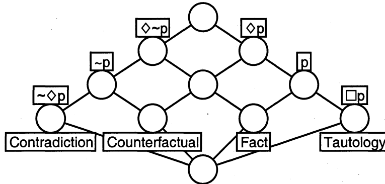
Figure 10: Concept lattice for modal logic
