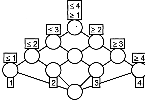
Figure 3: Interordinal lattice
