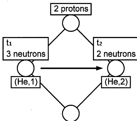
Figure 7: Concept lattice for {}^5\text{He} decay with life track
