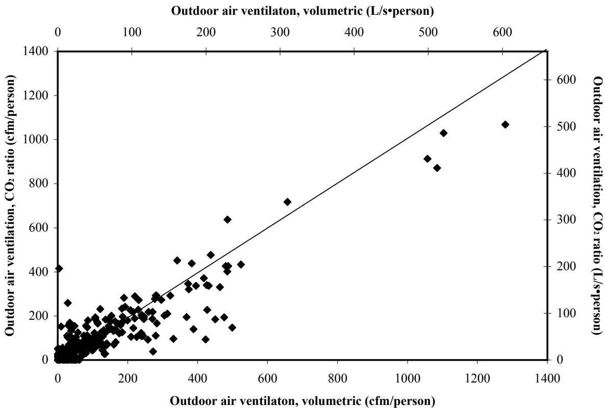
Figure 14 Outdoor air ventilation, CO 2 -ratio versus volumetric
