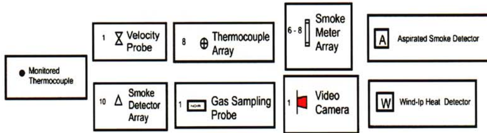
Figure 3. Instrument locations for smoke detector experiments.
