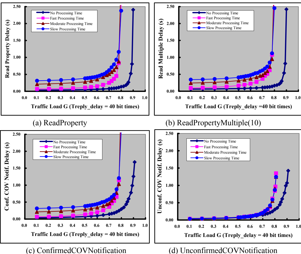
Figure 18. Average service delay of MS/TP with processing time ( T_{\text{reply\_delay}}=40 bit times).
