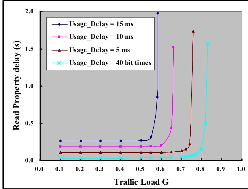
Figure 12. Effect of T_{usage\_delay} on average service delay.
