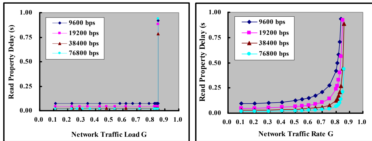
Figure 5. Average service delay for ReadProperty service requests (single-master).
