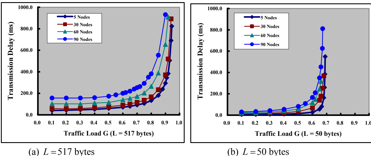
Figure 20. Transmission Delay in ARCNET Networks with a Change in the Number of Nodes
