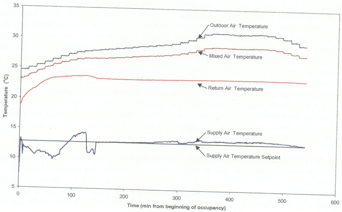
Figure 4.6 VCBT AHU-A Recirculation Damper Stuck Closed – Process Temperatures
